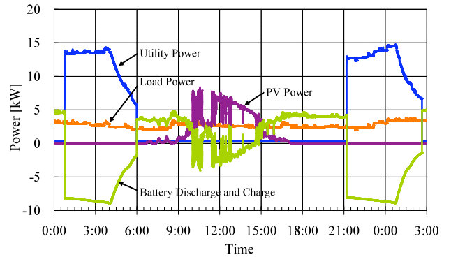
Fig. 8. A daily operating history
