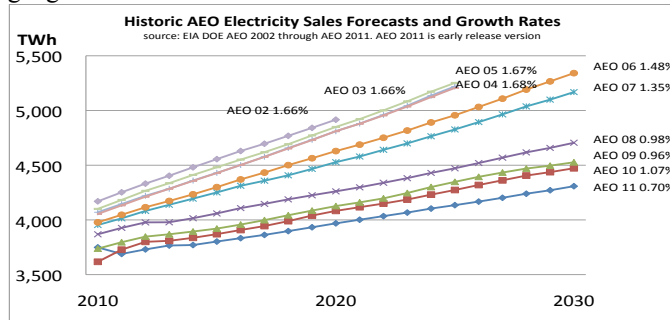
Fig. 1. U.S. Energy Information Administration forecasts of U.S. electricity consumption
