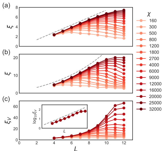
FIG. 2. Correlation length as a function of cylinder circumference L and bond dimension \chi , obtained from numerical iDMRG simulations. (a) On the O(5) line, with small stiffness: U = 2 , \bar{u} = u_3 = 1 , m = 0 . As \chi is increased, \xi approaches a linear dependence on size, \xi \sim \alpha L (dashed line), consistent with a CFT on the cylinder. (b) On the O(5) line, with large stiffness: U = 10 , \bar{u} = u_3 = 1 , m = 0 . \xi(L) is concave-up (dashed line is an exponential fit to the first 4 points at largest \chi ), consistent with a weakly-first-order transition. (c) On the VBS side: U = 2 , \bar{u} = 1 , u_3 = 0 , m = -0.1 . The correlation length in the valley channel \xi_v diverges exponentially with L (inset shows a semilogarithmic plot), clearly indicating a symmetry-broken state.
