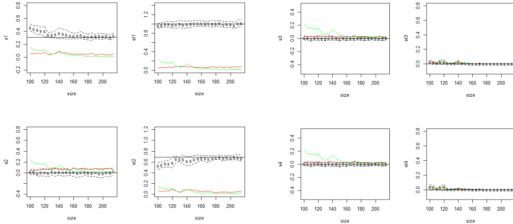
Figure 9: Graphs Showing Convergence of Sensitivities for Example 1 with Automatic Stopping: The x -axis is the training point size. The y -axis is the sensitivity. The sensitivities are S_1, S_{T1}, S_2, S_{T2}, S_3, S_{T3}, S_4, S_{T4} where the S_i are the first order sensitivities for variable i , S_{Ti} are the total sensitivities of variable i , the ‘S’s are the mean sensitivity estimates at each processing step converging to the horizontal straight black line which is the actual sensitivity, the irregular red (dark) lines are the standard deviations which stabilize as the training point size increases, the green (gray) lines are the emulator errors which decrease as the training point size increases, and the black dashed lines are the sensitivities plus and minus the standard deviation.
