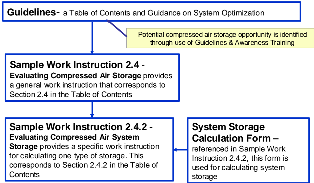
Figure 1: Organization of Industrial Systems Optimization Library
