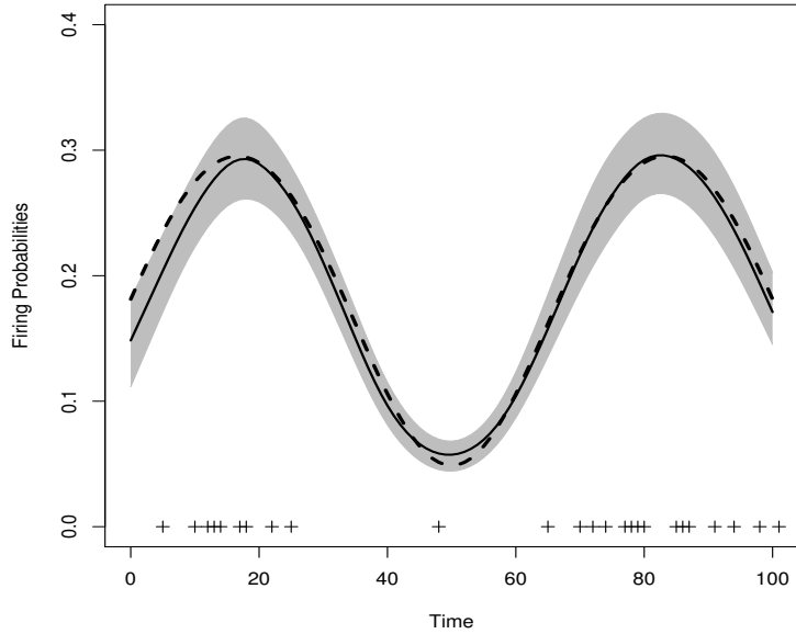
Figure 2.2: An illustrative example for using a Gaussian process model for a neuron with 40 trials. The dashed line shows the true firing rate, the solid line shows the posterior expectation of the firing rate, and the gray area shows the corresponding 95% probability interval. The plus signs on the horizontal axis represents spikes over 100 time intervals for one of the 40 trials.
