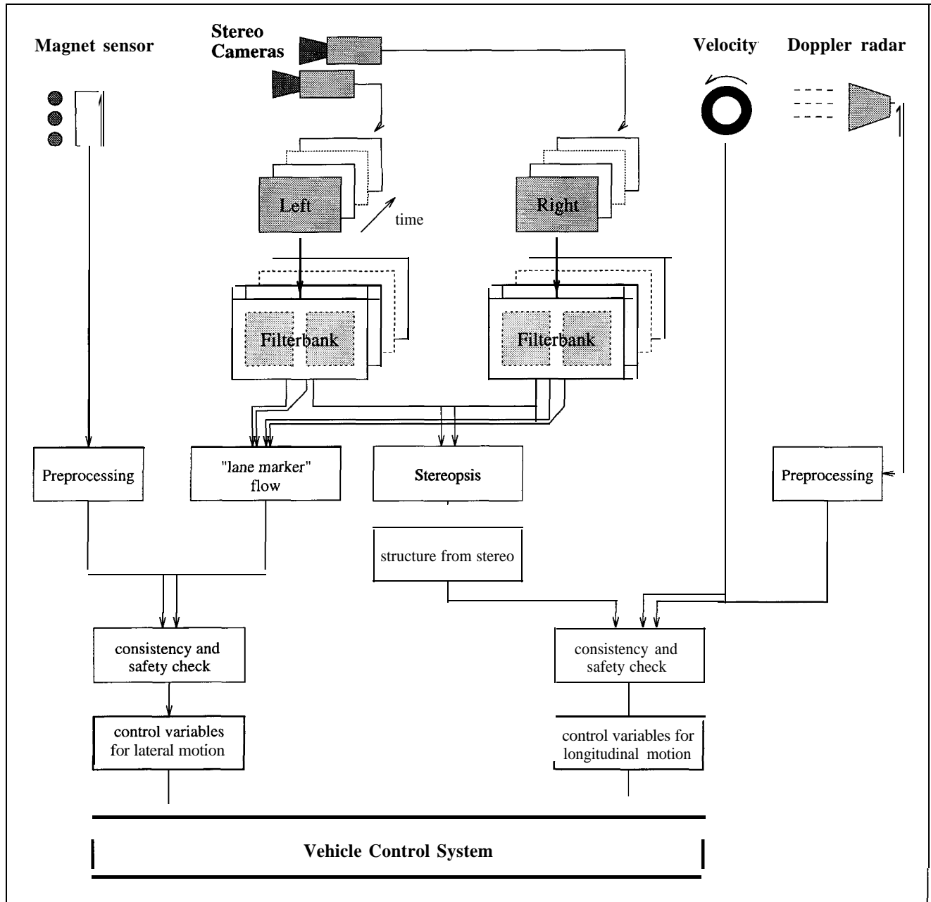
Figure 1: The flow chart of our proposed system for lane following.
