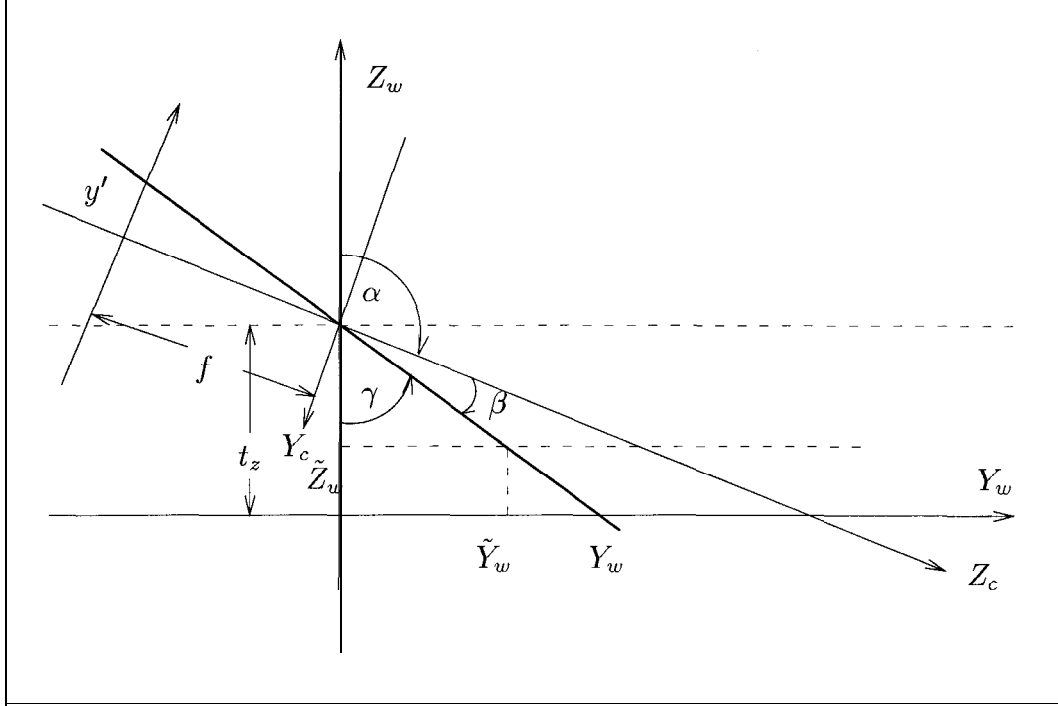
Figure 17: Both cameras are assumed to have an inclination angle \alpha . A point P = (X_w, Y_w, Z_w = 0)^T on the ground plane is projected onto the image plane at same location (x', y') as a point (\tilde{X}_w, \tilde{Y}_w, \tilde{Z}_w)^T .
