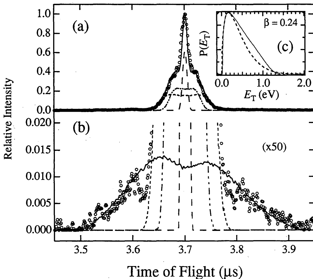
Figure 7: \text{CD}_2\text{CDO} TOF distribution for 3,140\text{ cm}^{-1} excess energy, showing individual fragment contributions. Experimental data ( \circ ), \text{CD}_2\text{CO} (— —), \text{CO} (— · — ·), \text{CD}_3 (· · ·). (a) sum of all contributions (—); (b) Magnification to show D atom contribution (—); (c) P(E_T) distribution (—) for this fit, with prior distribution also shown for comparison (· · ·).
