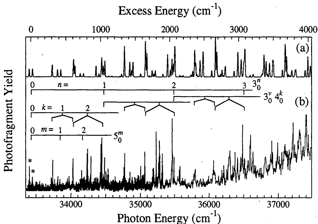
Figure 4: Vibrational structure in the first 4,000\text{ cm}^{-1} of the PFY spectrum. Excess energy is given relative to the rovibronic origin at 33,423.92\text{ cm}^{-1} . The vibrational progression in the \nu_3 CCO symmetric stretch and the two bending modes \nu_4 and \nu_5 are indicated by the combs, with the Renner-Teller splitting shown for \nu_4 .
