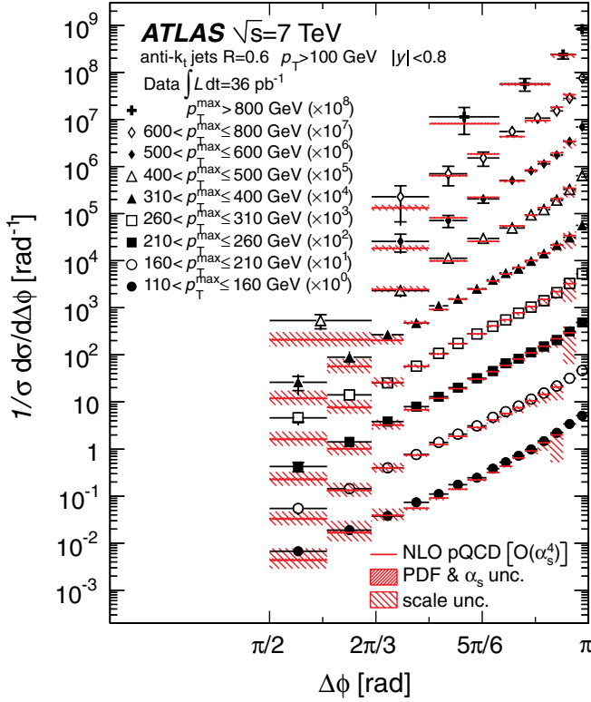
FIG. 2 (color online). The differential cross section (1/\sigma) \times (d\sigma/d\Delta\phi) binned in nine p_T^{\max} regions. Overlaid on the data (points) are results from the NLO pQCD calculation. The error bars on the data points indicate the statistical (inner error bar) and systematic uncertainties added in quadrature in this and subsequent figures. The theory uncertainties are indicated by the hatched regions. Different bins in p_T^{\max} are scaled by multiplicative factors of 10 for display purposes. The region near the divergence at \Delta\phi \rightarrow \pi is excluded from the calculation.
