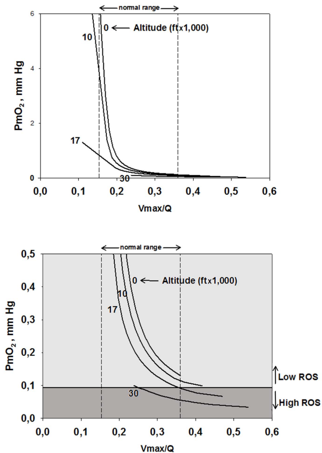
Figure 4. Mitochondrial P_{O_2} ( P_{mO_2} ) as a function of regional ratios of metabolic capacity ( \dot{V}_{max} ) to blood flow ( \dot{Q} ) at four altitudes. The lower \dot{Q} (supply) is in relation to \dot{V}_{max} (demand), the lower is P_{mO_2} at any altitude; also, P_{mO_2} at any \dot{V}_{max}/\dot{Q} ratio falls with increasing altitude. Vertical dashed lines mark the normal range of \dot{V}_{max}/\dot{Q} . Both panels show the same data, but the lower panel expands the y-axis in its lower range to show when ROS generation is high (i.e., when P_{mO_2} < 0.1 mm Hg). Below 17,000ft, ROS generation remains low, but above this altitude, regions of normal muscle with high \dot{V}_{max}/\dot{Q} ratio generate high ROS levels, until at the Everest summit, almost the entire muscle generates high ROS levels. doi:10.1371/journal.pone.0111068.g004
