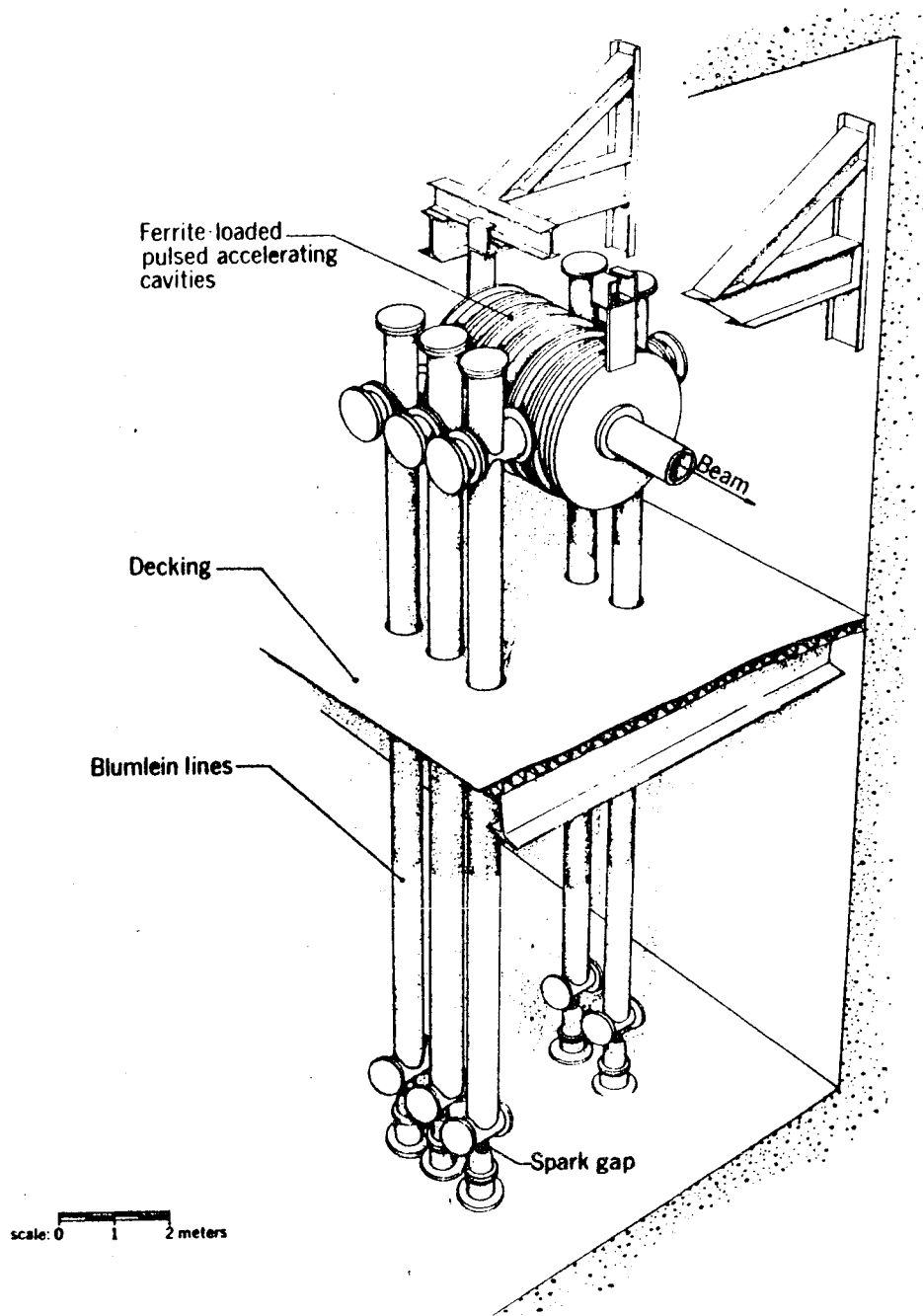
1.25 MeV Electron Induction-gun
