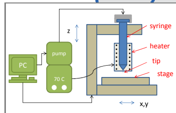
Image & schematic of Direct-Write Dispenser Printer
