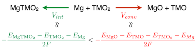
Figure 13. Schematic of competing intercalation and conversion reactions for a 2 electron transfer process with Mg. E_{\text{species}} is the internal energy of a species from DFT calculations and F the Faraday constant.
