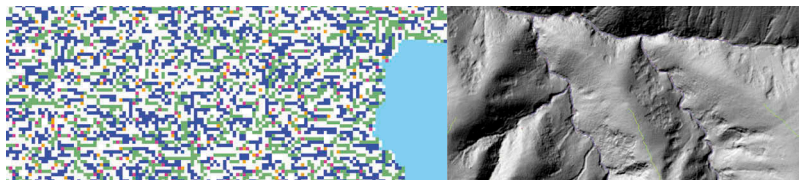
Figure 6. Computed surface network with critical points at two resolutions. Left: Swans Island Maine at 30 m (detail). Right: Part of Santa Cruz Island, California at 1 m (detail). Stream blue, ridge green, saddle orange, pit dark blue, summit pink.
