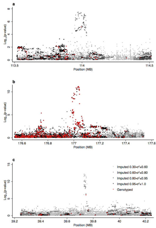
Figure 1. Manhattan plots showing association between risk of MOC and the genotypes of SNPs in a 1Mb region of re-imputation surrounding the most significantly associated SNP at (a) 2q13 (top SNP: rs752590), (b) 2q31.1 (top SNP: rs711830) and (c) 19q13.2 (top SNP: rs688187). Sample size is 1,644 cases and 21,693 controls. Red dots indicate a genotyped SNP in COGS, progressively darker grey dots indicate SNPs with pre-phased imputation r^2 values between 0.30 and 0.60, 0.60 and 0.80 and 0.80 to 0.95, respectively, and black dots indicate SNPs with pre-phased imputation r^2 values between 0.95 and 1.0.
