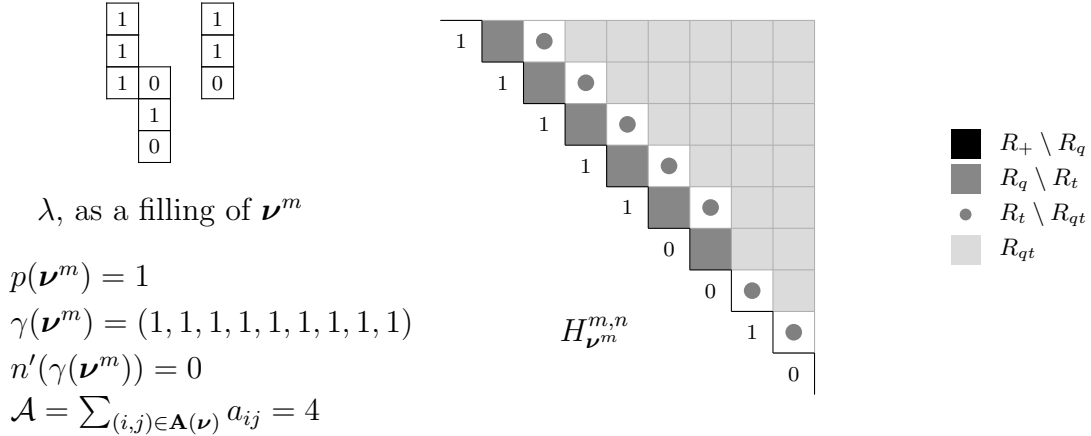
FIGURE 4. The LLT Catalanimal H_{\nu^m}^{m,n} for m = 3 , n = 2 , \nu = ((2), (1)) , \mathbf{o} = (-2, -2) , and its associated statistics. By Theorem 9.3.1, \psi_{\tilde{\Gamma}}(-q^5 t H_{\nu^m}^{m,n}) = \mathcal{G}_{\nu}[-MX^{m,n}] .
