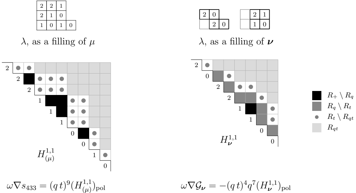
FIGURE 1. (i) The Catalanimal H_{(\mu)}^{1,1} for \mu = (433) . (ii) The Catalanimal H_{\nu}^{1,1} for \nu = ((32)/(1), (33)/(11)) . These are illustrated by drawing the root sets in an \ell \times \ell grid labeled by matrix-style coordinates, with the sets R_+ \setminus R_q , R_q \setminus R_t , R_t \setminus R_{qt} , R_{qt} specified according to the legend on the right; the weight \lambda is written on the diagonal with \lambda_1 in the upper left.
