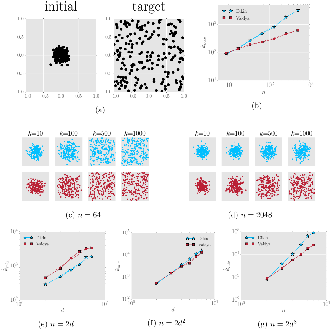
Figure 3. Comparison of the Dikin and Vaidya walks on the polytope \mathcal{K} = [-1, 1]^2 . (a) Samples from the initial distribution \mu_0 = \mathcal{N}(0, 0.04 \mathbb{I}_2) and the uniform distribution on [-1, 1]^2 . (b) Log-log plot of \hat{k}_{\text{mix}} (17) versus the number of constraints ( n ) for a fixed dimension d = 2 . (c, d) Empirical distribution of the samples for the Dikin walk (blue/top rows) and the Vaidya walk (red/bottom rows) for different values of n at iteration k = 10, 100, 500 and 1000 . (e, f, g) Log-log plot of \hat{k}_{\text{mix}} vs the dimension d , for n \in \{2d, 2d^2, 2d^3\} for d \in \{2, 3, 4, 5, 6, 7\} . The exponents from these plots are summarized in Table 2. Note that increasing the number of constraints n has more profound effect on the Dikin walk in almost all the cases.
