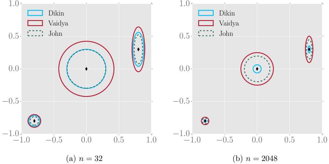
Figure 2. Visualization of the proposal distribution on the square with repeated constraints \mathcal{S}_{n/4} for the different random walks. (a, b) Unit ellipsoids associated with the covariances of the random walks at different states x on the square with repeated constraints \mathcal{S}_{n/4} . Clearly, all these ellipsoids adapt to the boundary but increasing n has a profound impact on the volume of the Dikin ellipsoids and comparatively less impact on the Vaidya and John ellipsoids.
