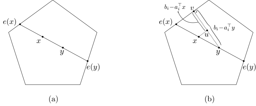
Figure 6. Polytope \mathcal{K} = \{x \in \mathbb{R}^d | Ax \leq b\} . (a) The points e(x) and e(y) denote the intersection points of the chord joining x and y with \mathcal{K} such that e(x), x, y, e(y) are in order. (b) A geometric illustration of the argument (23). It is straightforward to observe that \|x - y\|_2 / \|e(x) - x\|_2 = \|u - y\|_2 / \|u - v\|_2 = |a_i^\top (y - x)| / (b_i - a_i^\top x) .
