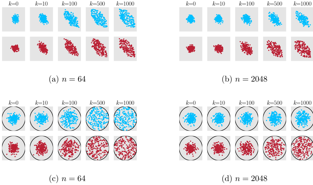
Figure 4. Empirical distribution of the samples from 200 runs for the Dikin walk (blue/top rows) and the Vaidya walk (red/bottom rows) at different iterations k . The 2-dimensional polytopes considered are: (a, b) random polytopes with n -constraints, and (c, d) regular n -polygons inscribed in the unit circle. For both sets of cases, we observe that higher n slows down the walks, with visibly more effect on the Dikin walk compared to the Vaidya walk.
