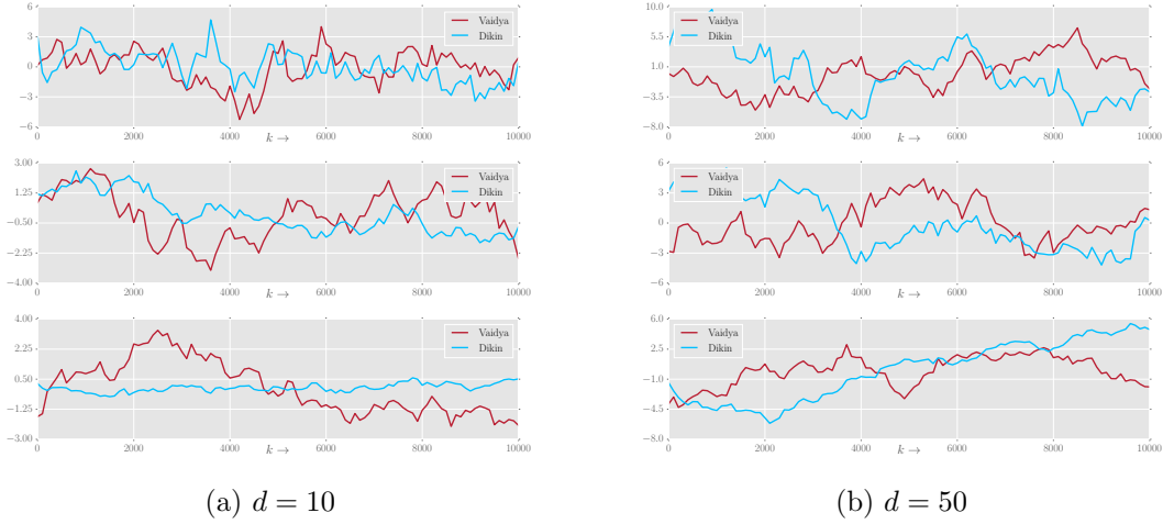
Figure 5. Sequential plots of a one-dimensional random projection of the samples on the hyperbox \mathcal{K} = [-1, 1]^d , defined by n constraints. Each plot corresponds to one long run of the Dikin and Vaidya walks, and the projection is taken in a direction chosen randomly from the sphere. (a) Plots for d = 10 and n \in \{20, 640, 5120\} . (b) Plots for d = 50 and n \in \{100, 400, 1600\} . Relative to the Dikin walk, the Vaidya walk has a more jagged plot for pairs (n, d) in which the ratio n/d is relatively large: for instance, see the plots corresponding to (n, d) = (640, 10) and (5120, 10) . The same claim cannot be made for pairs (n, d) for which the ratio n/d is relatively small; e.g., the plot with (n, d) = (20, 10) . These observations are consistent with our results that the Vaidya walk mixes more quickly by a factor of order \mathcal{O}(\sqrt{n/d}) over the Dikin walk.
