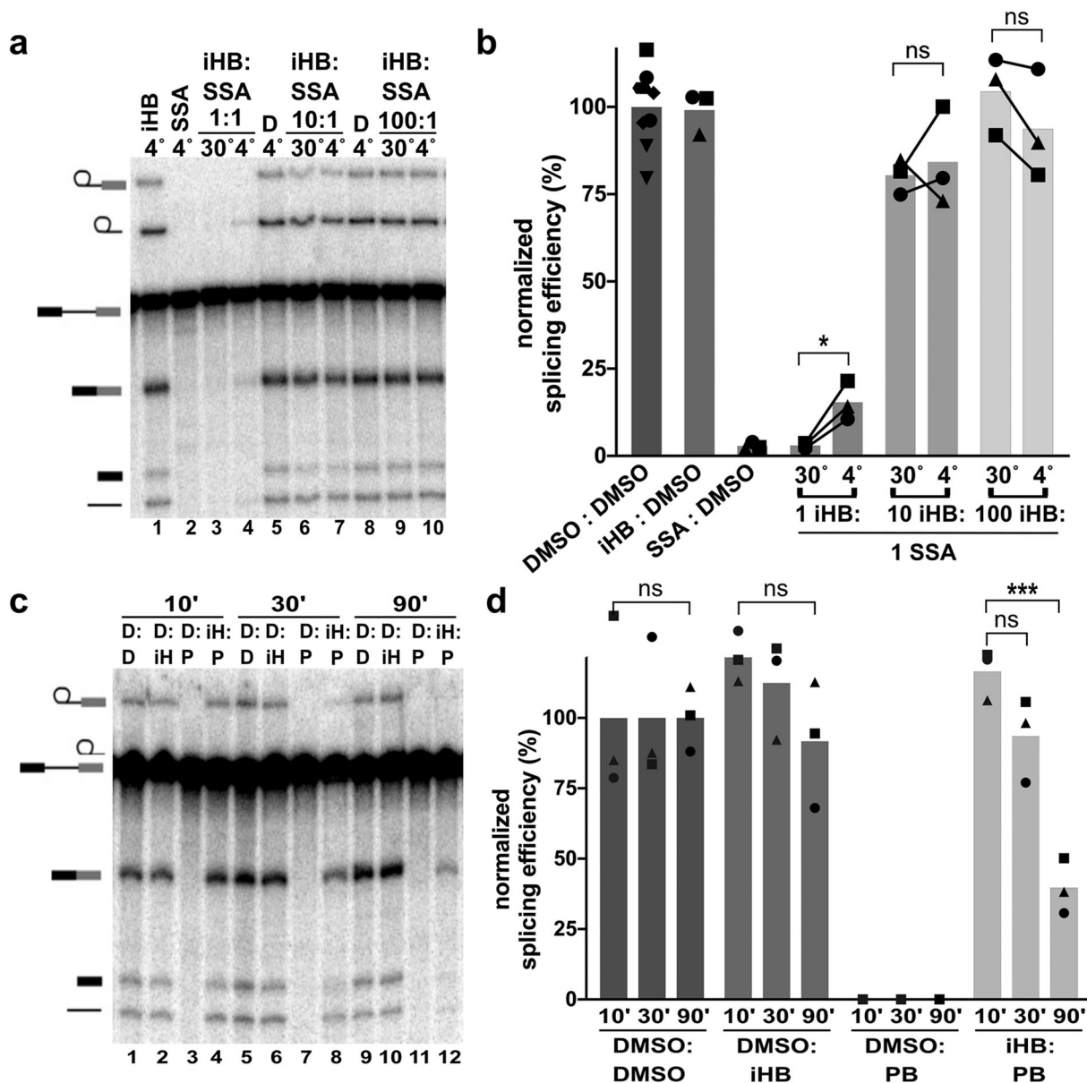
Figure 4. SF3B inhibitors exchange more slowly than inactive analogs. (a) Representative denaturing gel as described in Figure 1. Binding and competitions phases were 10 minutes with 1, 10 or 100 μM iHB and 1 μM SSA. (b) Splicing efficiency quantified from denaturing gels as described in Figure 1. (c) Representative denaturing gel with 10 minute binding phase and varying length competitions phases at 30°C. D= DMSO, iH = iHB, P=PB. (d) Splicing efficiency quantified for (c).
