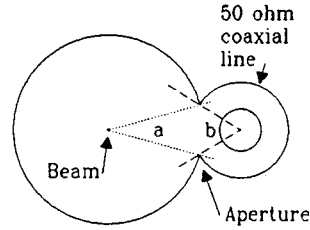
Fig. 3. Aperture Coupling
