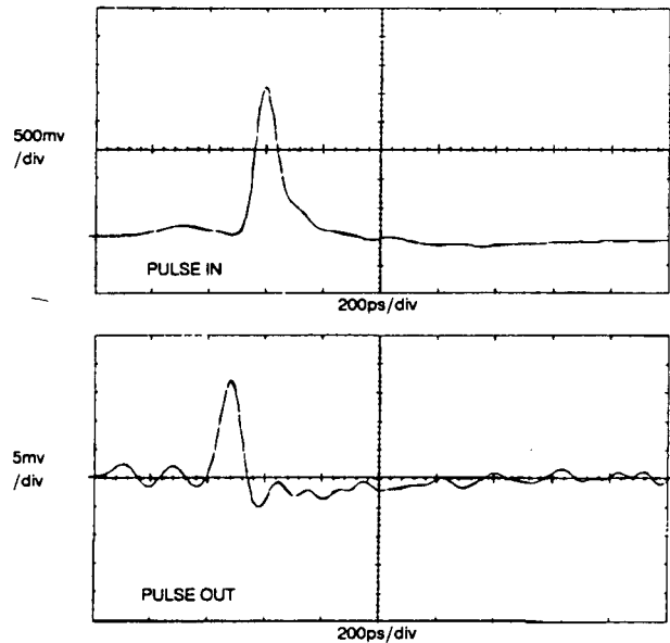
Fig. 6 Slot-Coupled Pickup Pulse Response
