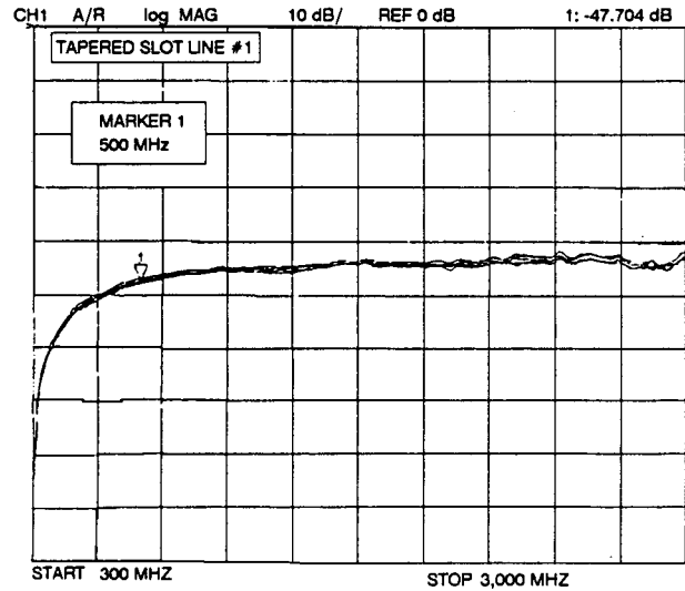
Fig. 5 Slot-Coupled Pickup Frequency Response
