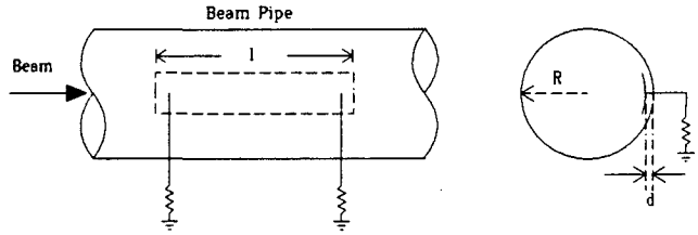
Fig. 1 Typical Stripline
