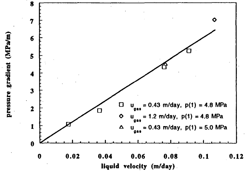
Figure 2: Experimental (symbols) and model (solid line) steady-state pressure gradient versus liquid velocity at fixed gas injection rate.
