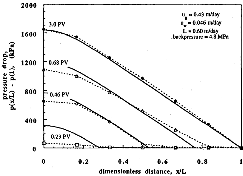
Figure 5: Experimental (symbols connected by dashed lines) and model (solid lines) transient pressure profiles for simultaneous injection of gas and foamer solution at fixed mass rates. Porous medium is presaturated with surfactant solution.
