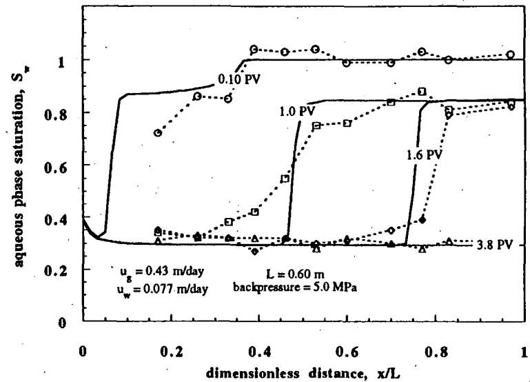
Figure 10: Experimental (symbols connected by dashed lines) and model (solid lines) transient aqueous-phase saturation profiles. Gas and foamer solution are simultaneously injected at fixed mass rates. Porous medium is initially free of surfactant.
