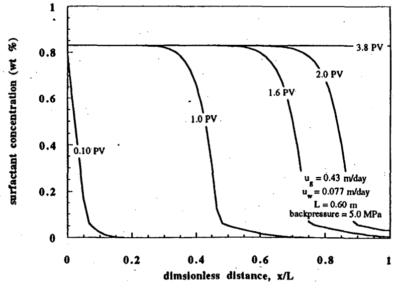
Figure 12: Model transient surfactant concentration. Gas and foamer solution are simultaneously injected at fixed mass rates.
