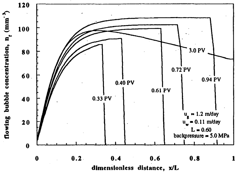
Figure 9: Model transient flowing-foam textures for a porous medium presaturated with surfactant. Gas and foamer solution are simultaneously injected at fixed mass rates.
