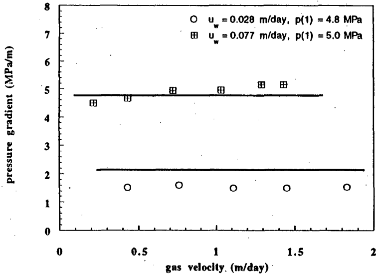
Figure 3: Experimental (symbols) and model (solid line) steady-state pressure gradient versus gas velocity at fixed liquid injection rate.
