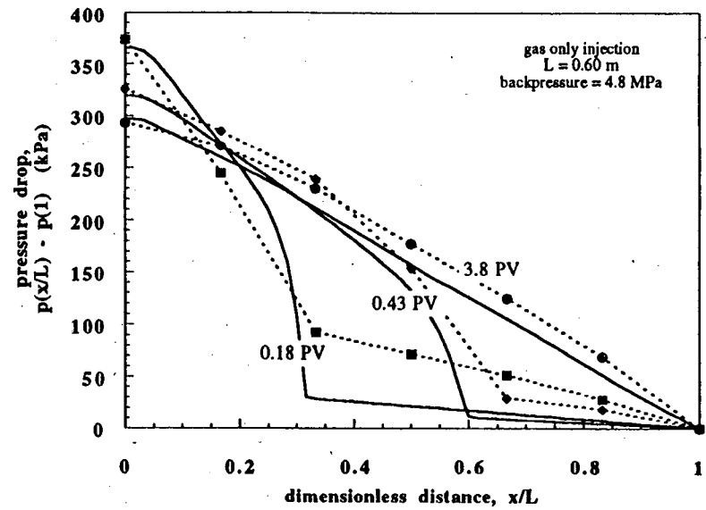
Figure 14: Experimental (symbols connected by dashed lines) and model (solid lines) transient pressure profiles. Gas is injected at fixed pressure at core inlet. Porous medium is initially saturated with surfactant.
