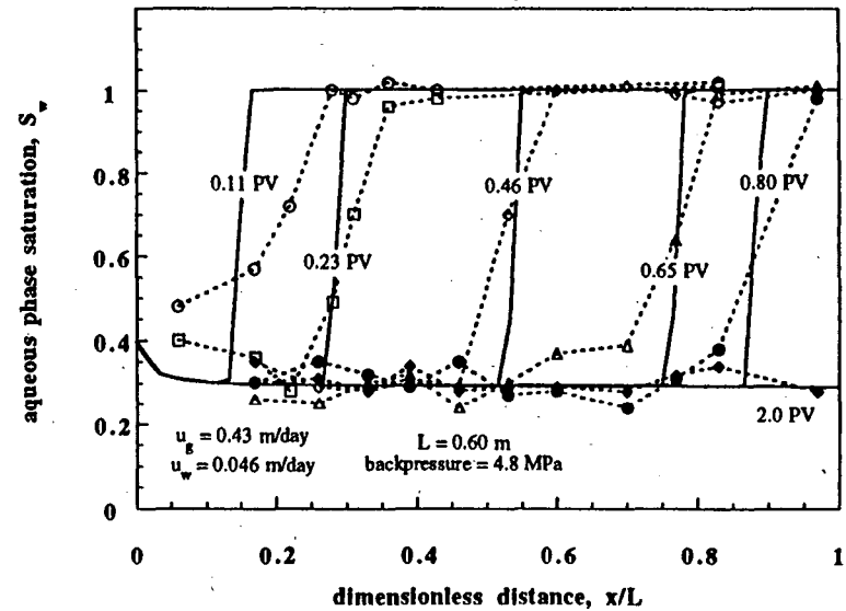
Figure 4: Experimental (symbols connected by dashed lines) and model (solid lines) transient aqueous-phase saturation profiles for simultaneous injection of gas and foamer solution at fixed mass rates. Porous medium is presaturated with surfactant solution.
