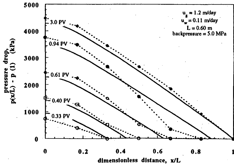
Figure 8: Experimental (symbols connected by dashed lines) and model (solid lines) transient pressure profiles. Porous medium is presaturated with surfactant solution. Gas and foamer solution are simultaneously injected at fixed mass rates.
