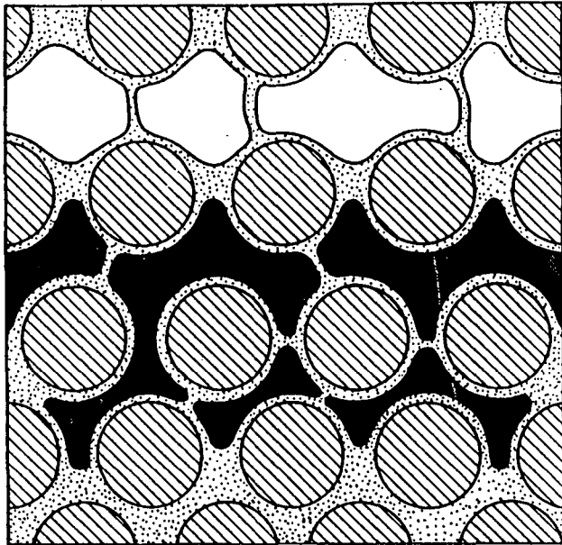
Figure 1: Pore-level schematic for a flowing foam. Flowing bubbles are unshaded and trapped gas is darkly shaded.
