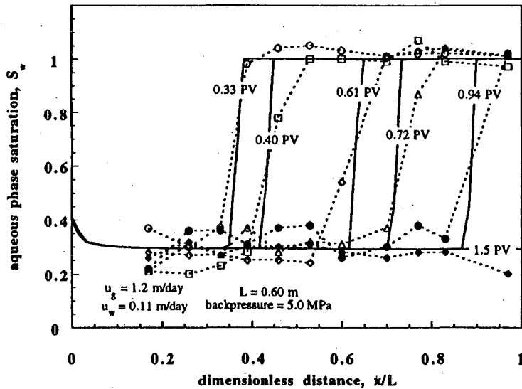
Figure 7: Experimental (symbols connected by dashed lines) and model (solid lines) transient aqueous-phase saturation profiles. Porous medium is presaturated with surfactant solution. Gas and foamer solution are simultaneously injected at fixed mass rates.
