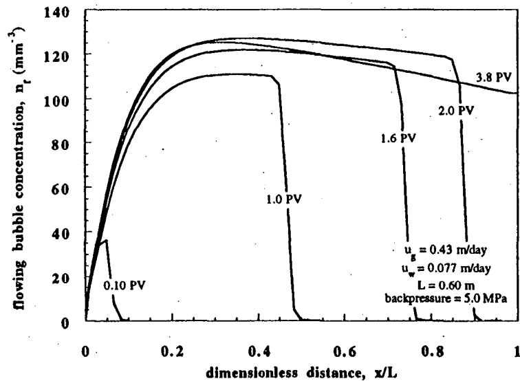
Figure 11: Model transient flowing-foam textures for a porous medium initially free of surfactant. Gas and foamer solution are simultaneously injected at fixed mass rates.
