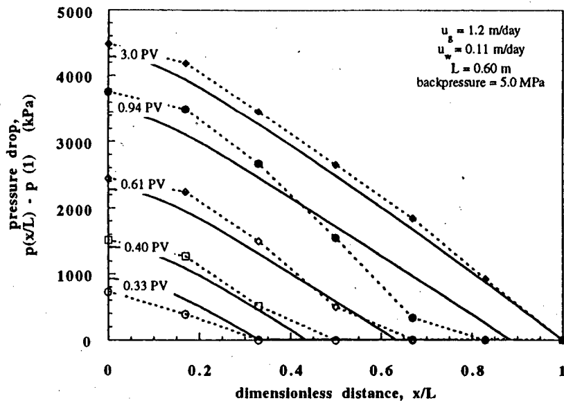
Figure 13: Experimental (symbols connected by dashed lines) and model (solid lines) transient pressure profiles. Gas and foamer solution are simultaneously injected at fixed mass rates. Porous medium is initially free of surfactant.
