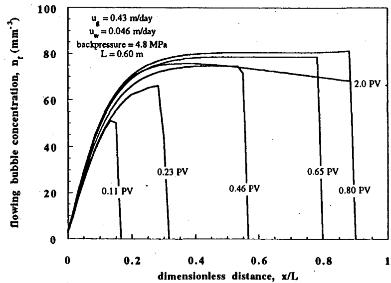
Figure 6: Model transient flowing-foam textures for a porous medium presaturated with surfactant. Gas and foamer solution are simultaneously injected at fixed mass rates.
