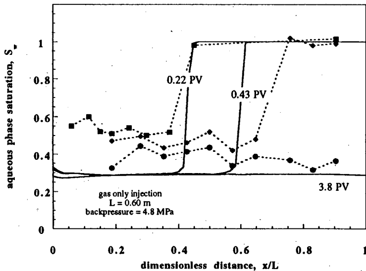
Figure 15: Experimental (symbols connected by dashed lines) and model (solid lines) transient aqueous-phase saturation profiles. Gas is injected at fixed pressure at core inlet. Porous medium is initially saturated with surfactant.
