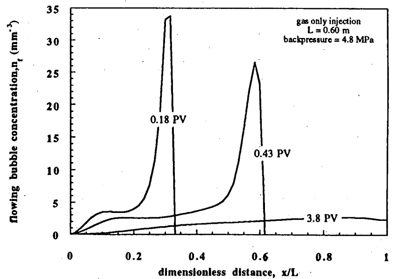
Figure 16: Model transient flowing-foam textures. Gas is injected at fixed pressure at core inlet. Porous medium is initially saturated with surfactant.
