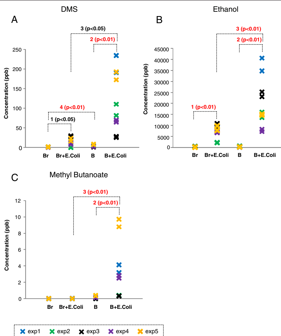
Figure 1 Representative patterns of VOCs in Category 1. (A) DMS, (B) Ethanol, and (C) Methyl Butanoate emission from 4 different conditions: broth only (Br), E. coli in LB broth (Br + E. coli ), whole blood only (B), and E. coli -inoculated whole blood (B + E. coli ). 1. significantly different between Broth only and Broth + E. coli ; 2. significantly different between Blood only and Blood + E. coli ; 3. significantly different between Broth + E. coli and Blood + E. coli ; 4. significantly different between Broth only and blood only.
