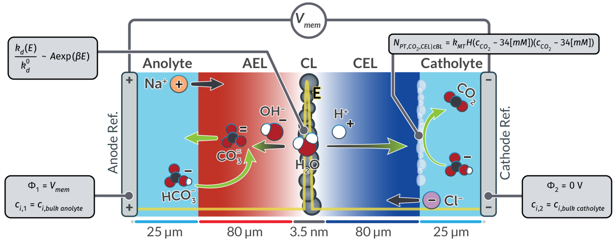
Figure 2: Schematic of simulated domain for BPM performing BPM-ED EMCC. \text{H}_2\text{O} at the interface of the AEL and CEL (in the CL) is reacted by electric-field-enhanced water dissociation to form \text{H}^+ and \text{OH}^- . The \text{H}^+ reacts with \text{HCO}_3^- in the catholyte to form \text{CO}_2 . Once the in situ generated \text{CO}_2 has exceeded its solubility limit in the catholyte, it exits the aqueous phase in the form of bubbles. \text{OH}^- from water dissociation reacts with \text{HCO}_3^- absorbed in the AEL to form \text{CO}_3^{2-} that transports back into the anolyte. Spectator co-ions from the anolyte or catholyte can cross through the membrane to reduce the developed pH gradient.
