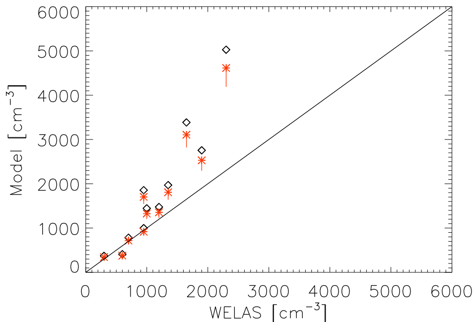
Figure 6. The number of cloud droplets formed in the model (orange stars) and the number of aerosols immediately before the expansion (black diamonds), plotted against the maximum number of droplets detected by WELAS during the presence of the cloud. The error bars on the modelled droplet numbers correspond to simulations using the high and low values of the dew point calculated from the SIMONE data. Data are shown for all CLOUD9 experiments where data were available.
