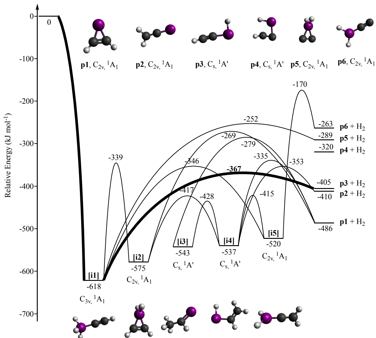
Fig. 3. Potential energy surfaces (PESs) in \text{kJ mol}^{-1} for the reactions of singlet dicarbon with silane along with electronic ground state symmetries and point groups of intermediates and products. The lowest energy pathway from reactants to products is bolded. Atoms are color coded in white (hydrogen), purple (silicon), and black (carbon). Structures along with the vibrational frequencies of the reactants, intermediates, products, and transition states are compiled in the Supplementary Material (Table S2).
