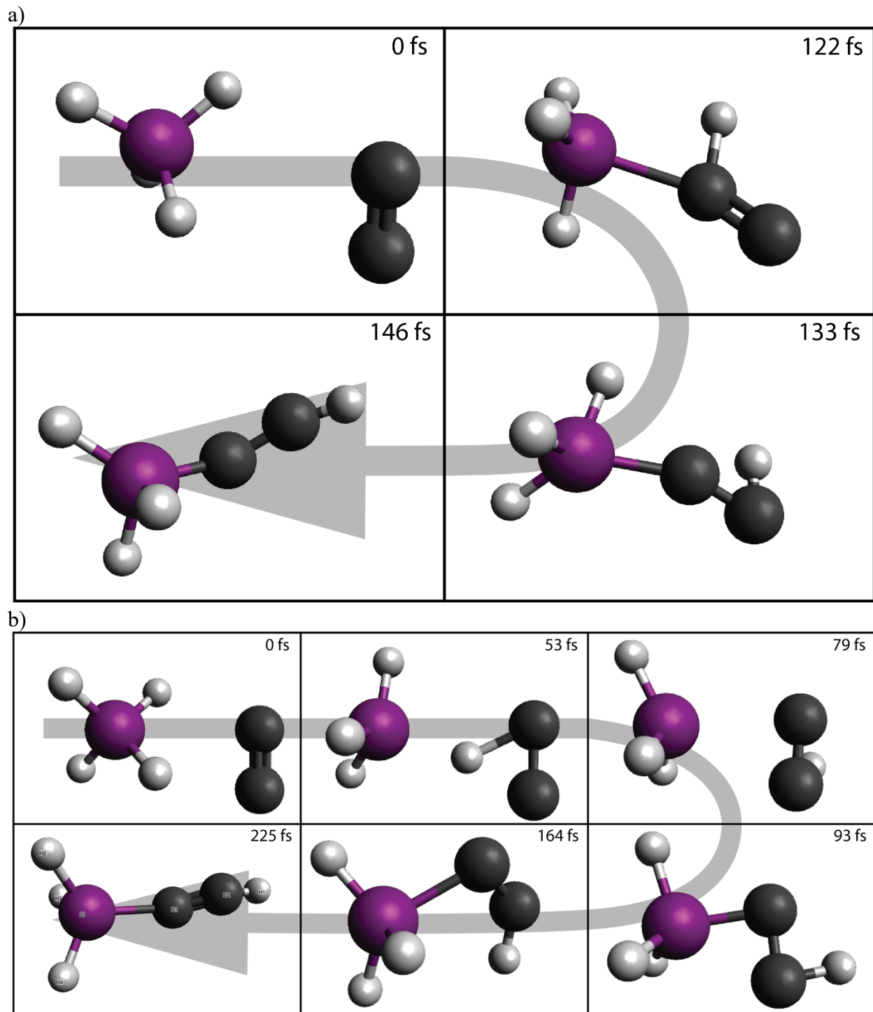
Fig. 4. Snapshots along the reaction coordinate for a) an initial barrierless 1,1-insertion of singlet dicarbon into a silicon – hydrogen bond of silane followed by hydrogen migration leading to the 3-sila-methylacetylene (HCCSiH 3 ) intermediate [i1] and b) a hydrogen abstraction leading to the ethynyl and silyl radical pair followed by radical-radical recombination to 3-sila-methylacetylene (HCCSiH 3 ) intermediate [i1].
