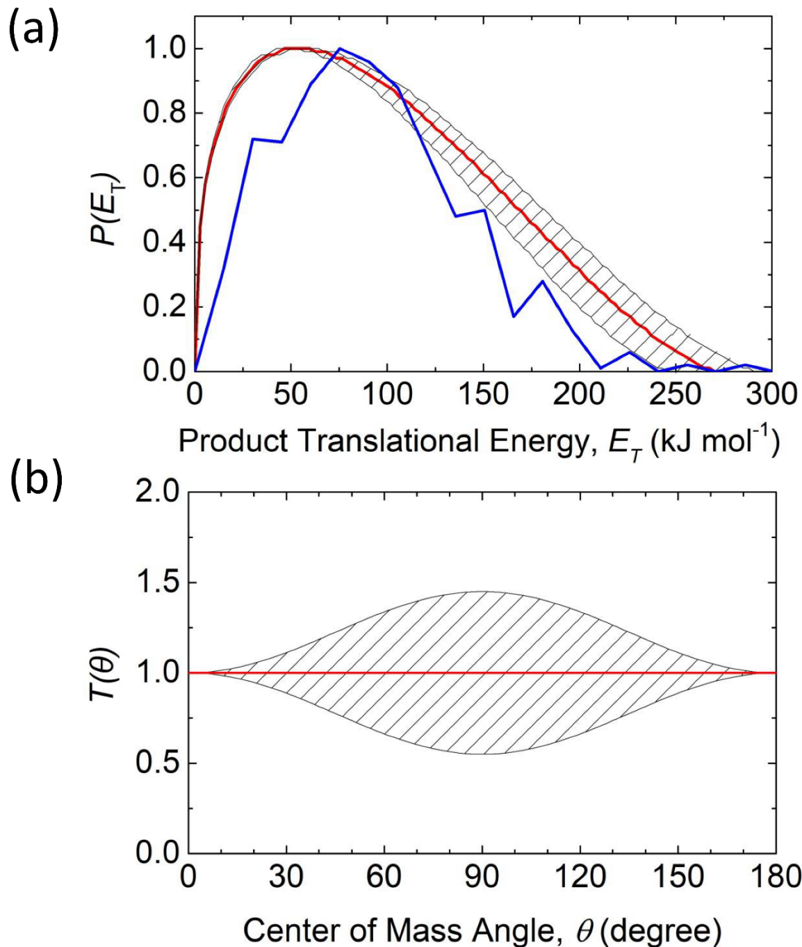
Figure 2: Center-of-mass translational energy (a) and angular (b) flux distributions for the formation of C_2SiH_2 isomers plus molecular hydrogen via the reaction of dicarbon ( C_2; X^1\Sigma_g^+/a^3\Pi_u ) with silane ( SiH_4; X^1A_1 ). The hatched areas define regions of acceptable fits. In (a), QCT calculations provide the center-of-mass translational energy distribution color coded in blue.
