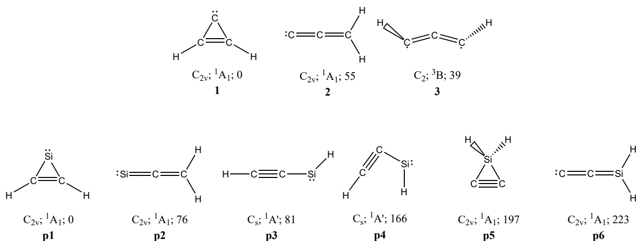
Scheme 1. Molecular structures, electronic ground state wave functions, point groups, and the relative energies of \text{C}_3\text{H}_2 ( 1-3 ) and \text{SiC}_2\text{H}_2 ( p1-p6 ) isomers. Energies are shown in \text{kJ mol}^{-1} .
