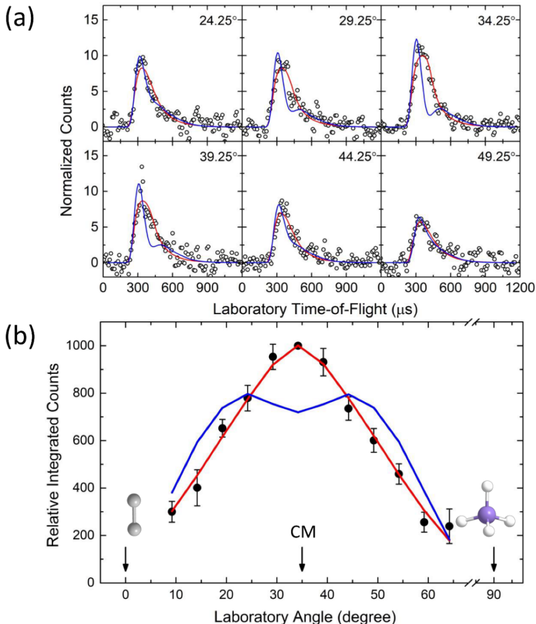
Figure 1. (a) Time-of-flight (TOF) spectra recorded at m/z = 54 ( \text{C}_2\text{SiH}_2^+ ) for reaction of dicarbon ( \text{C}_2 ; X^1\Sigma_g^+ / a^3\Pi_u ) with silane ( \text{SiH}_4 ; X^1A_1 ). The open circles are experimental data; the fits in blue and red result from the quasiclassical theory (QCT)-based and ‘best fit’ center-of-mass translational energy distributions respectively. (b) Laboratory angular distribution obtained at m/z = 54 ( \text{C}_2\text{SiH}_2^+ ) from the reaction of dicarbon ( \text{C}_2 ; X^1\Sigma_g^+ / a^3\Pi_u ) with silane ( \text{SiH}_4 ; X^1A_1 ). The circles are experimental data; the fits in blue and red result from the QCT-based and ‘best fit’ center-of-mass translational energy distributions respectively.
