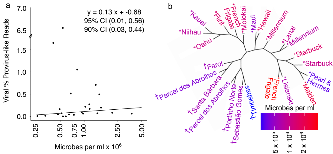
Extended Data Figure 2.4: Temperateness of viral communities increases with host density and viral functional composition change.
