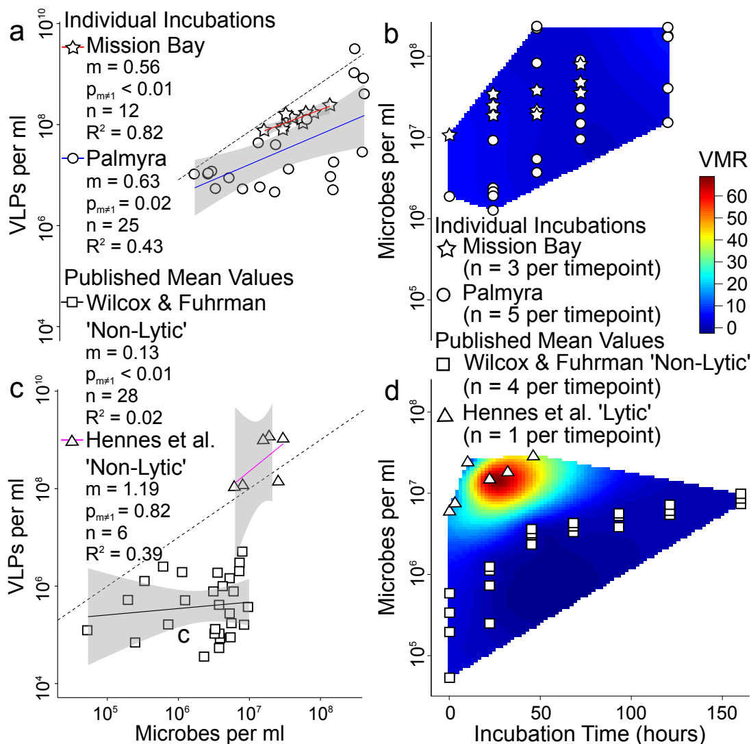
Figure 2.3: Density dependence does not drive viral predation.
