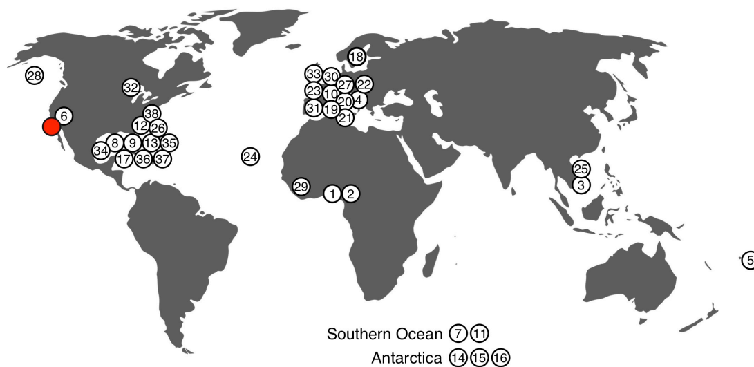
Figure 3.1: Schematic map of locations of the thirty-eight published chemically induced lysogen studies subjected to meta-analysis.
