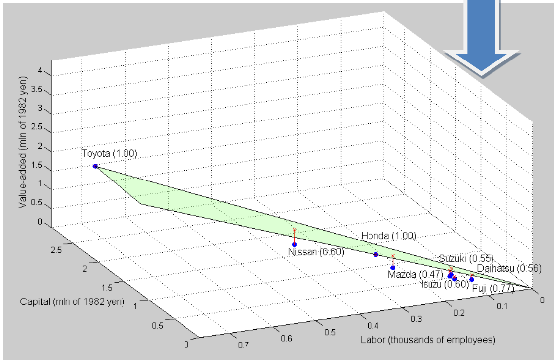
Figure 2 Three-dimensional efficient frontier (year 1997)
