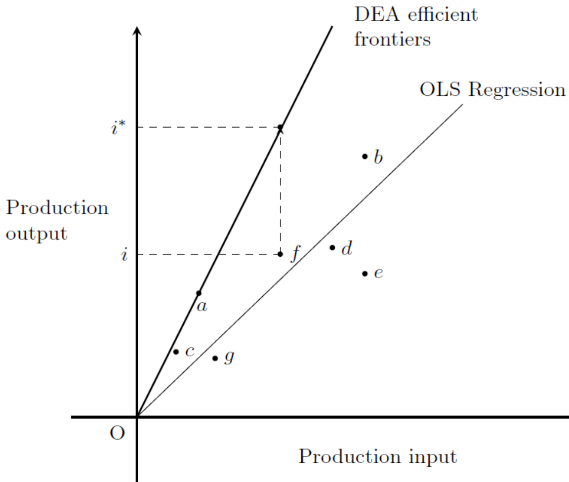
Figure 1(a) Illustration of the DEA frontier
