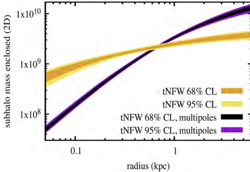
Figure 2.3: Projected mass profiles for the tNFW and tNFWmult models. While the mass profiles differ substantially, near the perturbation radius at around 1 kpc, the projected masses converge to a similar value. [92]
