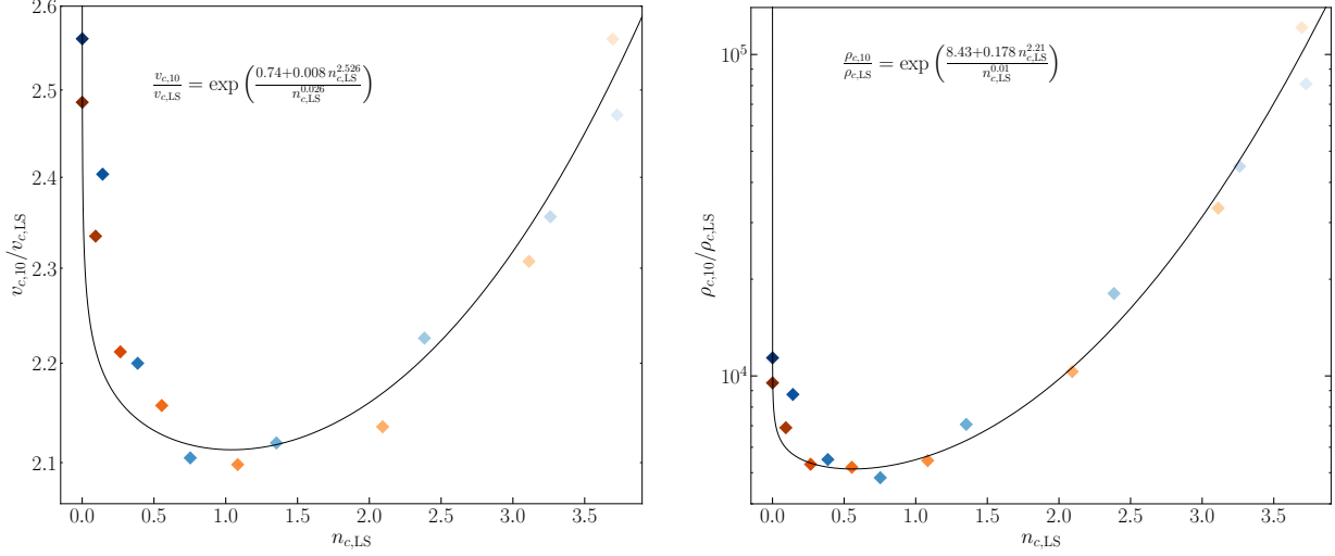
Figure 5.6: (Left) The v_{c,10}/v_{c,LS} to n_{c,LS} relation plotted as a black curve, fitted to our numerical results (diamonds). (Right) Same as the left, but for the \rho_{c,10}/\rho_{c,LS} to n_{c,LS} relation.
