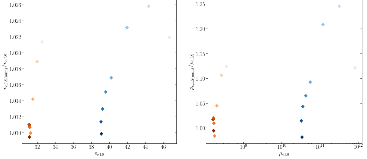
Figure 5.9: ( Left ) Comparison between the numerically obtained and analytically predicted central velocity at LS transition, plotted as a function of the analytic central velocity at the LS transition. The difference between them is very small, within \sim 2.6\% . ( Right ) Comparison between the numerically obtained and analytically predicted central density at LS transition, plotted as a function of the LS transition central density. Here the analytic and numerical values differ by at most \sim 25\% . It is unsurprising that the central density is a bit less accurate as it is the parameter that changes drastically.
