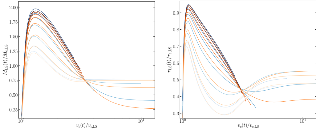
Figure 5.10: ( Left ) The LS transition mass normalized by the core mass at LS transition as a function of central velocity. ( Right ) The LS transition radius normalized by the core radius at LS transition as a function of central velocity.
