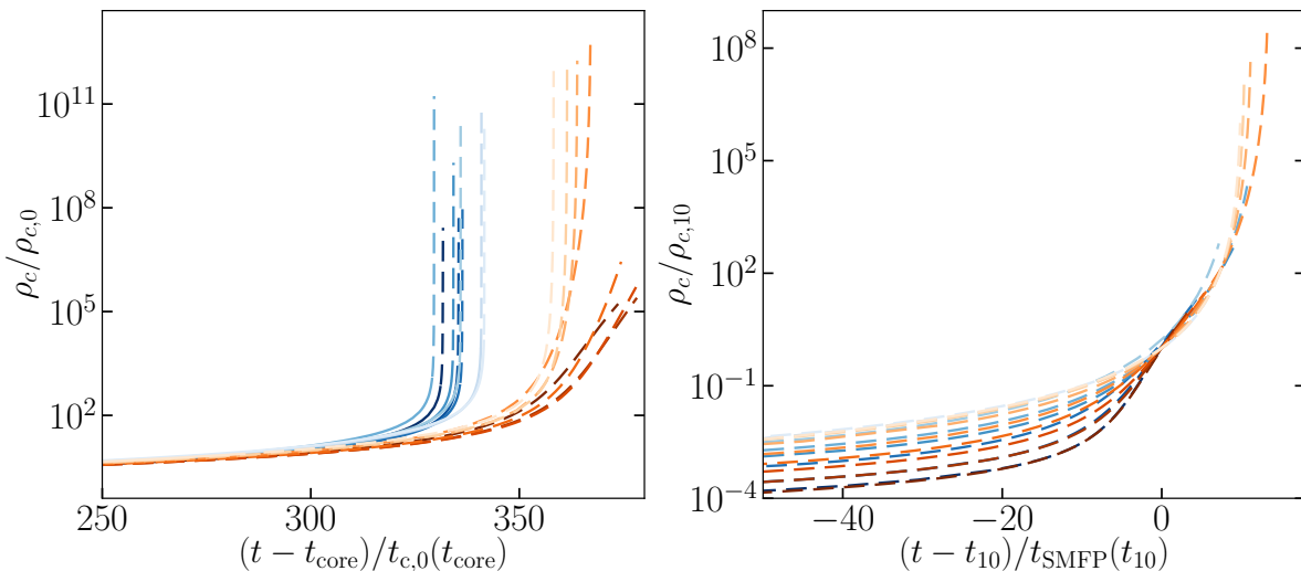
Figure 5.3: ( Left ) The evolution of the central density as a function of time, shifted and normalized to the time maximal core is reached as defined in O23. One can see that for different \sigma_{c,0} , the collapse times differ. ( Right ) Same as the left plot, except the time here is shifted and normalized to the time the halos enter the \gamma = 10 phase, where the curves line up relatively well as we are already in the self-similar solution. Note that here, the time the curves enter the \gamma = 10 phase is not analytically determined, thus resulting in the scatter.
