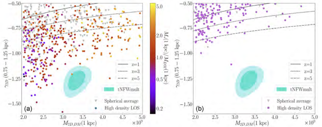
Figure 2.5: Slope of the surface density profile versus projected mass in 1 kpc. Here, we limit the sample to the range M(1 \text{ kpc}) = 2 - 5 \times 10^9 M_\odot and \gamma_{2D} \leq -0.5 for both the hydrodynamical (panel (a)) and DMO (panel (b)) runs. Color conventions for markers are the same as in Fig. 2.4. Both panels include the 68% and 95% contours from lensing constraints for the tNFWmult model. Included is the cosmological relation for dark matter for z = 1, 3, 5 at 3\sigma .
