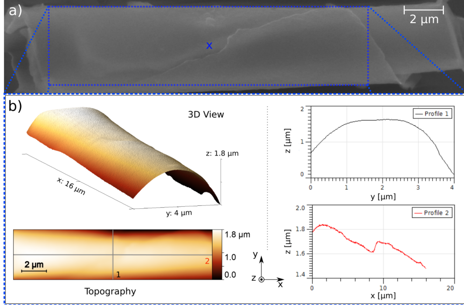
Figure 2: a) SEM image of a Co/Pd microtube with two windings: Blue drawn box with center point (x) shows the range of the MFM scan, representing an area of 16 \mu\text{m} \times 4 \mu\text{m} . b) MFM topographic channel, recorded in zero-field from top left to bottom right at a tip-surface distance of (205 \pm 10) \text{ nm} , with the latter measured above the center point. In this experiment, A_2 = 0.22 \text{ nm} , if \hat{U}_{AC} = 1.0 \text{ V} is applied between MFM tip and sample. Shown are 3D and top view topographic images with two line profiles across the tube circumference (profile 1) and along the tube axis (profile 2). Profile 2: A step in the tube topography is visible which originates from the edge of the outer winding that is wrapped around the inner winding with a spacing of approximately 100 \text{ nm} .
