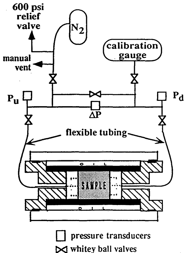
Figure 1. Gas-pressure-pulse-decay apparatus.
