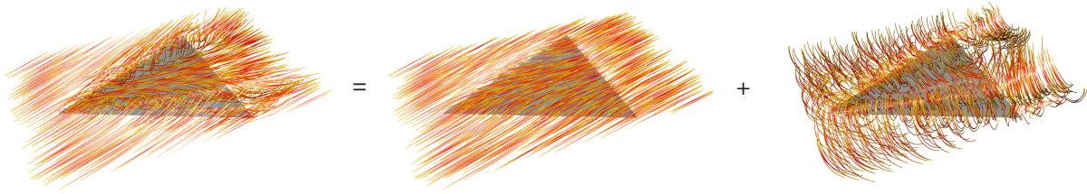
Figure 1: Illustration of the different components of the flow around the delta wing. Left: Original flow field from the CFD simulation, Middle: Laplacian field computed by the original field's flow normal to the boundary. Note that the flow is simple but not constant. Right: Localized or region-specific flow obtained by subtracting the Laplacian field from the original field.
