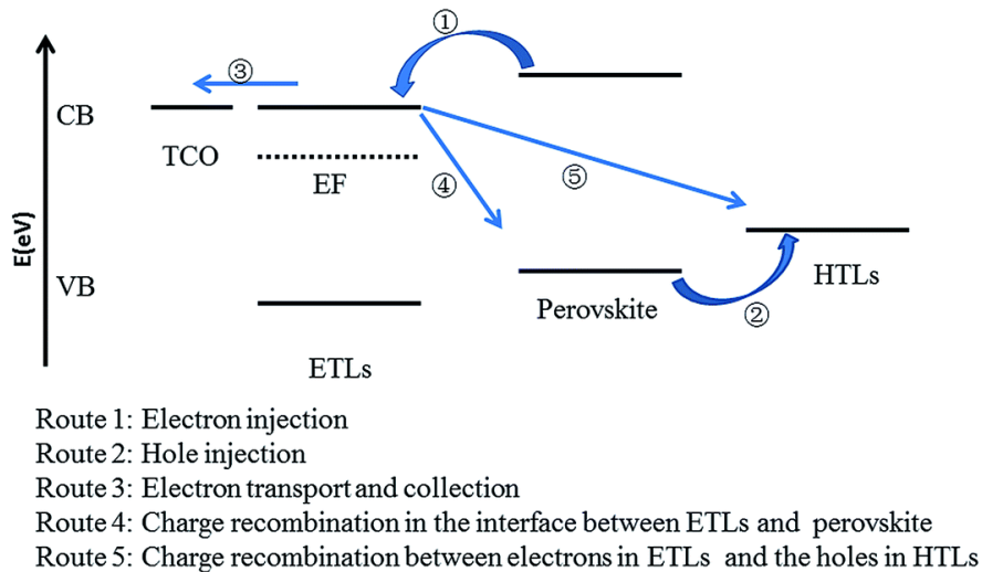
Figure 2.2 Charge transfer/recombination processes in PSCs 24
