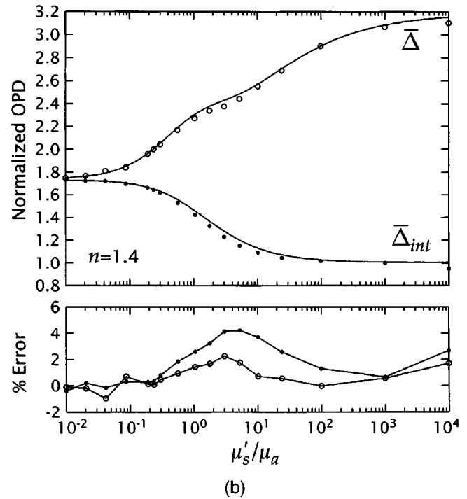
Fig. 7 Normalized optical penetration depths \bar{\Delta} \equiv \mu_{eff}\Delta (○) and \bar{\Delta}_{int} \equiv \mu_{eff}\Delta_{int} (●) versus (\mu'_s/\mu_a) as predicted by the \delta - P_1 approximation (solid curves) and MC simulations (symbols) for planar illumination under refractive index (a) matched ( n=1.0 ) and (b) mismatched ( n=1.4 ) conditions. Lower plots show the percentage error of the \delta - P_1 predictions relative to the MC simulations.
