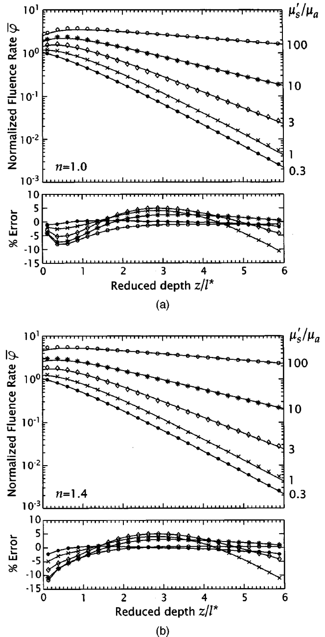
Fig. 3 Normalized fluence rate \bar{\phi} versus reduced depth ( z/l^* ) as predicted by the \delta - P_1 approximation (solid curves) and Monte Carlo simulations (symbols) for planar illumination under refractive index (a) matched ( n=1.0 ) and (b) mismatched ( n=1.4 ) conditions. Profiles are shown for (\mu'_s/\mu_a) = 100 ( \circ ), 10 ( * ), 3 ( \diamond ), 1 ( \times ), and 0.3 ( \bullet ) with g=0.9 . Lower plots show the percentage error of the \delta - P_1 predictions relative to the Monte Carlo simulations using the same symbols as the main plot.
