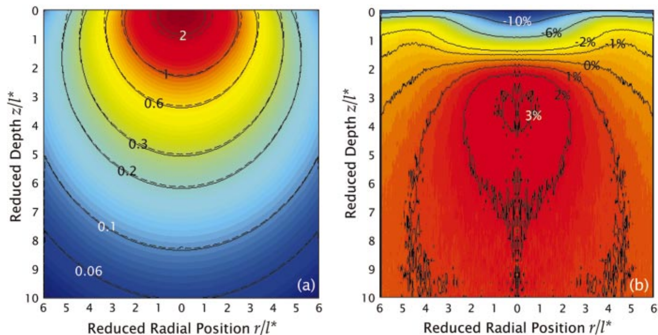
Fig. 12 (a) Color contour plot of the normalized fluence rate \bar{\varphi}(r, z) as predicted by both the \delta - P_1 approximation (solid contours and color) and MC simulations (dashed contours) for Gaussian beam irradiation with r_0 = 3l^* in media with (\mu'_s/\mu_a) = 100 for g = 0.9 under refractive index mismatched conditions ( n = 1.4 ); and (b) relative error between \delta - P_1 approximation and MC simulations.
