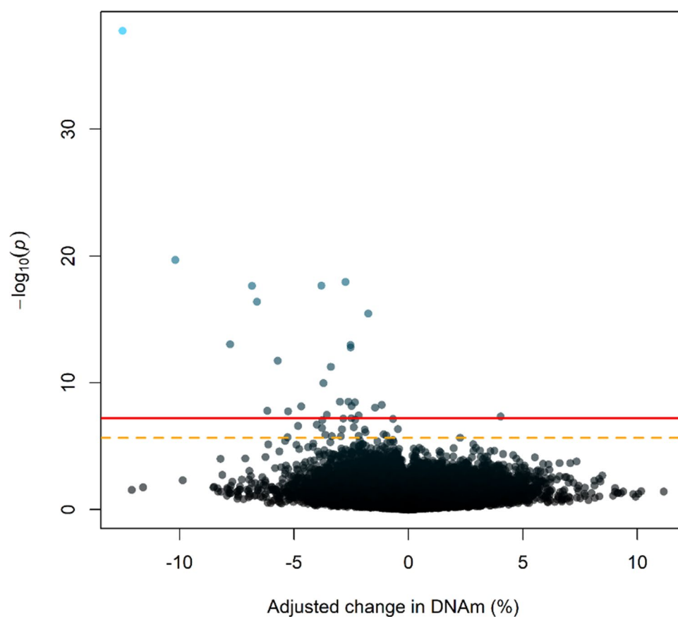
Figure 2. Volcano plot of the -\log_{10}(p\text{-values}) against adjusted regression coefficients for each CpG for the Epigenome-Wide Association Study comparing current smokers to non-smokers (red solid line represents a Bonferroni corrected level of significance; orange dotted line represents a false discovery rate of 5%).
