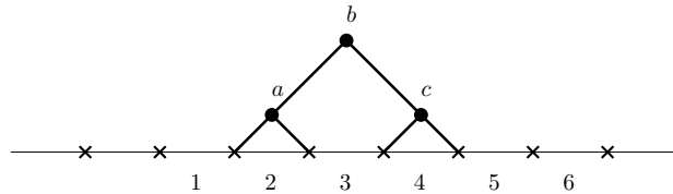
Figure 3.3: An indexed forest F with c(F) = (0, 2, 0, 1) .
