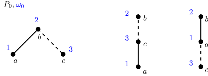
Figure 2.1: A labeled poset and its two linear extensions.
