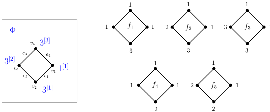
Figure 3.1: A poset with labeled flag (P, \Phi) and its five (P, \Phi) -partitions.
