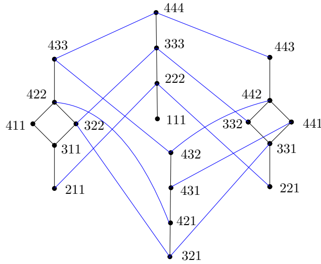
Figure 5.1: Hasse diagram of the convex subset of \mathcal{P}_3 formed by all words below 444 and with positive letters.
