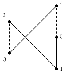
Figure 2.2: Counterexample to an argument in the proof of [AB20, Proposition 4.3].
