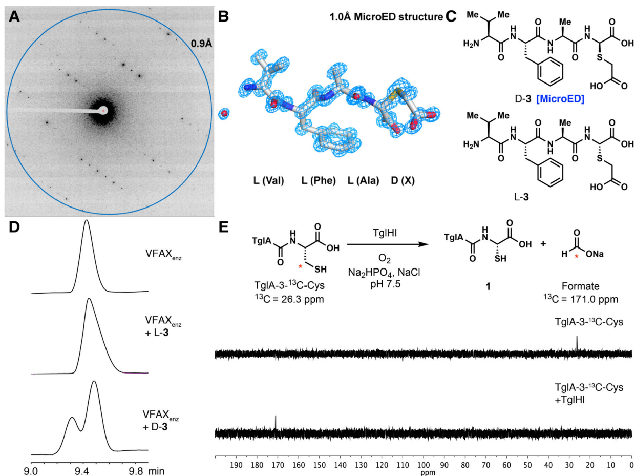
Figure 3. In vitro TglHI reacts with 13 C-labeled TglA-Cys to produce 13 C-formate and 1 with retention of configuration.
