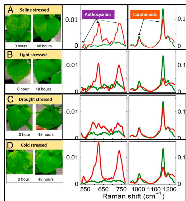
Figure 3. The Raman spectra of unstressed plants (green curves) and stressed plants at 48 h after stress (red curves) of (A) saline, (B) light, (C) drought, and (D) cold. Insets: Photos of coleus leaves for unstressed (left) and stressed (right) plants. Adapted with permission from ref 17. Copyright 2017 National Academy of Sciences.
