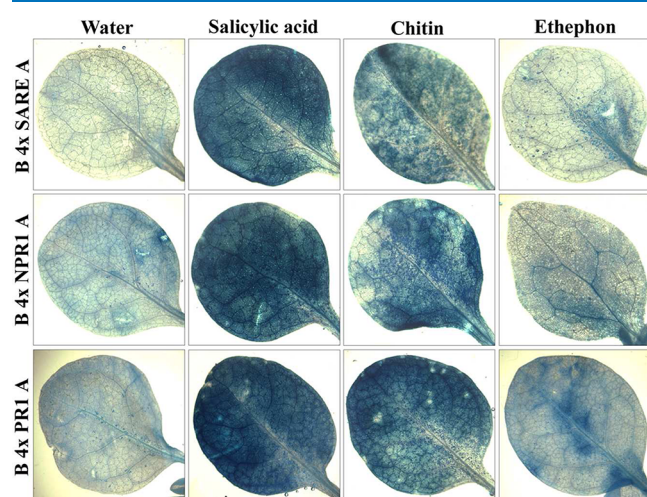
Figure 1. Histochemical analysis of GUS expression in transgenic tobacco plants exposed to salicylic acid, chitin, or ethephon treatments for 24 h. Adapted with permission from ref 7. Copyright 2008 Multidisciplinary Digital Publishing Institute.
