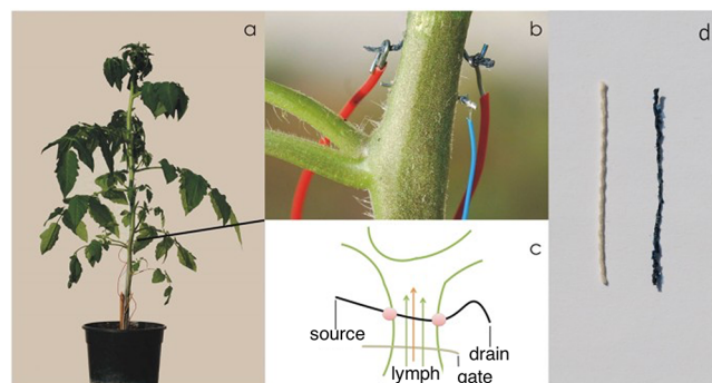
Figure 4. (a) A bioristor integrated in a tomato plant. (b) Detail of the textile device implantation and the silver gate connected through the plant stem. (c) Sketch of the proposed biosensor device showing the electrical connections. Green lines: sketch of plant stems. Black line: textile thread. Grey line: gate electrode. Arrows: lymph flow. (d) Cotton thread untreated (left) and functionalized with PEDOT:PSS (right). Adapted with permission from ref 27. Copyright 2017 Nature Publishing Group.
