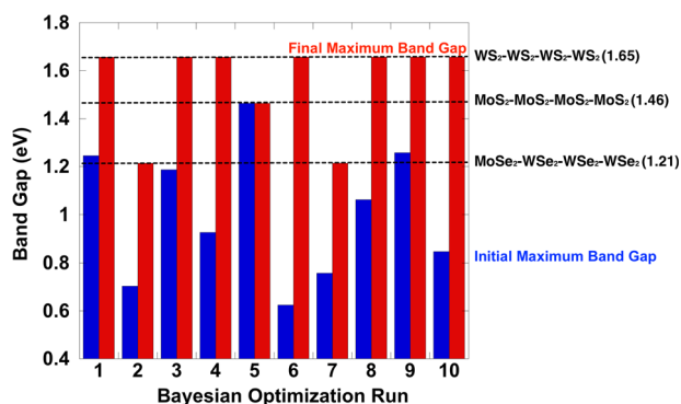
Fig. 4 Initial and final maximum band gap values for ten different BO runs on the class of four-layered hetero-structures. Optimal structures, along with their band gap value are labeled
