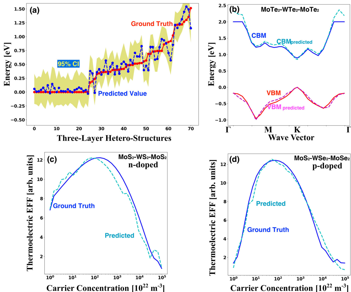
Fig. 2 a Predicted (blue) and ground truth (red) band gap values of three-layer hetero-structures in the test data set. Yellow shading represents a 95% confidence interval (CI) of the predicted results. b Predicted (dashed lines) and ground truth (solid lines) values for the VBM and CBM dispersion curves in momentum space for a sample three-layered hetero-structure. c , d Predicted (dashed lines) and ground truth (solid lines) thermoelectric EFF curves versus carrier concentration for a sample n(p)-type-doped three-layered hetero-structure. In all models, 60% of the three-layered structures were randomly selected to comprise the training data set
