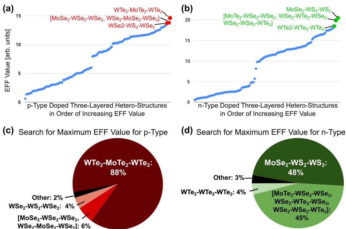
Fig. 5 a , and b Thermoelectric EFF values for all p-type-doped a and n-type-doped b three-layered hetero-structures, where hetero-structures on the x-axis are ordered by increasing EFF value. Points highlighted in red and green denote hetero-structures returned most frequently as the optimal structure by a BO model searching for the p-type- and n-type-doped structures, respectively, with maximum EFF value. c , d Pie chart showing the distribution of optimal thermoelectric structures returned in 500 independent BO searches for the p-type-doped c and n-type-doped d materials with maximum EFF value
