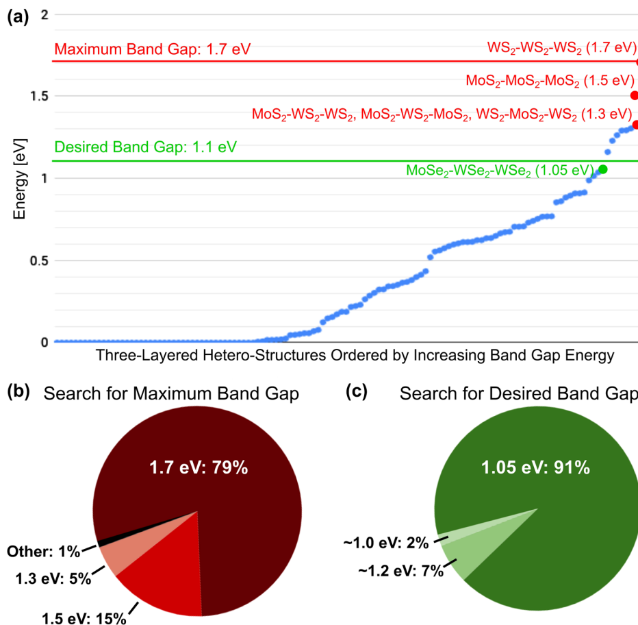
Fig. 3 a Band gap values for all three-layered hetero-structures, where hetero-structures on the x-axis are ordered by increasing band gap value. A table of structure names and corresponding band gap values is found as Table S5 in Supplementary Information. Highlighted points denote hetero-structures returned most frequently as the optimal structure by a BO model searching for the maximum band gap (red) and a desired value of 1.1 eV (green). b Pie chart showing the distribution of optimal band gap values returned in 500 independent BO searches for the maximum band gap. c Pie chart showing the distribution of optimal band gap found in 500 independent BO searches for a desired band gap value of 1.1 eV. \text{MoSe}_2\text{-WSe}_2\text{-WSe}_2 , with a band gap of 1.05 eV, has the closest band gap value to 1.1 eV and was returned as the optimal structure in 91% of the 500 independent BO searches. \text{WSe}_2\text{-WSe}_2\text{-WSe}_2 and \text{MoS}_2\text{-MoS}_2\text{-WS}_2 , with band gap values of 1.23 and 1.26 eV, respectively, were returned in 7% of the BO searches, while \text{WSe}_2\text{-MoSe}_2\text{-WSe}_2 and \text{MoSe}_2\text{-WSe}_2\text{-MoSe}_2 , with band gap values of 1.01 and 1.04 eV, respectively, were returned in the remaining 2% of BO searches
