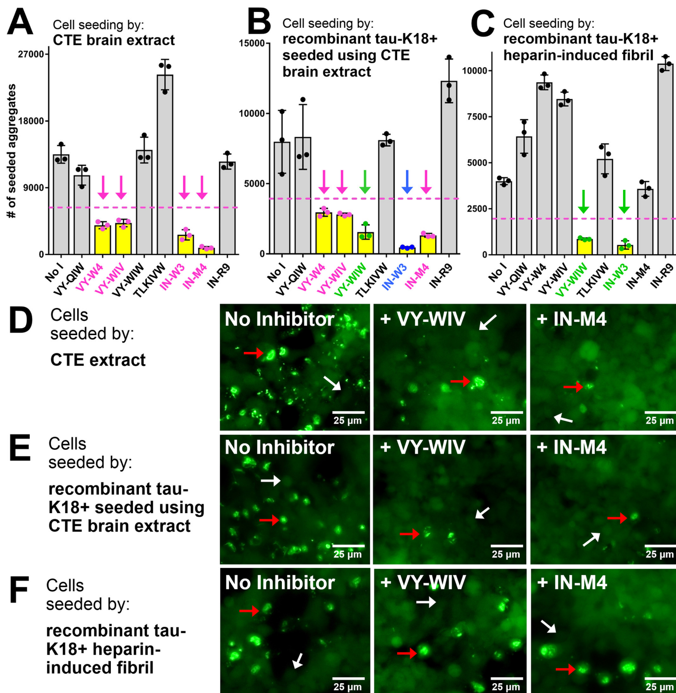
Figure 5. Inhibitor sensitivity of CTE-derived tau seeds. A–C, seeding by crude brain extract from the temporal cortex (A), recombinant tau-K18+ fibrils that were seeded with CTE-derived tau seeds (B), or recombinant tau-K18+ fibrils that were aggregated in the presence of heparin (C). Seeding inhibition measurements for the CTE-seeded recombinant fibril polymorph in B were carried out in tau biosensor cells after three sequential rounds of in vitro seeding. Seeding inhibition was measured by counting the number of fluorescent puncta as a function of inhibitor. In A–C, magenta arrows were used to mark capping inhibitors that were effective at blocking seeding by CTE-derived tau from crude brain extracts, green arrows mark inhibitors effective at blocking seeding by recombinant tau-K18 fibrils, and the blue arrow marking IN-W3 in B emphasizes that it is the only one of the inhibitors that blocks seeding by both the CTE-derived tau and recombinant tau fibrils. D–F, representative images from A, B, and C, respectively, showing seeding and inhibition in tau-K18 biosensor cells. Red arrows, representative cells containing seeded tau aggregates; white arrows, representative cells lacking aggregated tau. Error bars, S.D.
