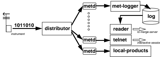
Figure 2: Instrument Node Data Flow
