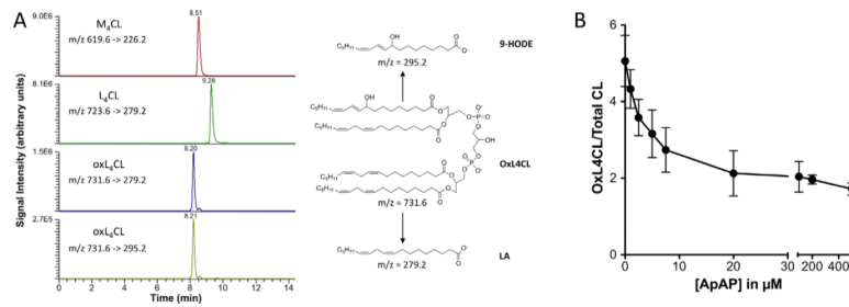
Figure 2. ApAP inhibits cyt c-catalyzed oxidation of cardiolipin
