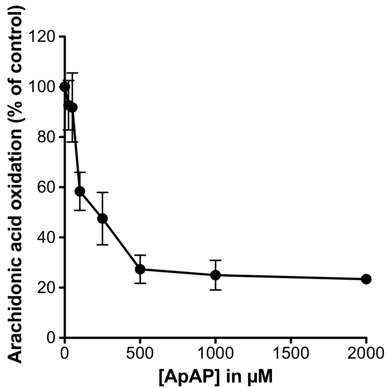
Figure 1. ApAP inhibits cyt c induced oxidation of arachidonic acid (AA)
