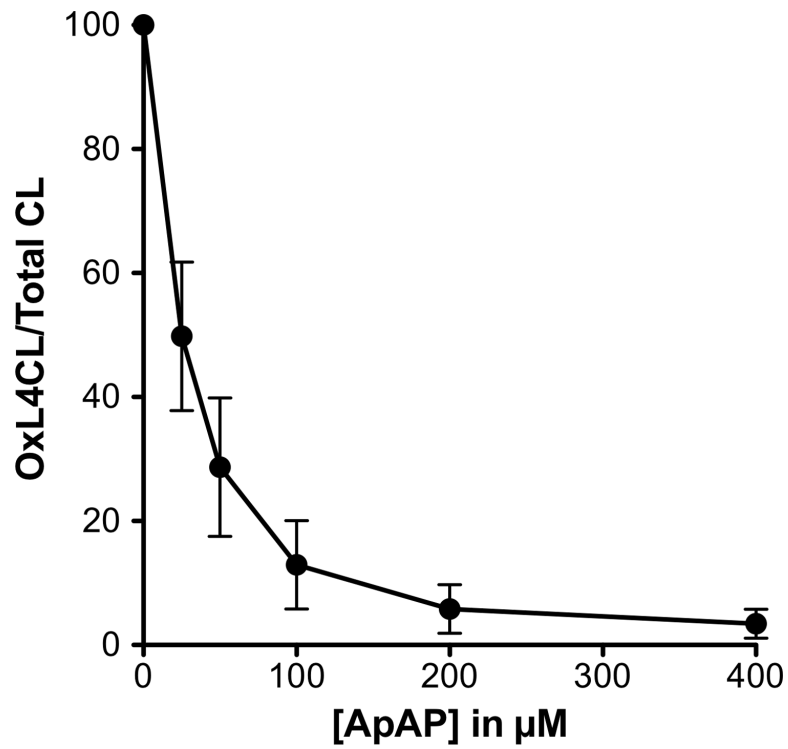
Figure 3. ApAP inhibits CL oxidation in isolated mitochondria
