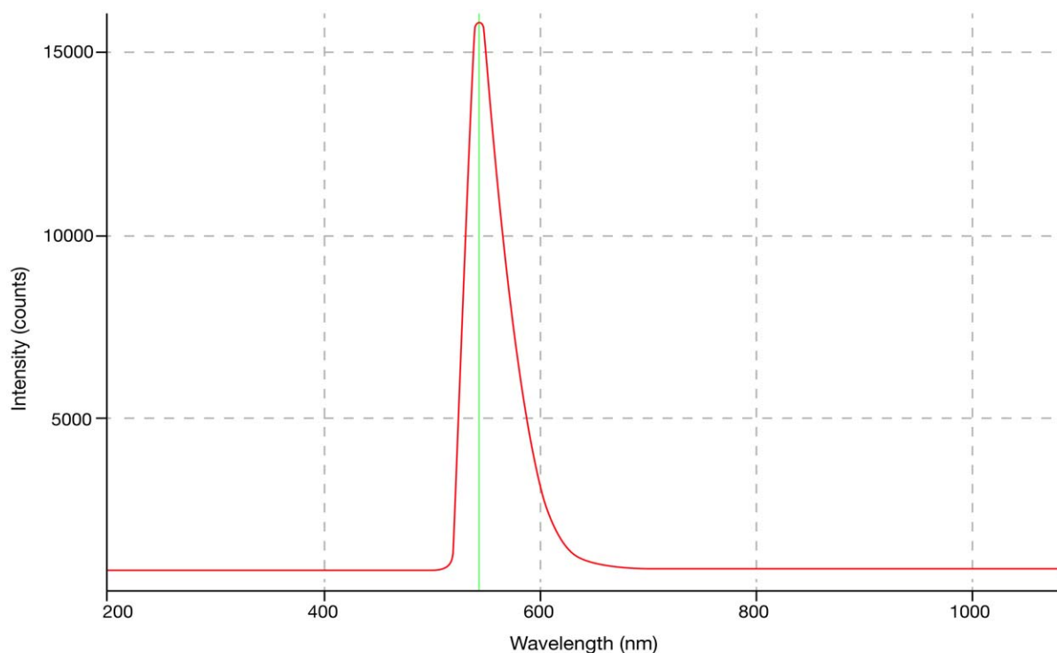
Figure 2. Pyromethene 556, 0.15 g/L. Peak at 544 nm.
