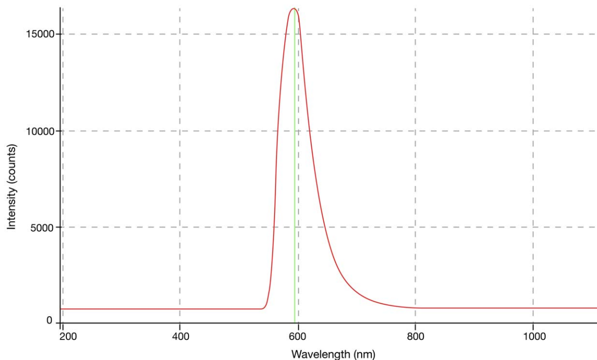
Figure 3. Rhodamine 590, 0.0375 g/L. Peak 592 nm. doi:10.1371/journal.pone.0035899.g003
