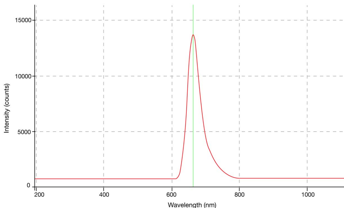
Figure 4. Sulphorhodamine 640, 0.75 g/L. Peak at 658 nm. doi:10.1371/journal.pone.0035899.g004
