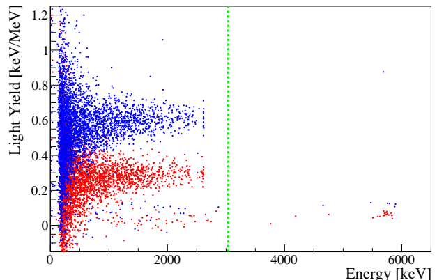
Fig. 4 Light yield measured in a LD as a function of the energy deposited in the LMO surrounded by the reflecting foil (Blue) and LMO without reflector (Red). Data were collected with a ^{232}\text{Th} \gamma source and a smeared \alpha source.
