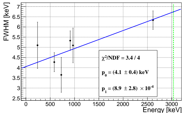
Fig. 3 FWHM energy resolution as a function of the energy. Data were fitted with a linear function: FWHM = p_0 + p_1 \times E (blue line). Green dotted line (color online): Q_{\beta\beta} of ^{100}\text{Mo} .
