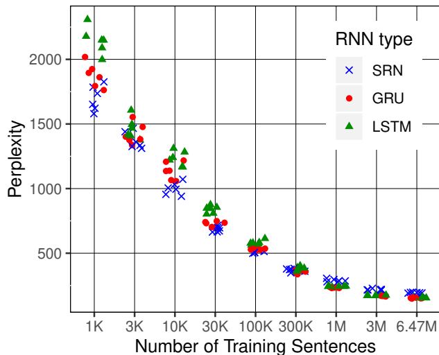
Figure 1: Perplexity on the experimental sentences for each of three RNN types at nine different training corpus sizes. At each training size there are six models of each type with different sentence orderings and initial weights. Data points are subjected to horizontal jitter to improve readability.
