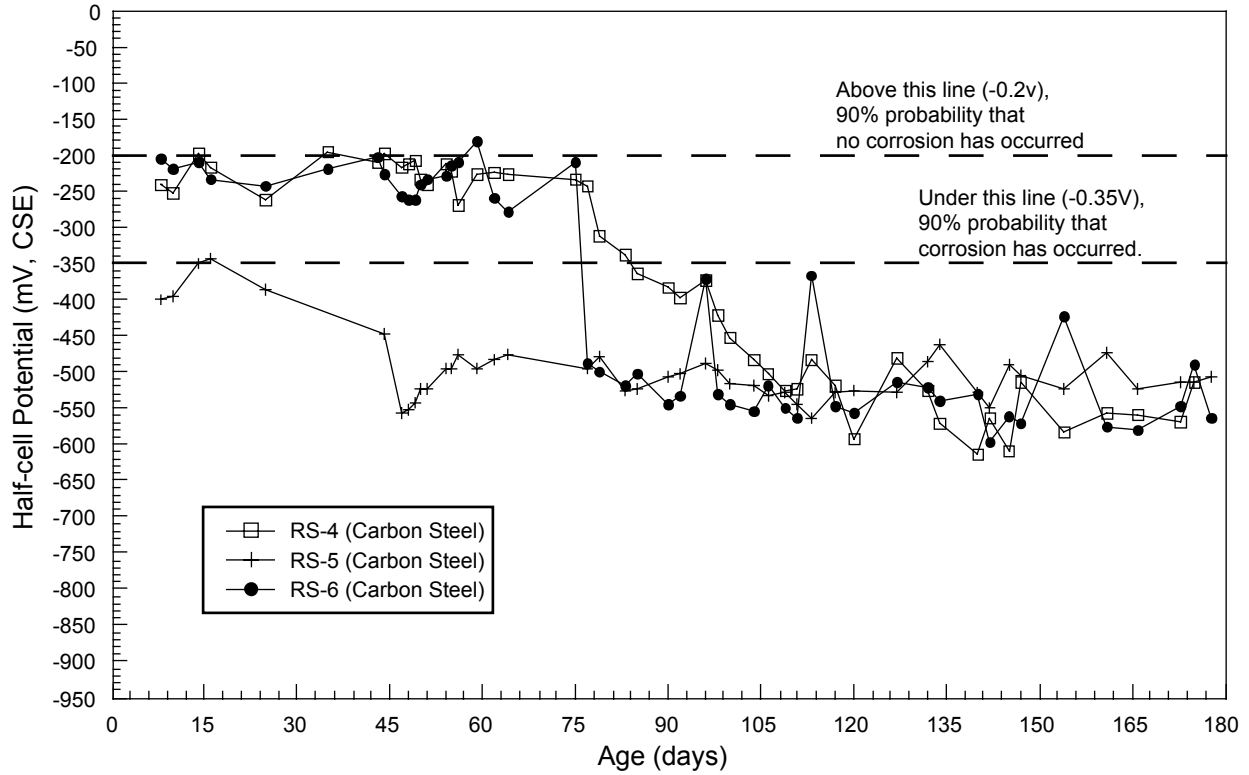
Figure 12. Half-cell potentials of carbon steel bars in Chloride ponding at 40-43°C.
