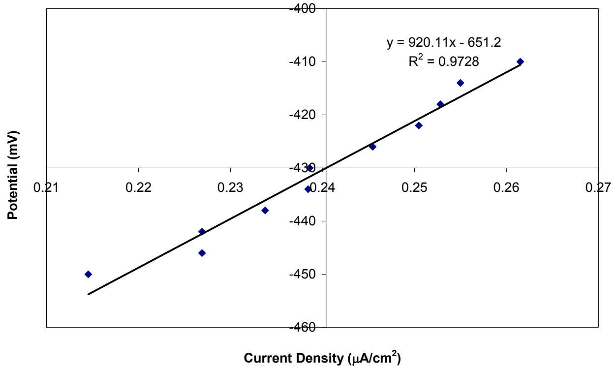
Figure 51. Linear Polarization Resistance, WSDOT slab, Specimen A.
