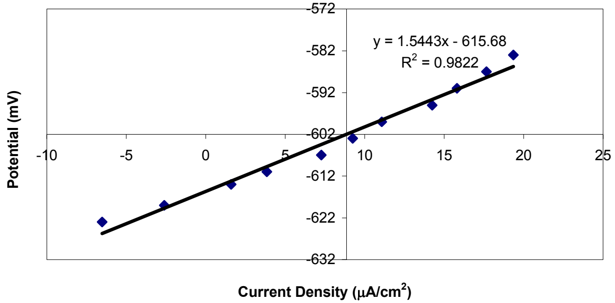
Linear Polarization Resistance Carbon Steel - 2
