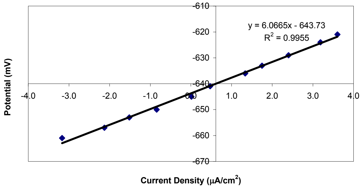
Linear Polarization Resistance Carbon Steel - 2
