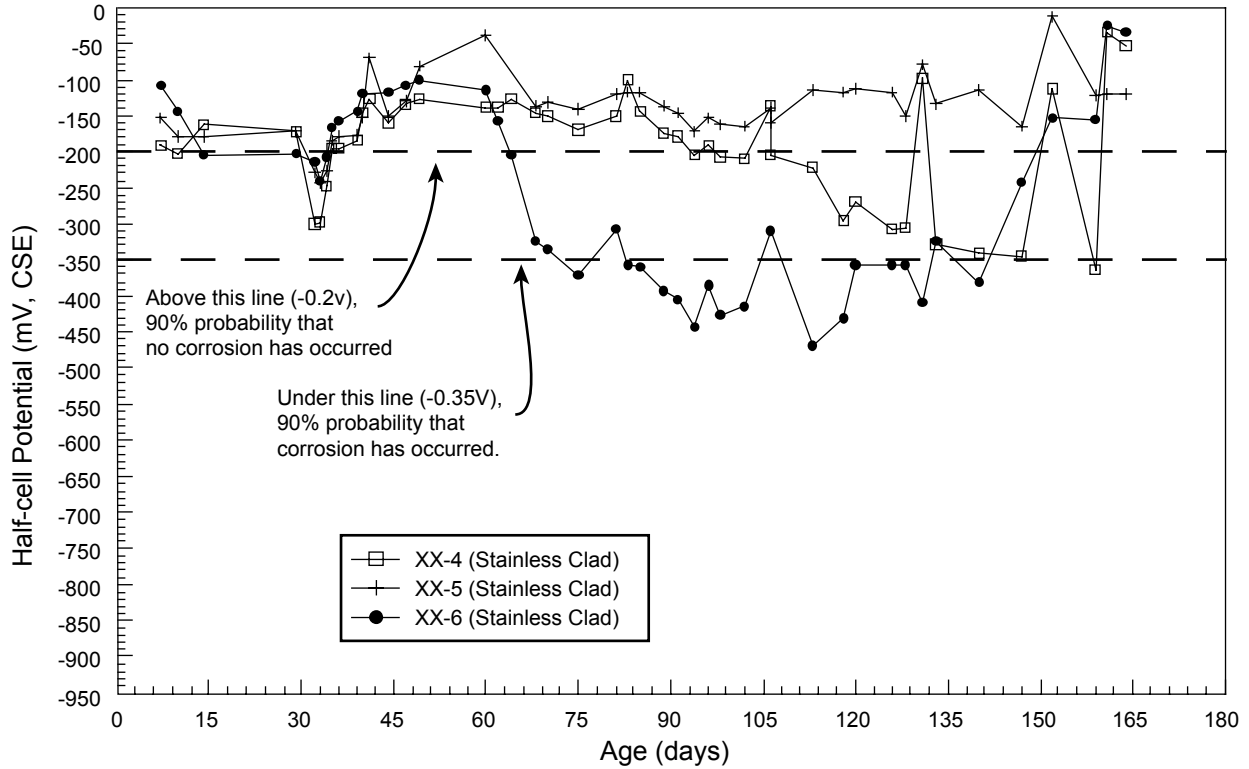
Figure 18. Half-cell potentials of stainless clad steel bars in Chloride ponding at 40-43°C.
