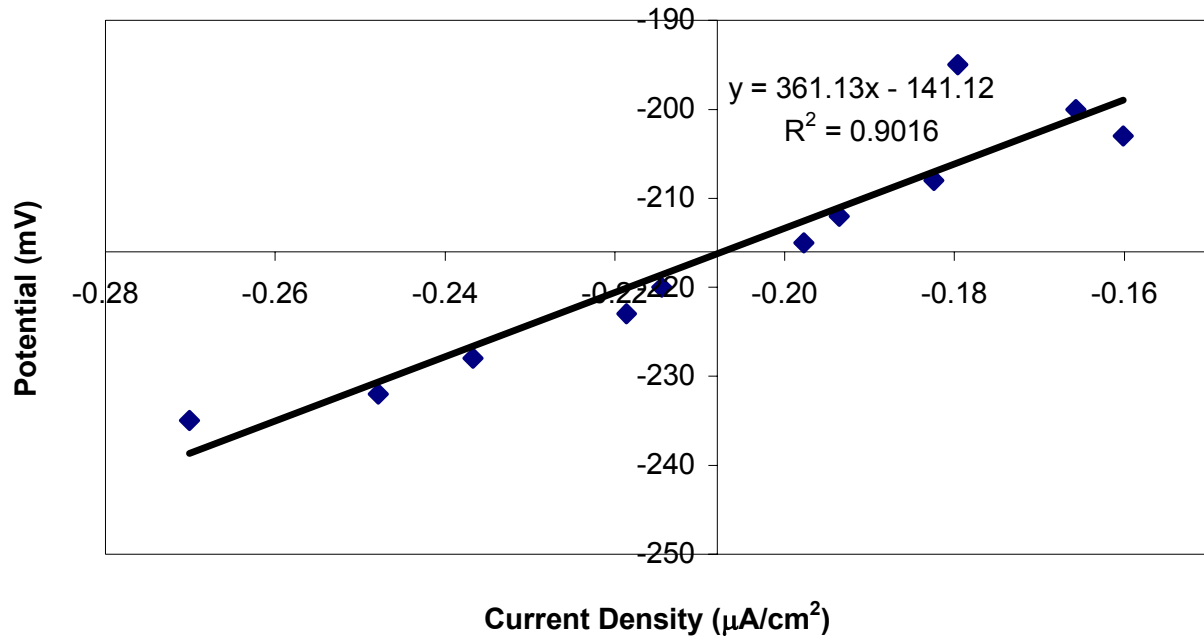
Linear Polarization Resistance Stainless Steel Clad - 3
