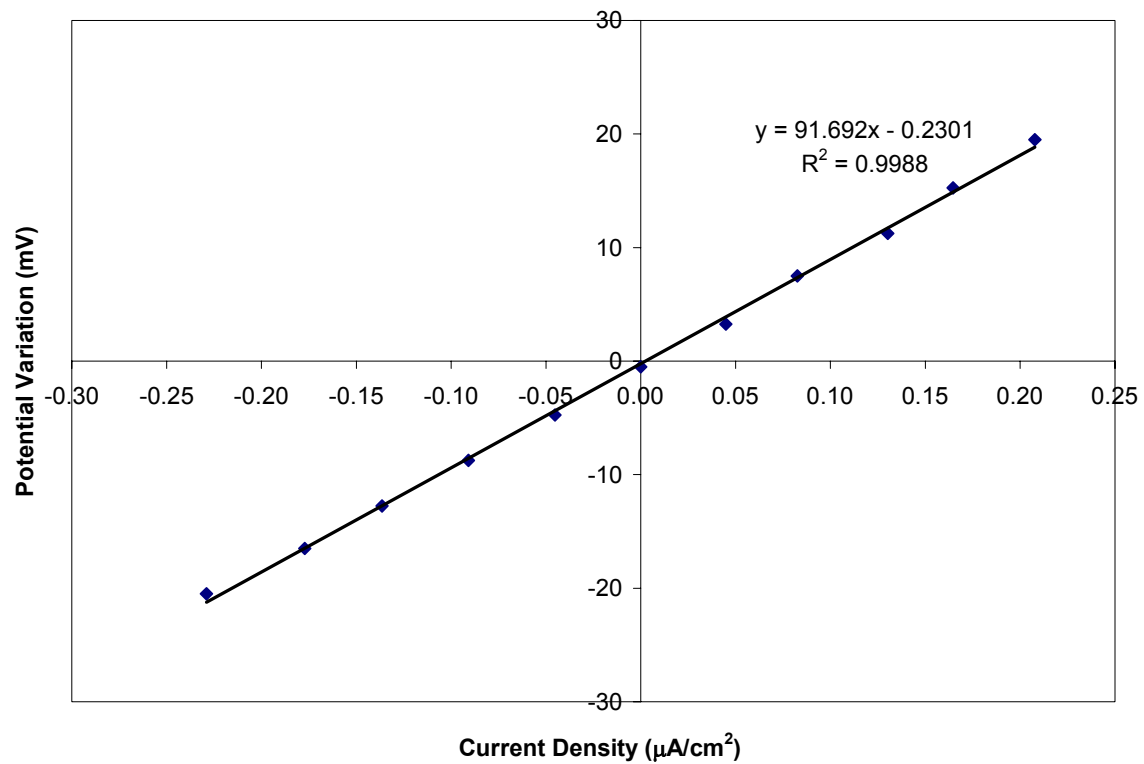
Figure 30. Linear Polarization Resistance results for non-flexible, purple epoxy-coated dowels.
