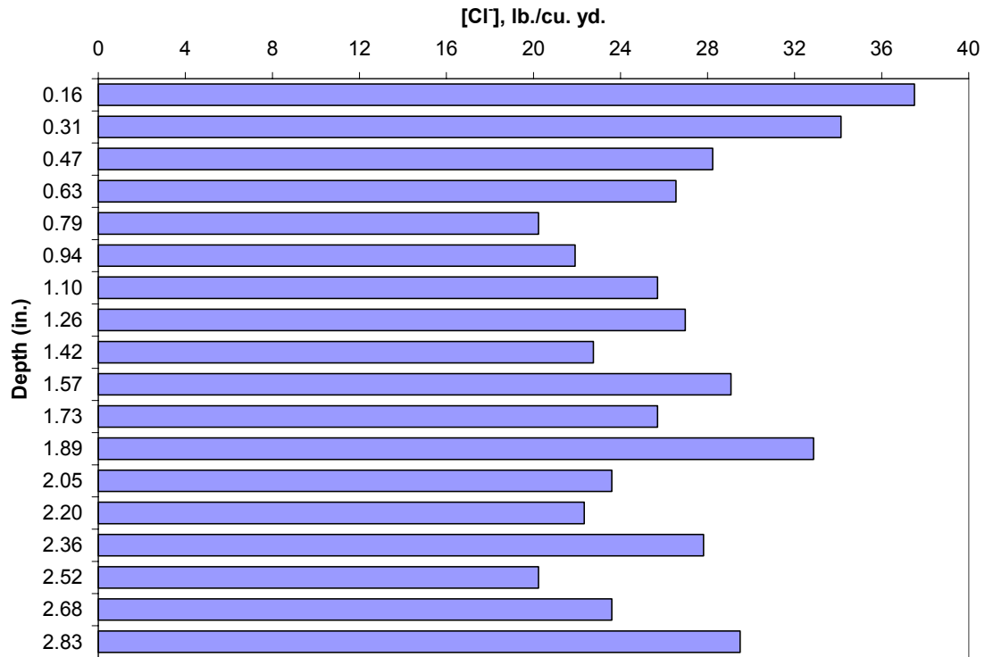
Figure 67. Chloride profile on the concrete of a stainless clad specimen.
