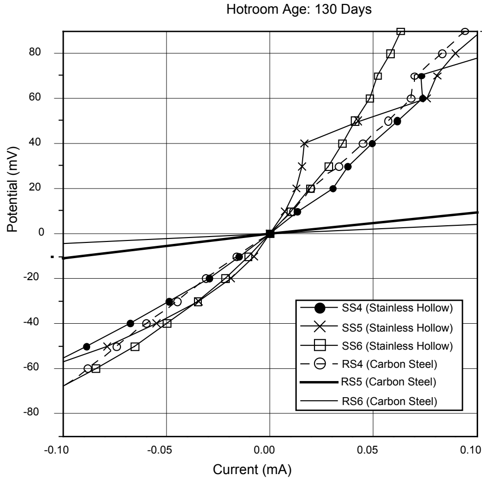
Figure 20. Linear Polarization of the carbon and stainless steels at 40-43°C.
