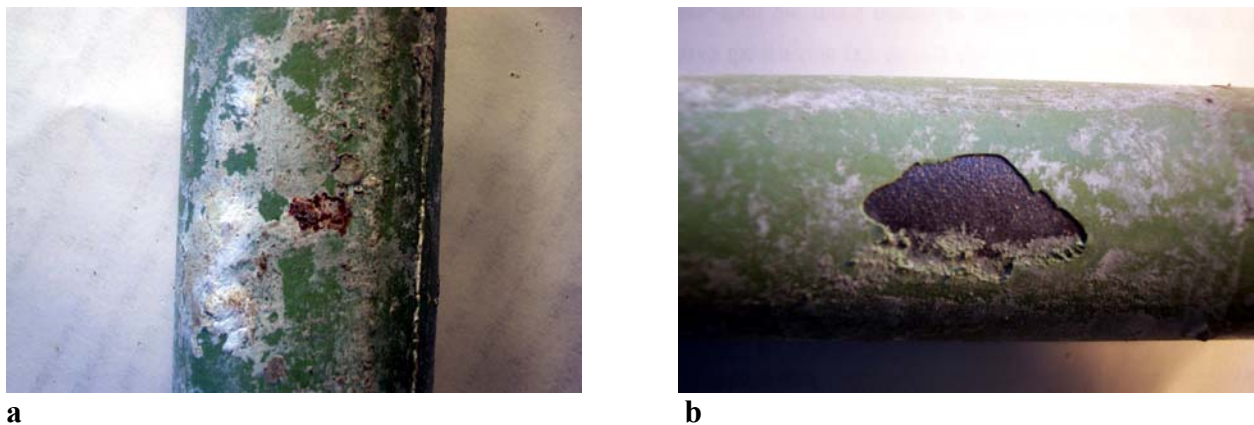
Figure 43. Corrosion product concentrated in a defective area in the epoxy coating (a); part of the epoxy coating was removed in order to observe the state of the carbon steel beneath the coating (b).
