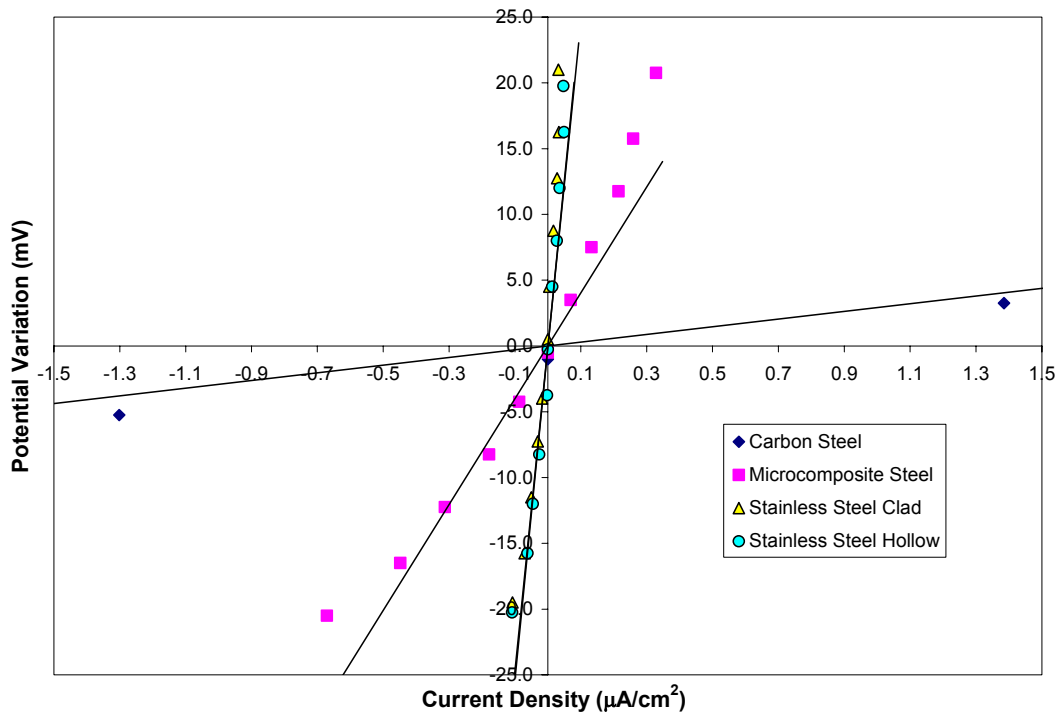
Figure 34. Detail of the region around the half-cell potential. The greater the slope, the higher the corrosion resistance.
