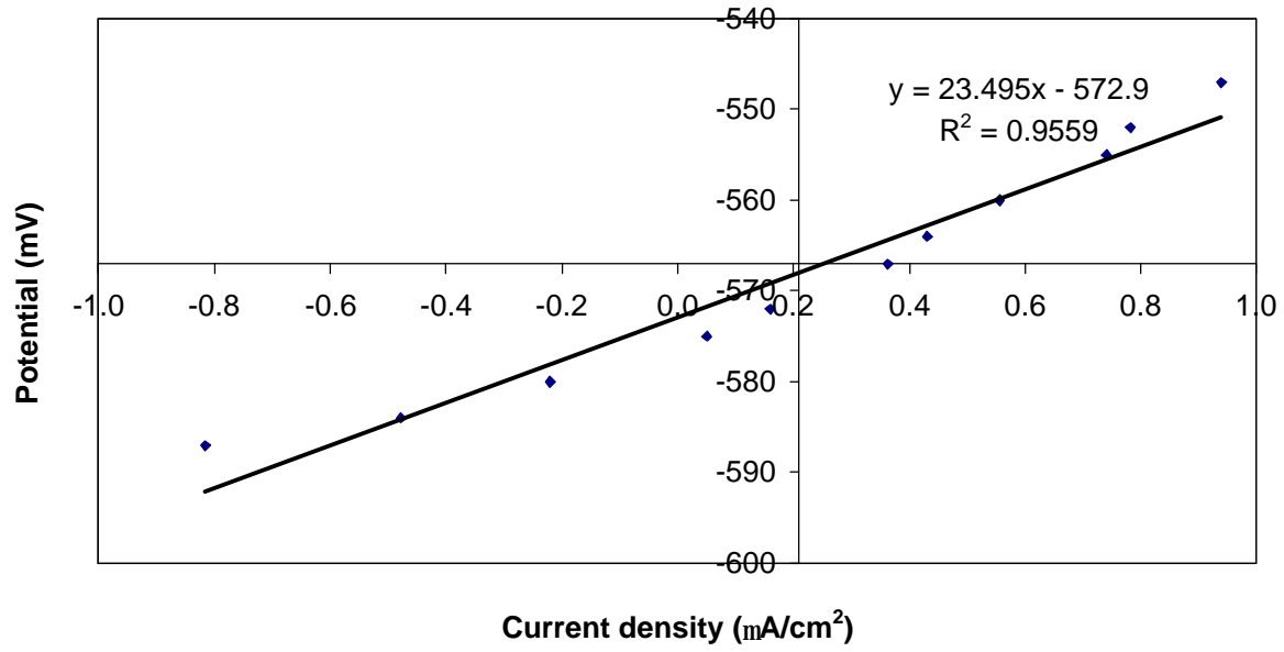
Linear Polarization Microcomposite - 1
