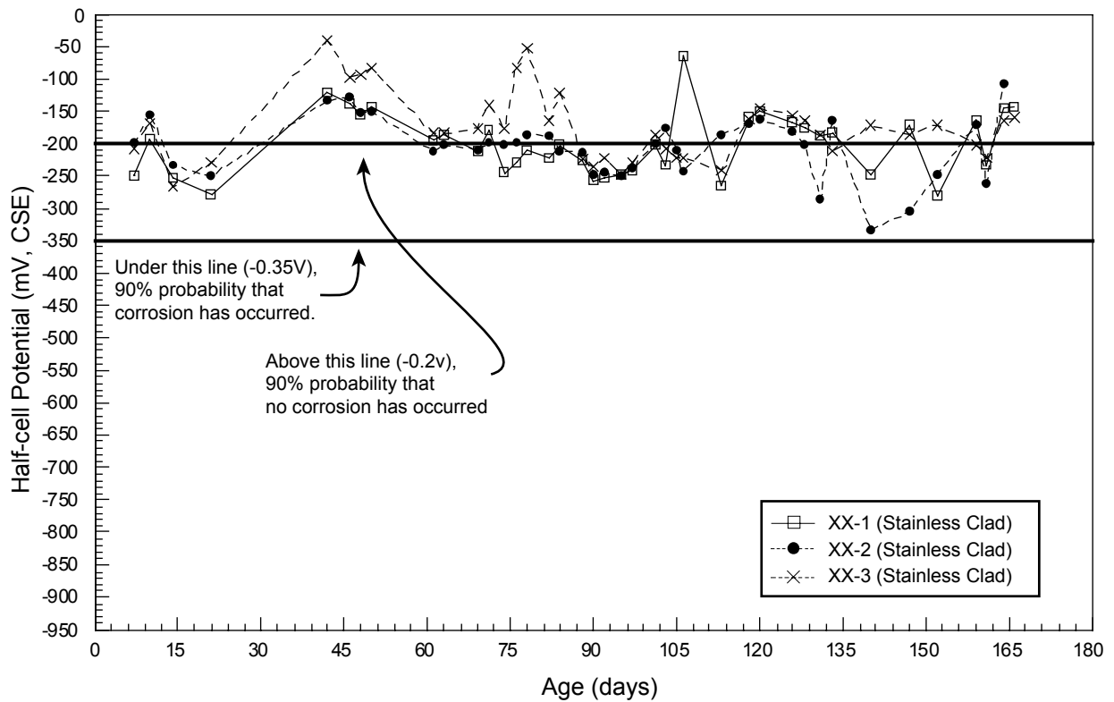
Figure 19. Half-cell potentials of stainless clad steel bars in Chloride ponding at 4.4°C.
