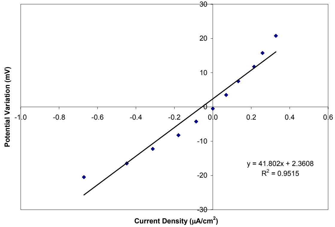
Figure 27. Linear Polarization Resistance results for microcomposite steel dowels.
