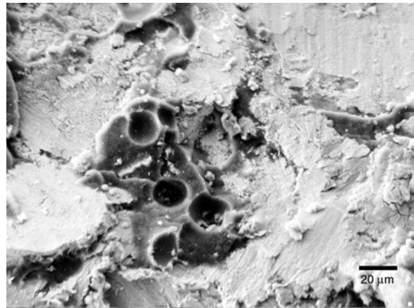
Figure 49. Green-epoxy-coated samples: (a) general view of the surface, 100×; (b) region where part of the epoxy coating was removed, 100×; (c) condition of the steel underneath the epoxy, 302×; (d) detail of corroded area and pits present under the coating, 1330×.
