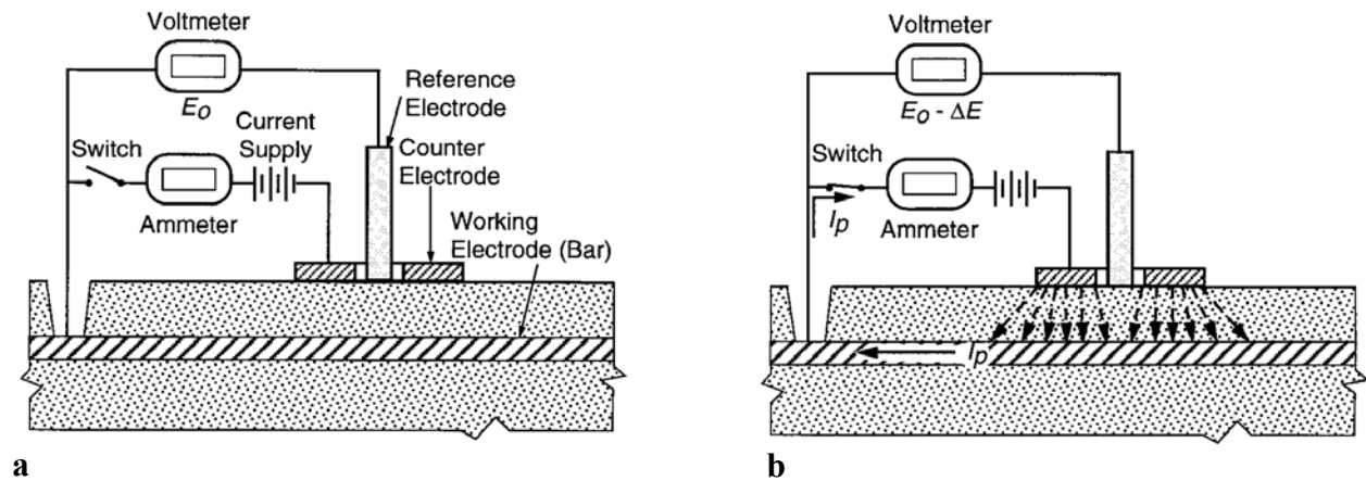
Figure A2. Three-electrode Linear Polarization Resistance method. (a) Measurement of the open-circuit potential (half-cell potential); (b) Current applied to the counter electrode to produce a small change in voltage \Delta E .(12)
