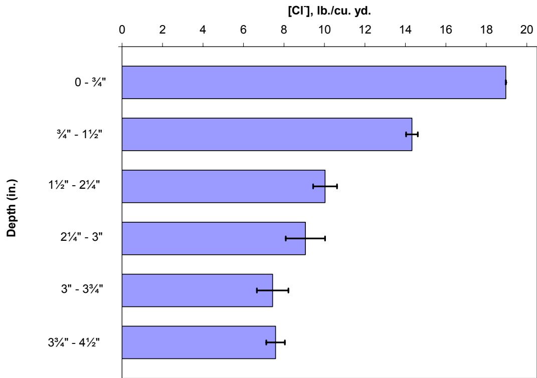
Figure 63. Chloride profile for SR 90 MP 61.304 (Price Creek).
