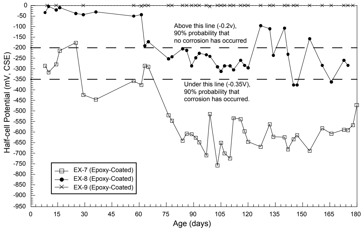
Figure 15. Measured potentials of epoxy-coated bars in Chloride ponding at 4.4°C.
