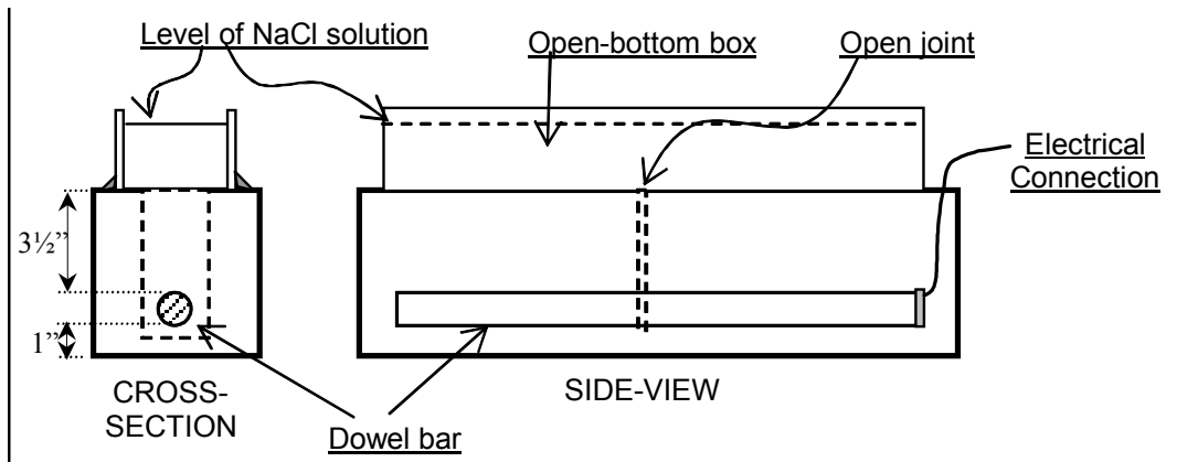
Figure 9. Experiment setup to accelerate corrosion using chloride ponding.
