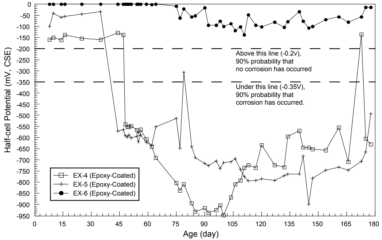
Figure 14. Half-cell potentials of epoxy-coated bars in Chloride ponding at 40-43°C.
