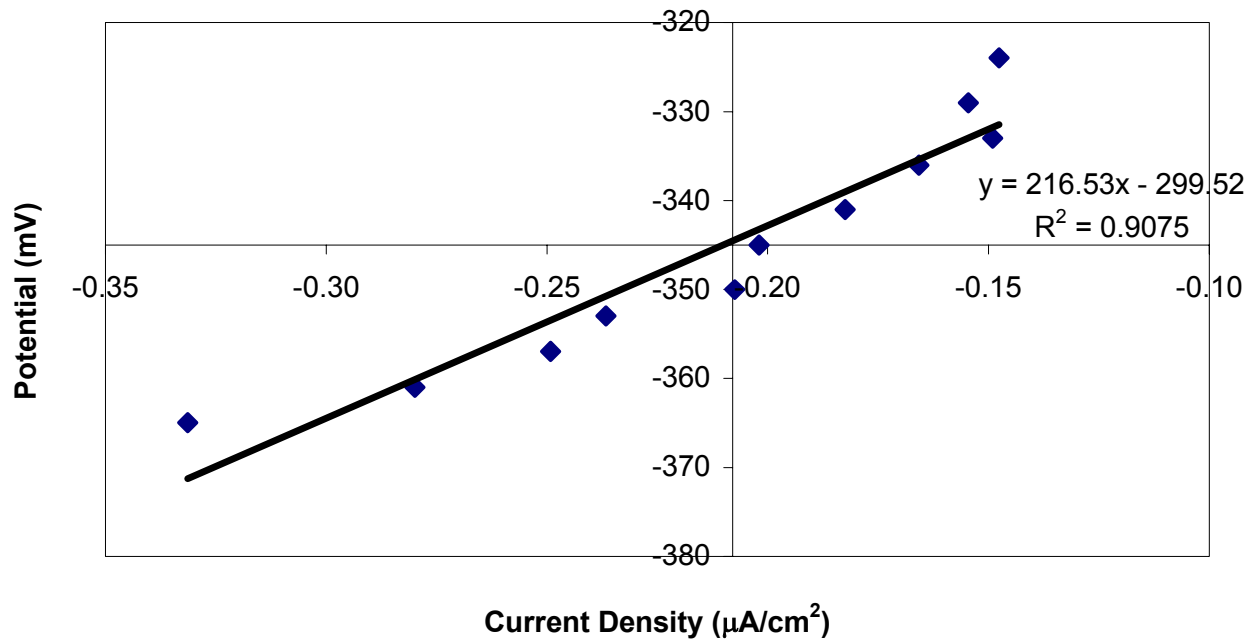
Linear Polarization Resistance Stainless Steel Clad - 4
