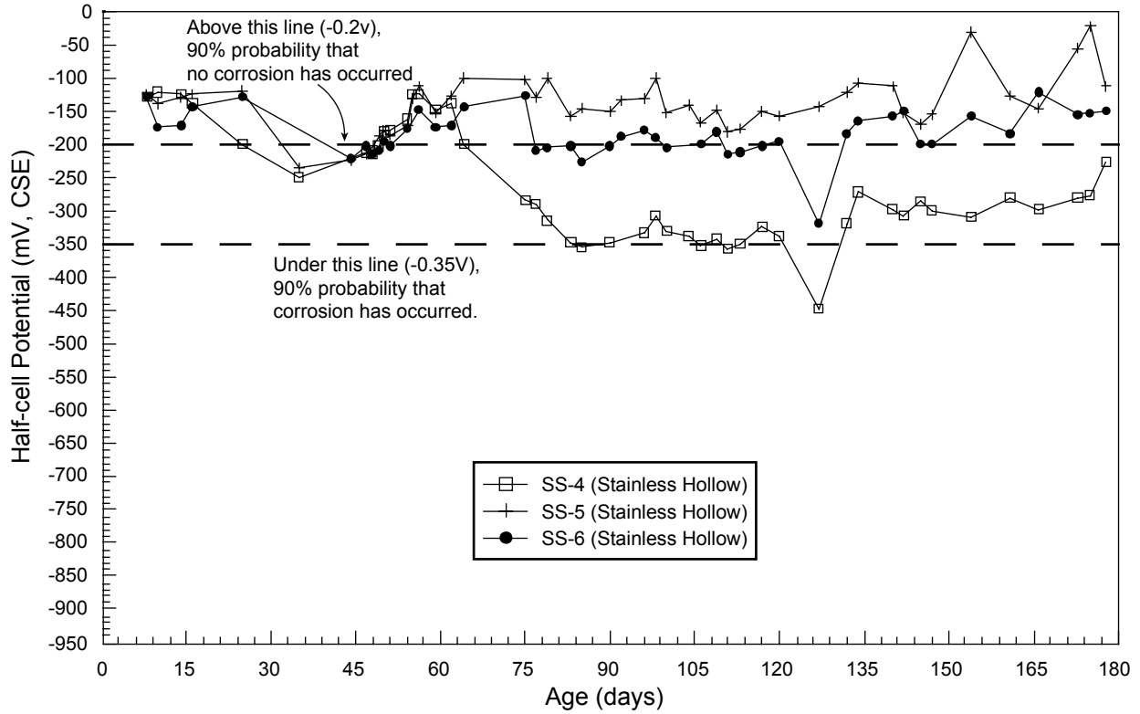
Figure 16. Half-cell potentials of stainless hollow steel bars in Chloride ponding at 40-43°C.
