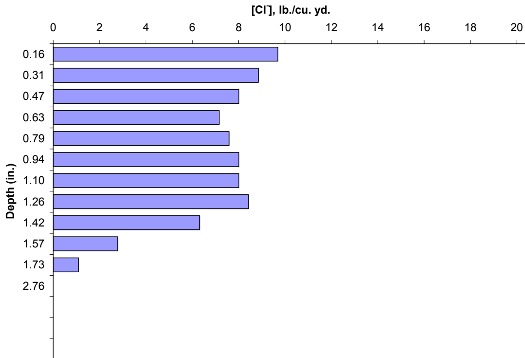
Figure 59. Chloride profile of the grout around the pavement joint (Core #5).
