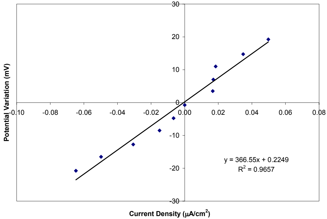
Figure 31. Linear Polarization Resistance results for non-flexible gray epoxy-coated dowels.
