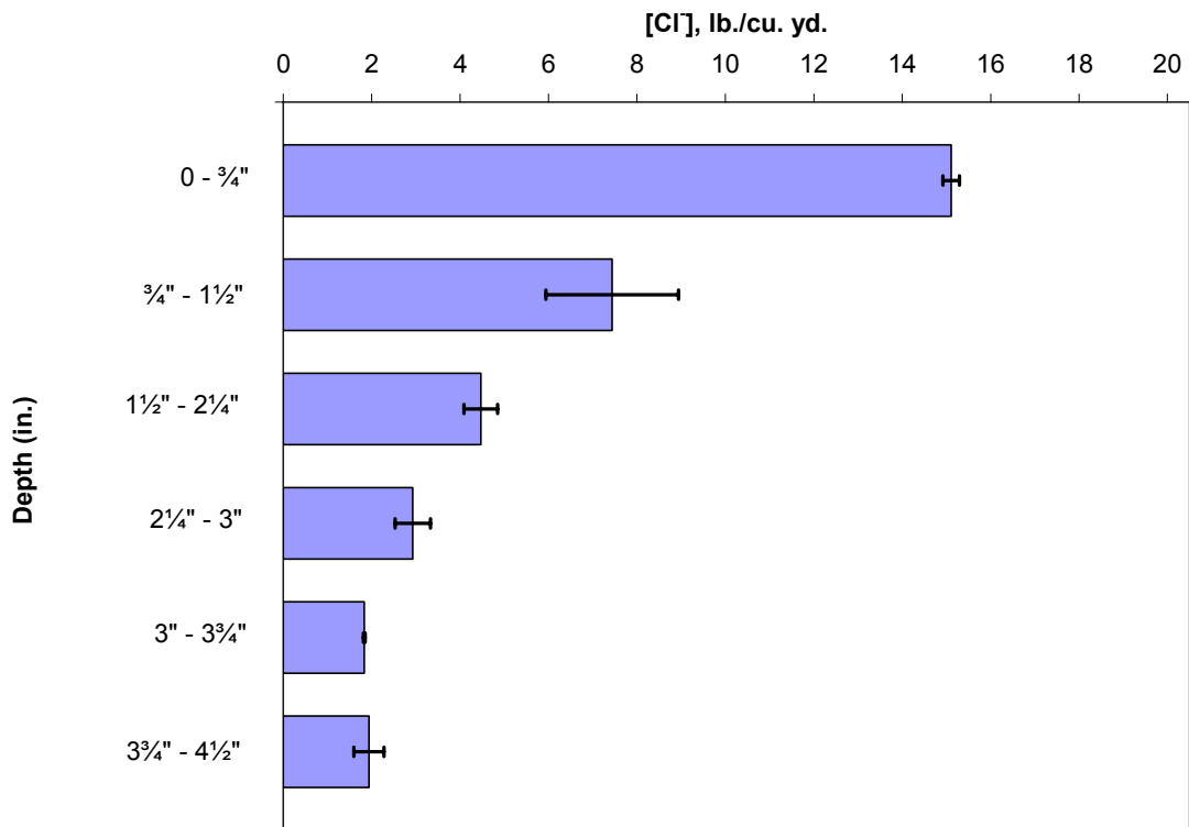
Figure 64. Chloride profile for SR 82 MP 10.617 (Military Road).
