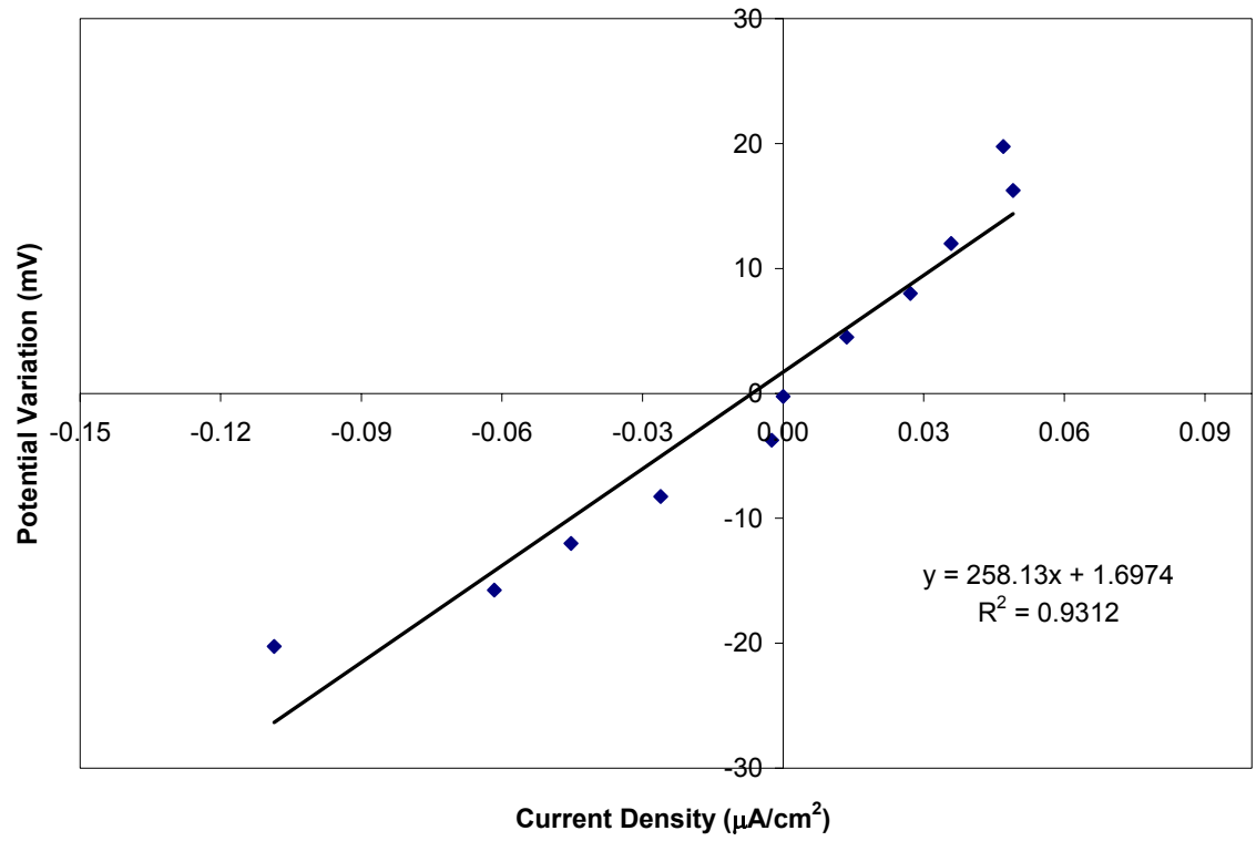
Figure 29. Linear Polarization Resistance results for stainless steel hollow dowels.
