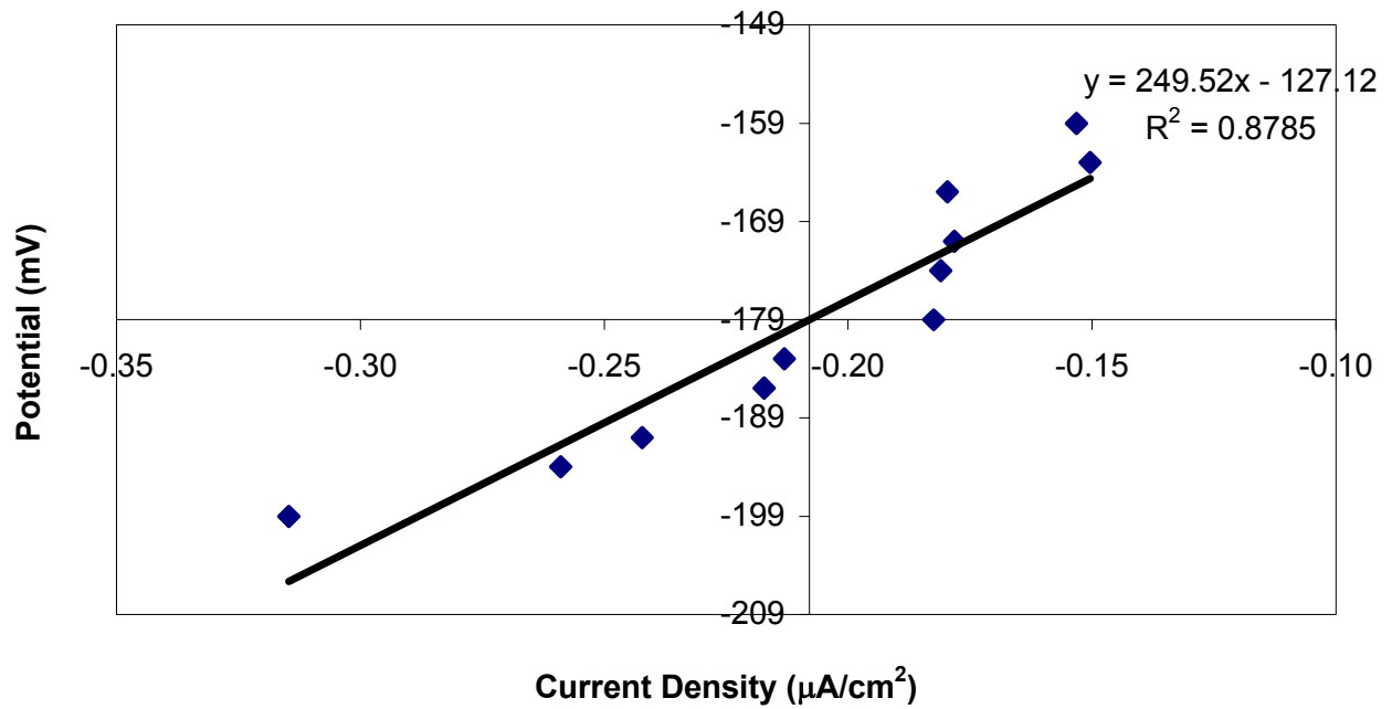
Linear Polarization Resistance Stainless Steel Clad - 2
