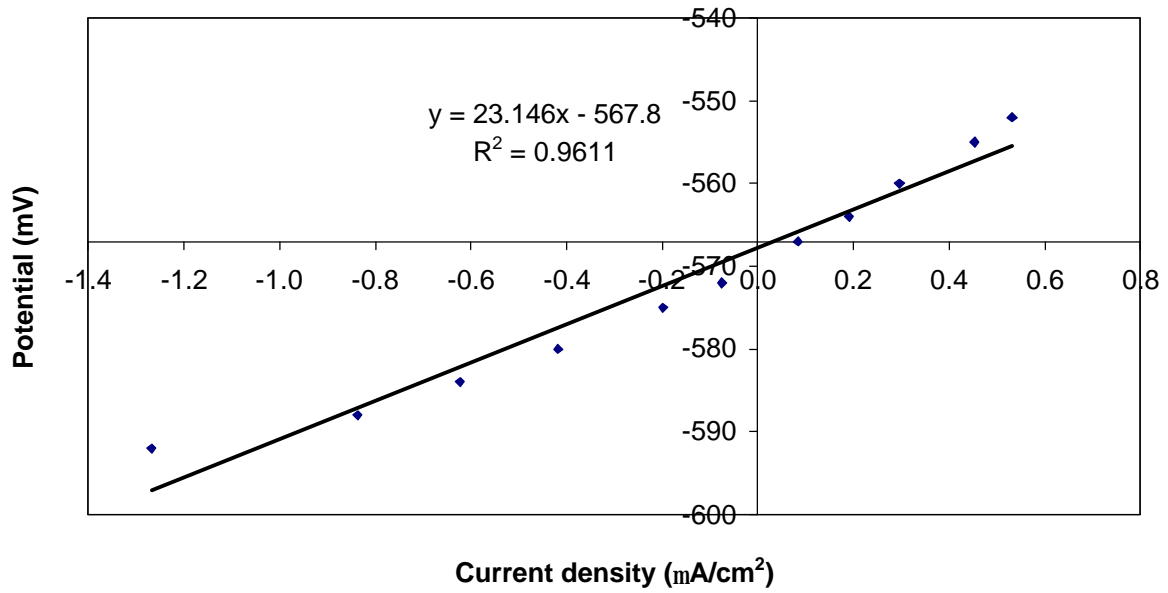
Linear Polarization Microcomposite - 2
