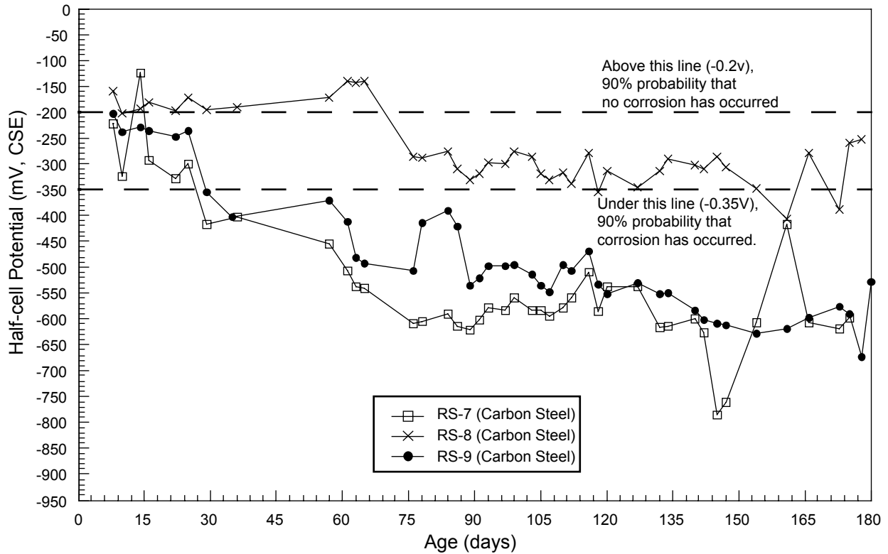
Figure 13. Half-cell potentials of carbon steel bars in Chloride ponding at 4.4°C.
