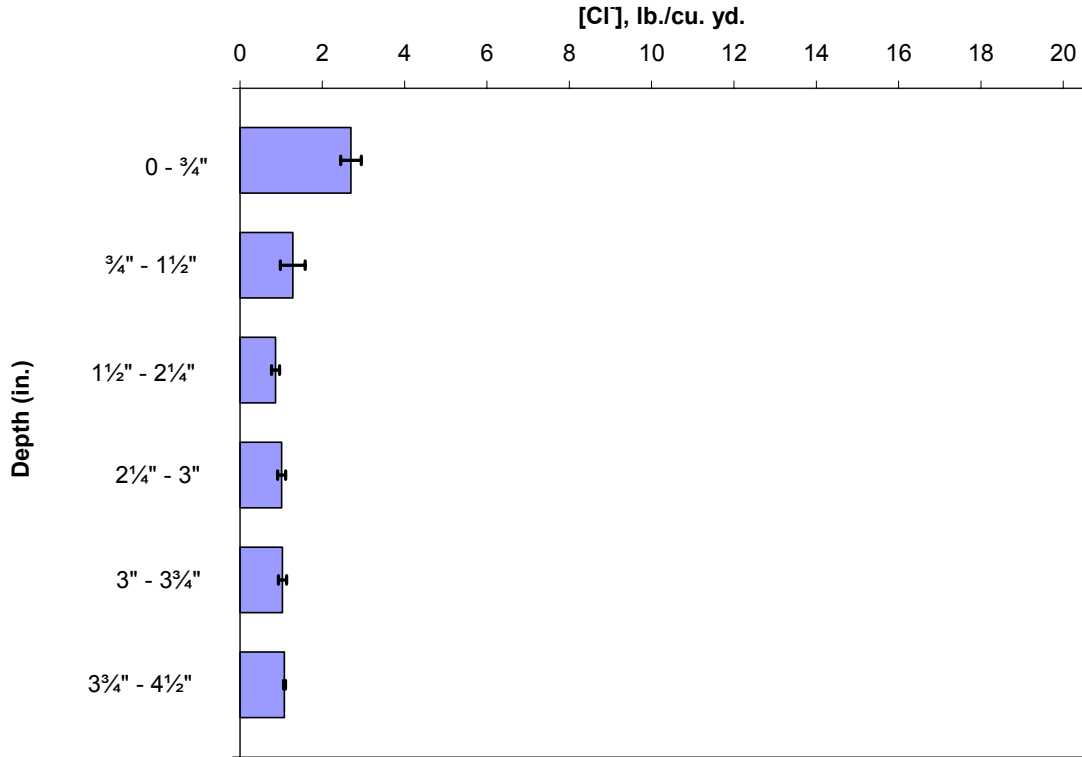
Figure 61. Chloride profile for SR 5 MP 166.00 (downtown Seattle).
