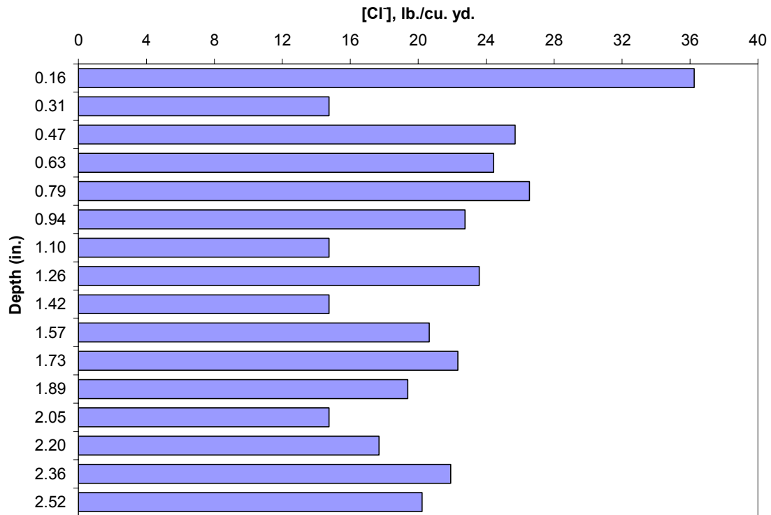
Figure 70. Chloride profile on the concrete of a non-flexible (purple) epoxy-coated specimen.
