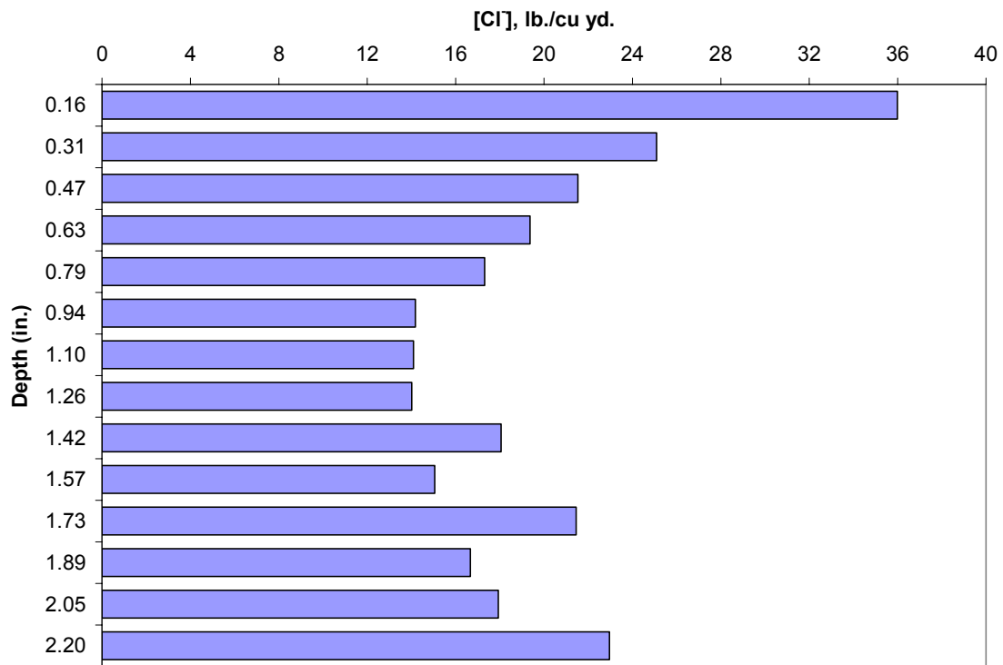
Figure 68. Chloride profile on the concrete of a stainless hollow specimen.
