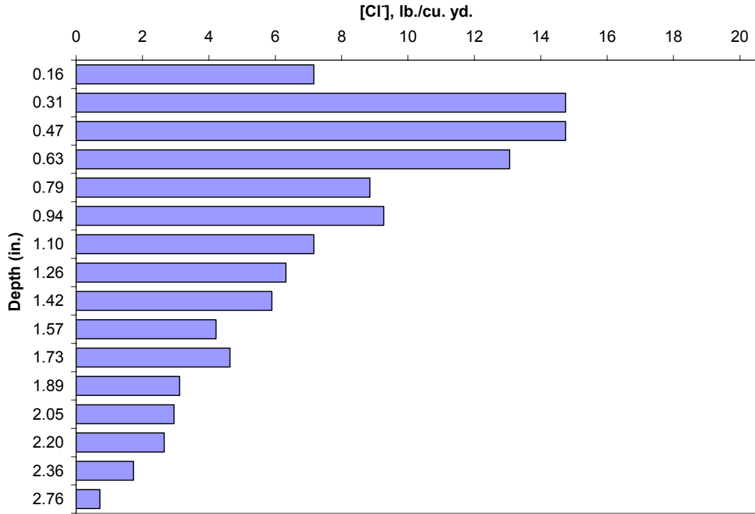
Figure 56. Chloride profile of the slab concrete (Core #1).
