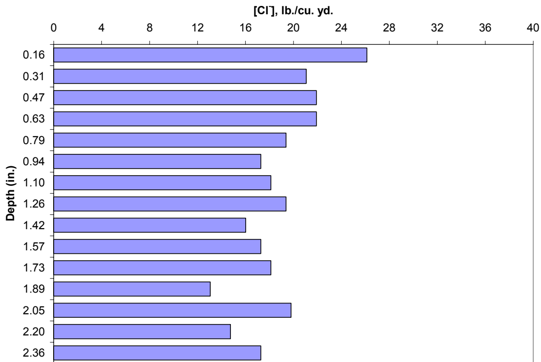
Figure 66. Chloride profile on the concrete of a carbon steel specimen.
