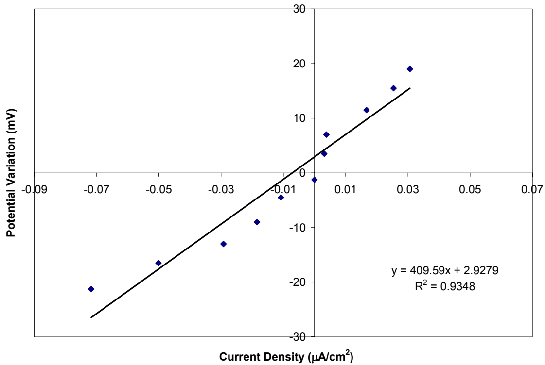
Figure 32. Linear Polarization Resistance results for flexible green epoxy-coated dowels.
