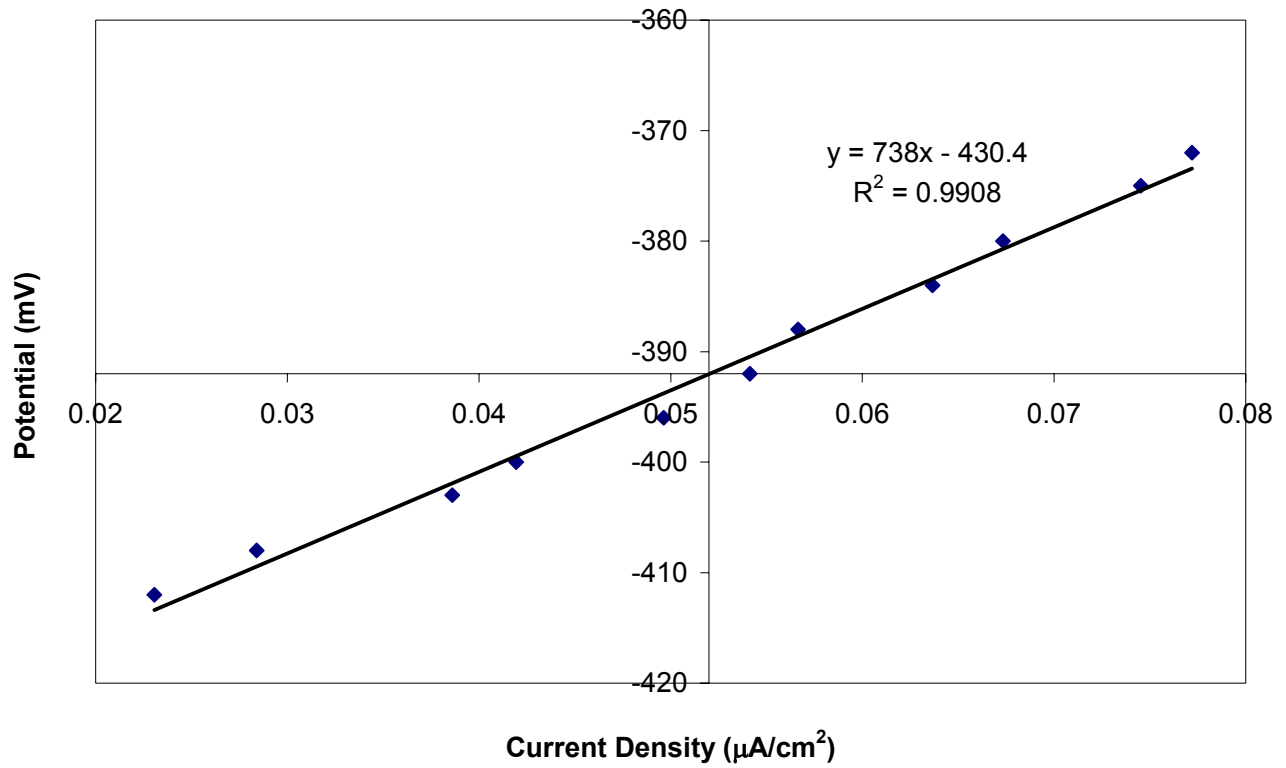
Figure 53. Linear Polarization Resistance, WSDOT slab, Specimen C.
