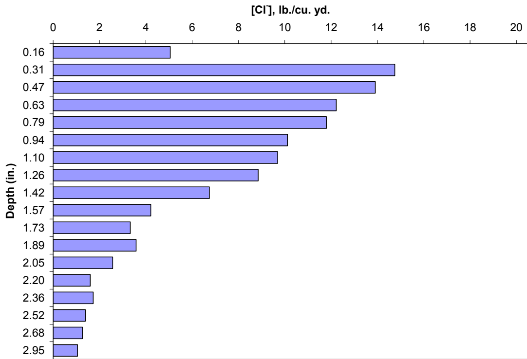
Figure 57. Chloride profile of the slab concrete (Core #2).
