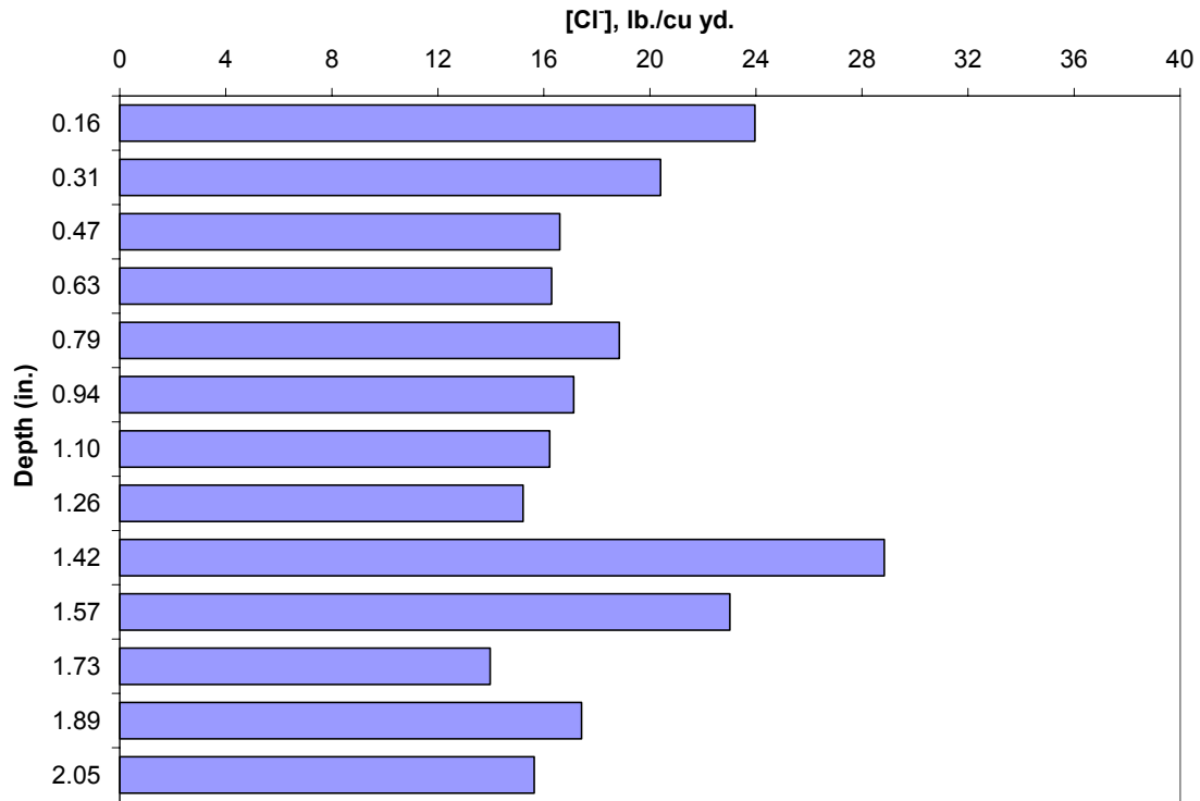
Figure 69. Chloride profile on the concrete of a flexible (green) epoxy-coated specimen.
