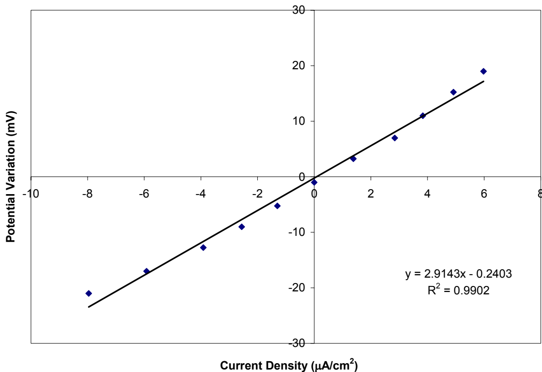
Figure 26. Linear Polarization Resistance results for carbon steel dowels.
