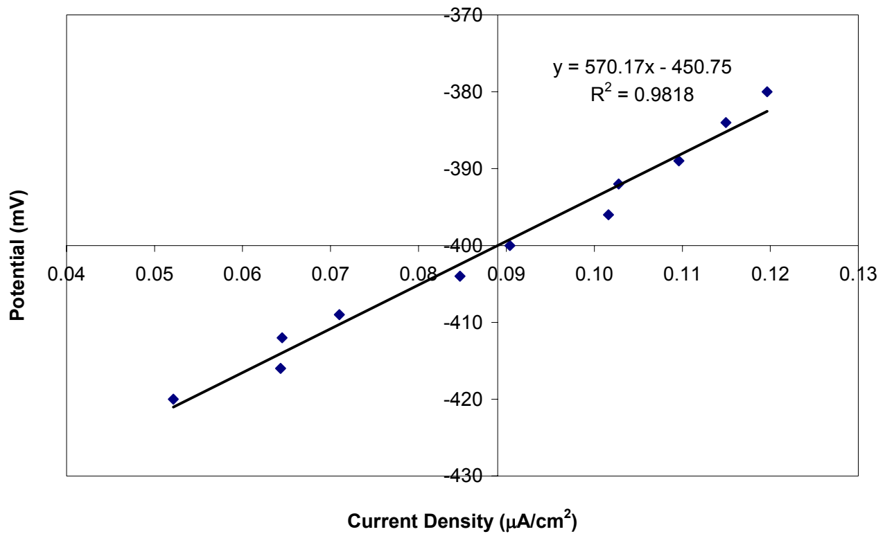
Figure 52. Linear Polarization Resistance, WSDOT slab, Specimen B.
