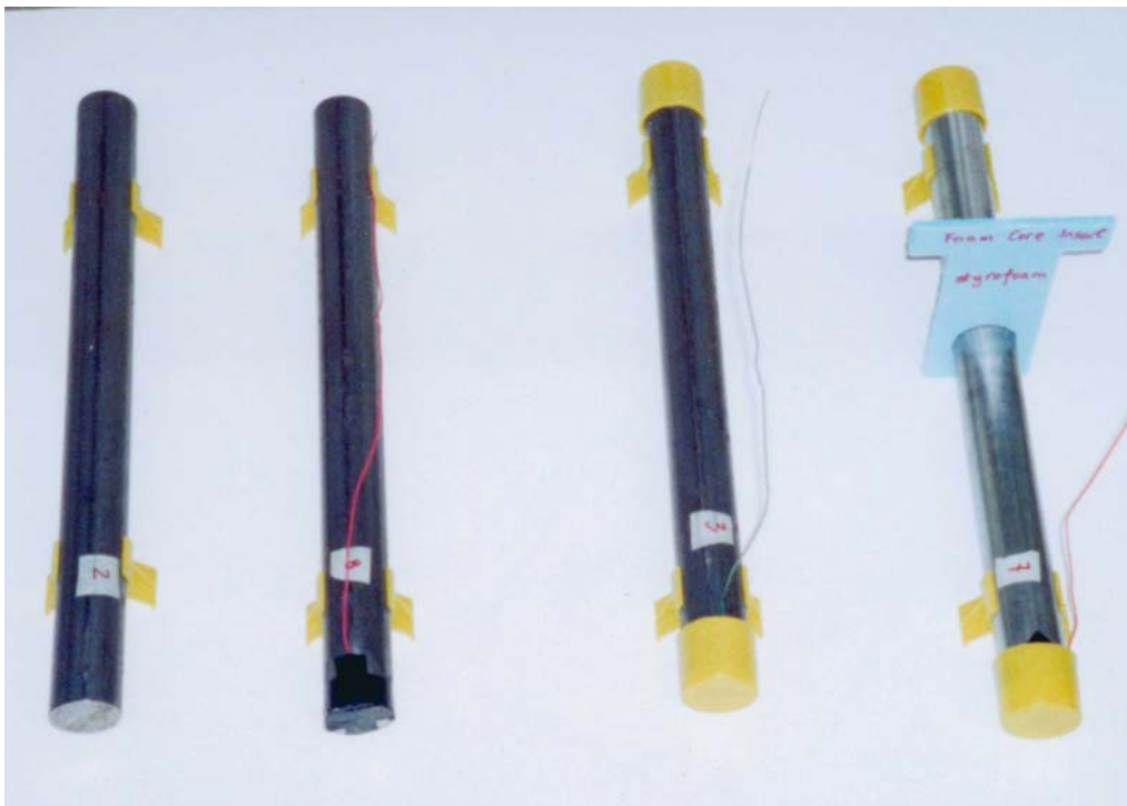
Figure 4. Preparation of dowels before casting in the concrete beams.
