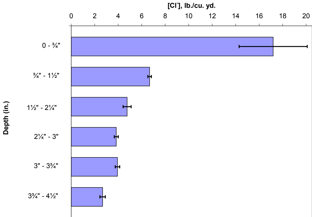
Figure 62. Chloride profile for SR 90 MP 91.324 (Elk Heights).
