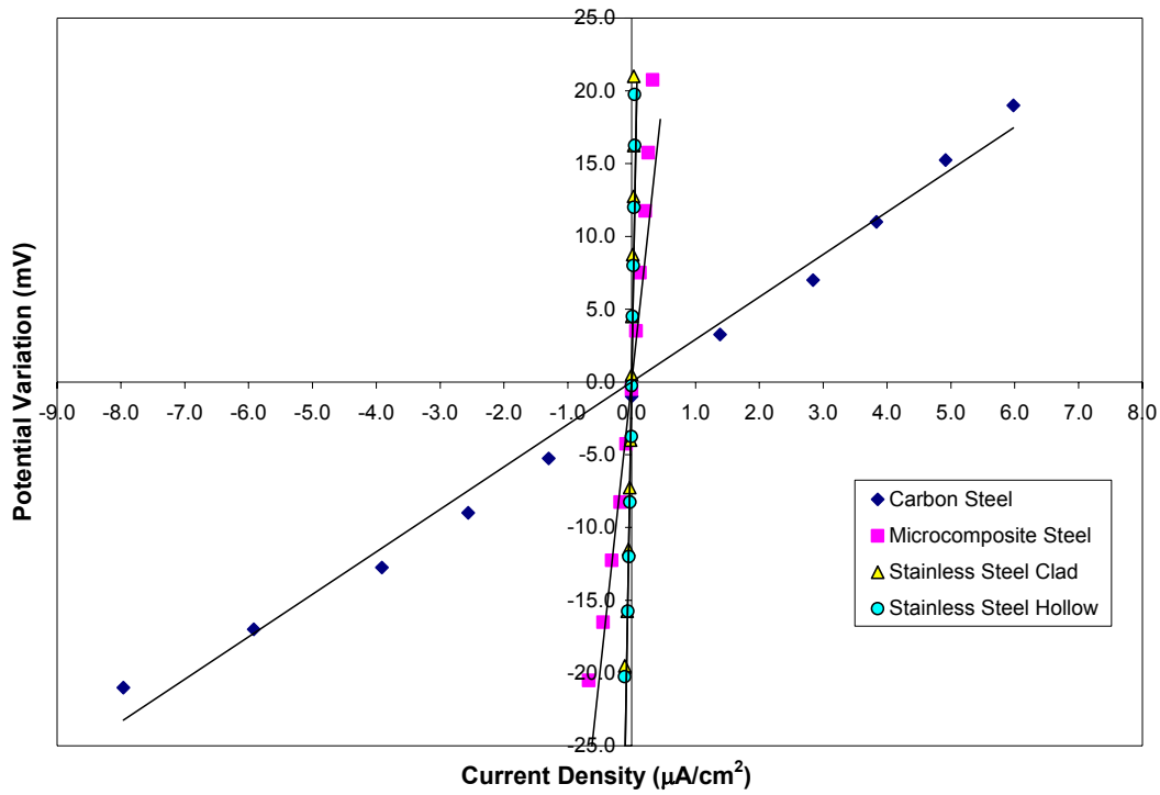
Figure 33. Summary plot showing the variation of potential and current density about the half-cell potential, for different dowels.
