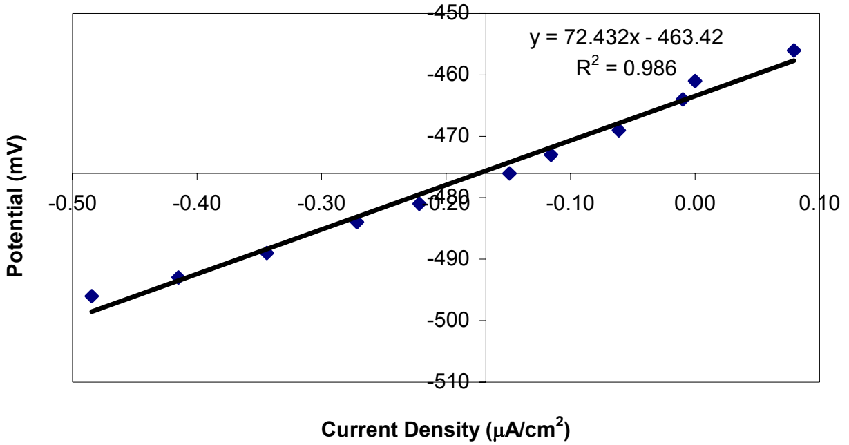
Linear Polarization Resistance Purple Epoxy (Non-flexible) - 2
