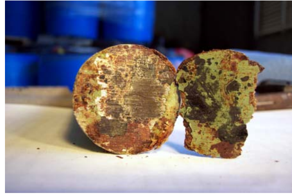
Figure 42. Epoxy-coated dowel (green). (a) General view of the center region; (b) Corroded edges and corrosion underneath coating at the end of dowels.
