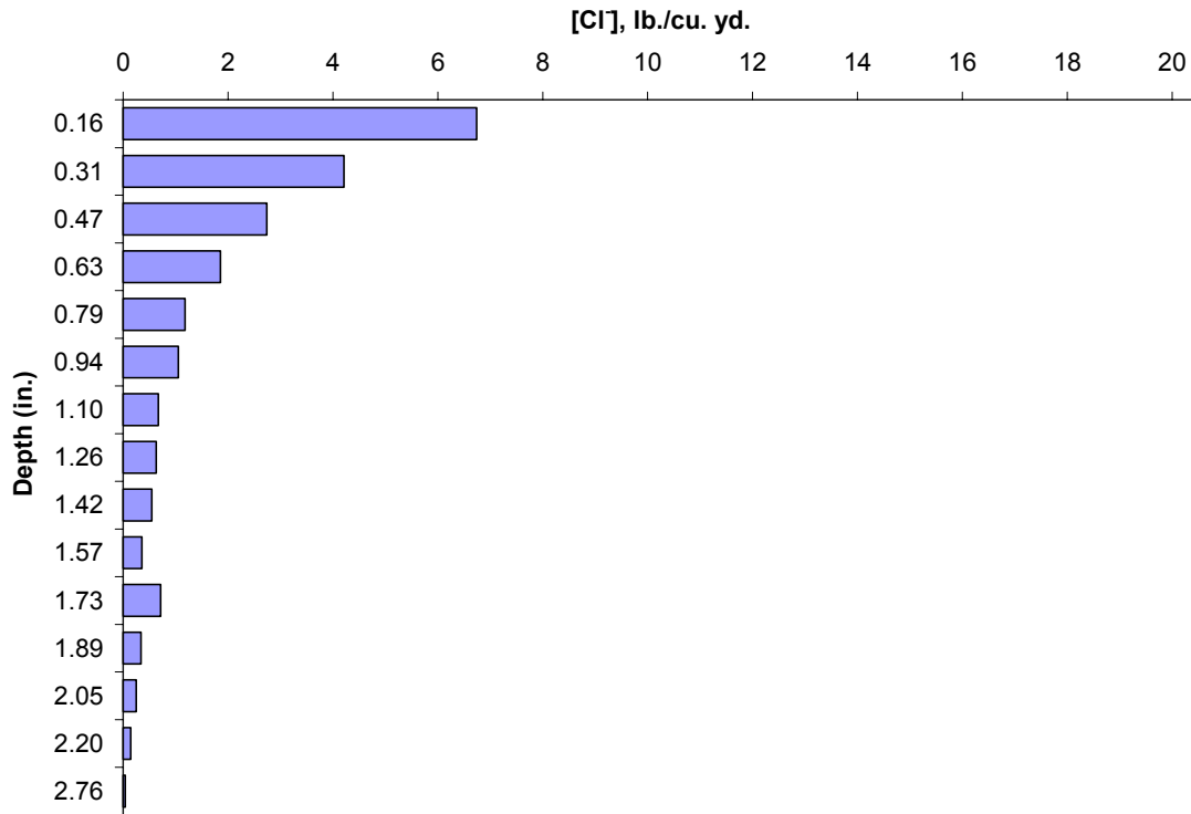
Figure 58. Chloride profile of the grout used for dowel bar retrofit (Core #3).
