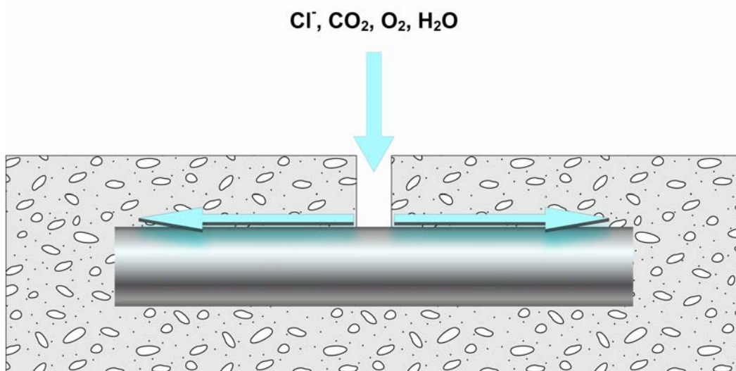
Figure 2. Aggressive agents have free access to dowels and are easily dispersed along the length of the dowel.
