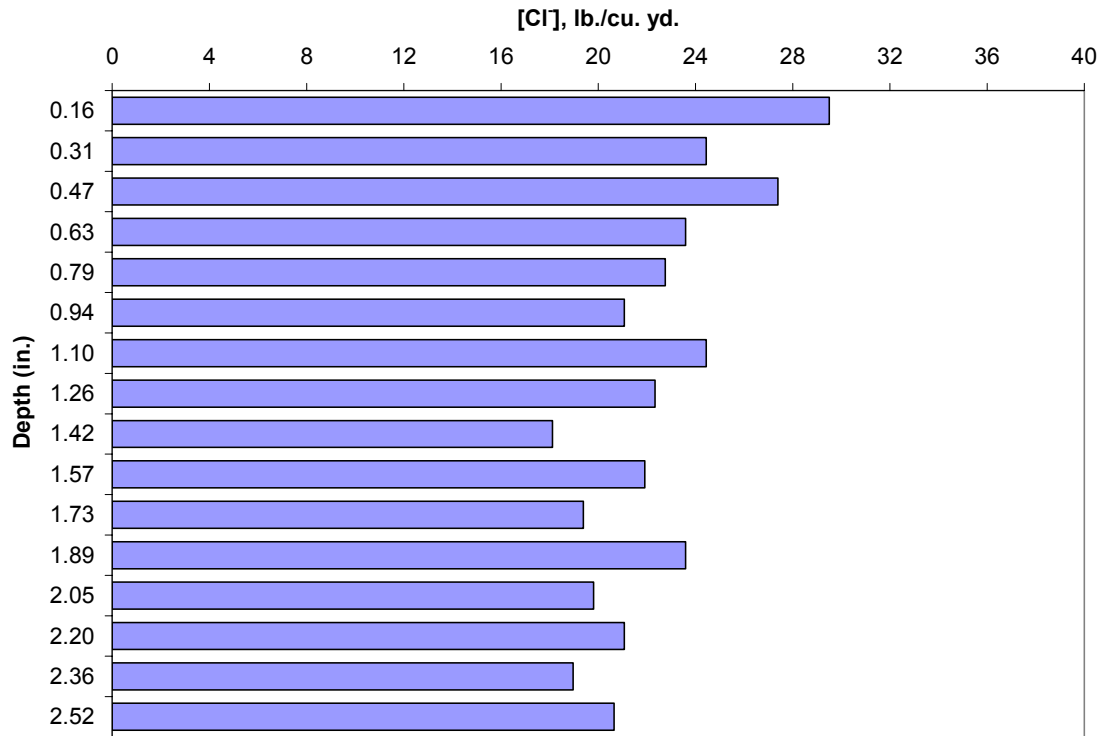
Figure 71. Chloride profile on the concrete of a microcomposite steel specimen.
