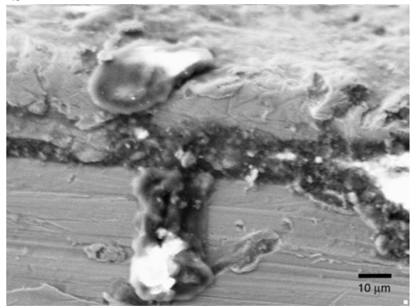
Figure 47. Stainless steel clad samples: (a) aspect of corrosion along the surface, in a region close to the end of the dowel, 100×; (b) zoom around same region, 200×; (c) details of corrosion at the surface, interface between sound and corroded area, 2390×; (d) detail of corrosion at an edge, 2320×.
