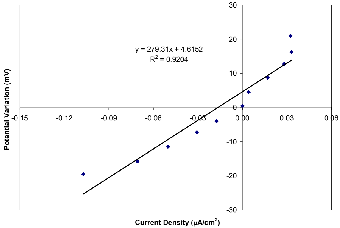
Figure 28. Linear Polarization Resistance results for stainless steel clad dowels.
