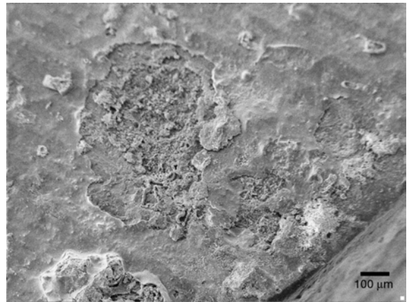
Figure 44. Carbon steel samples. (a) heavy corrosion along at the dowel surface, magnification = 100×; (b) same region, 200×; (c) different region at the surface, 200×; (d) corrosion at the bar end, 100×.
