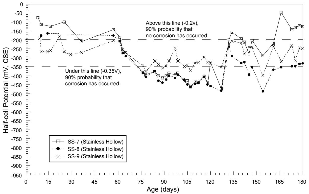
Figure 17. Half-cell potentials of stainless hollow steel bars in Chloride ponding at 4.4°C.
