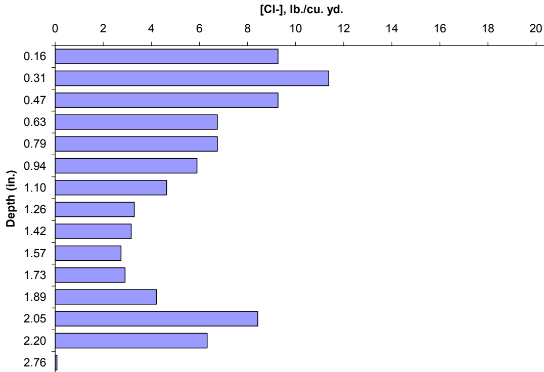
Figure 60. Chloride profile of the grout around the pavement joint (Core #6).
