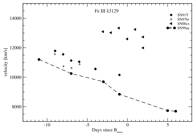
FIG. 20.—Doppler shift of the Fe III \lambda 5129 . The values for SN 1999aa are compared with those for other SNe Ia taken from Li et al. (1999, 2001a) and references therein.
