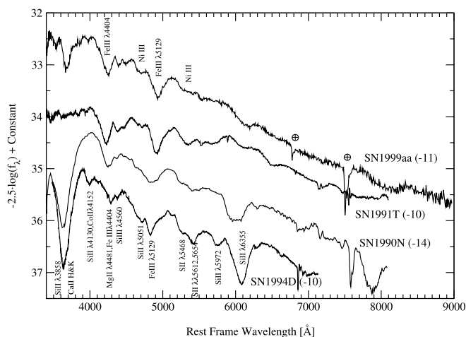
FIG. 3.—Day -11 spectrum of SN 1999aa together with those of SN 1991T and normal SN 1990N and SN 1994D from Filippenko et al. (1992), Leibundgut et al. (1991), and Patat et al. 1996. Each spectrum is labeled with the phase (days since B maximum). Line identification is explained in the text. The circled plus sign marks atmospheric absorptions.
