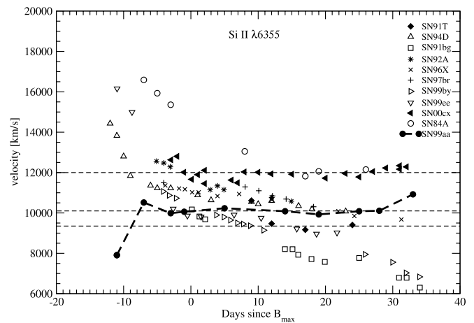
FIG. 18.—Doppler shift of the Si II \lambda 6355 . The values for SN 1999aa are compared with those for other SNe Ia taken from Li et al. (1999, 2001a), Garnavich et al. (2001), and Salvo et al. (2001) and references therein. The low value of SN 1999aa at day -11 is probably due to C II or H contamination. SN 2000cx, SN 1999aa and SN 1991T maintain a constant velocity of 12,000, 10,100, and 9400 \text{km s}^{-1} (dashed lines), respectively, from maximum light to after day 20.
