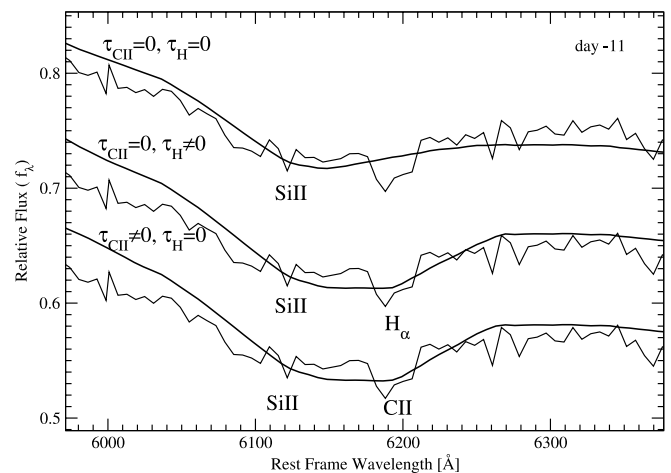
FIG. 21.—Synthetic spectra compared with SN 1999aa spectrum for day -11 around 6150 \text{ \AA} . Top model: Solid lines, \tau_{\text{H}} = 0 , \tau_{\text{CII}} = 0 and data. Middle model: Solid lines, \tau_{\text{H}} \neq 0 , \tau_{\text{CII}} = 0 and data. Bottom model: Solid lines, \tau_{\text{CII}} \neq 0 , \tau_{\text{H}} = 0 and data. The continuum level has been shifted to match the data. SYNOW parameters for C II are presented in Table 2 and those for H are presented in the text. Ions responsible for features in the synthetic spectrum are labeled.
