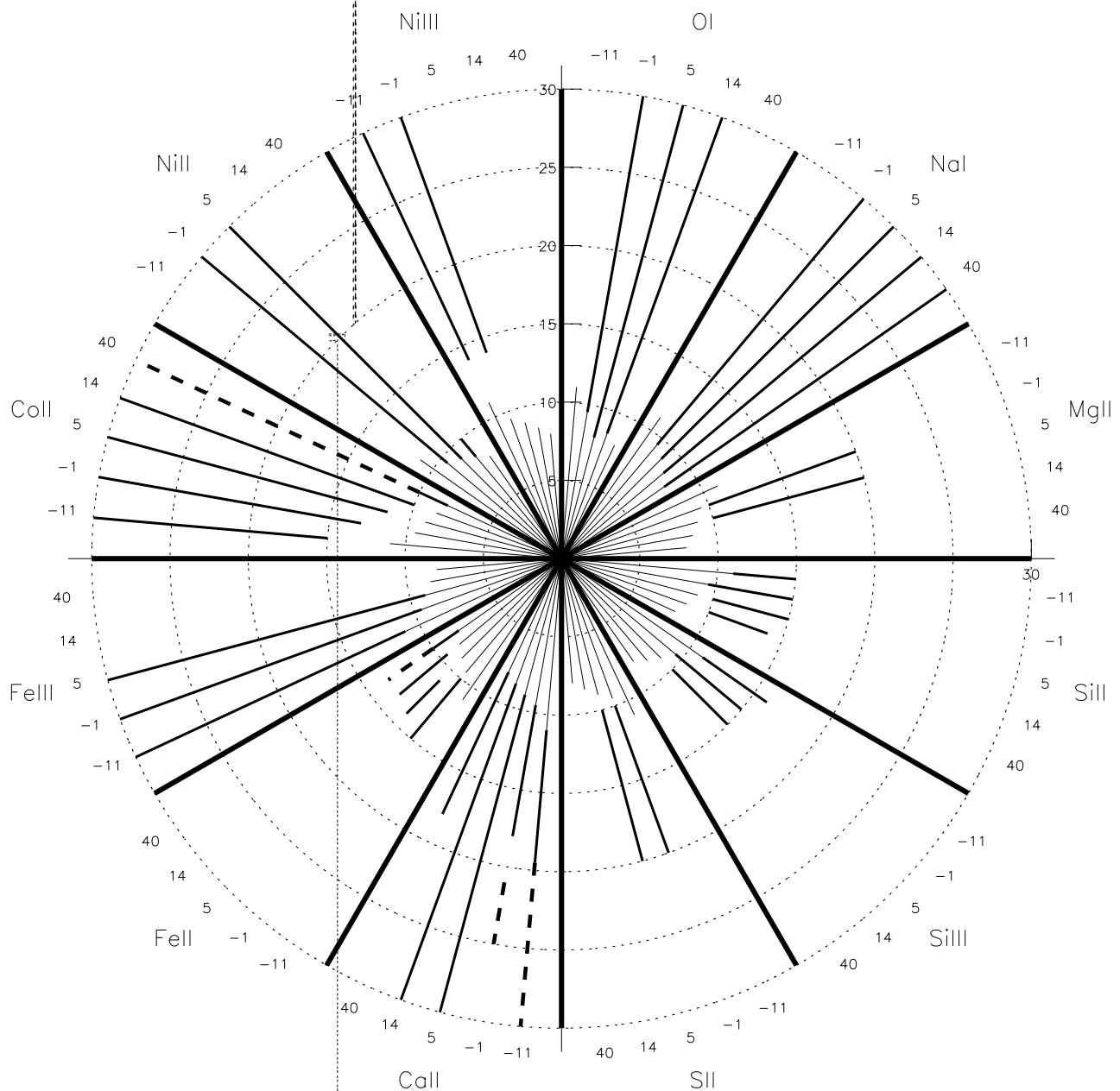
FIG. 23.—Schematic representation of the composition of SN 1999aa in velocity space as inferred from the SYNOW synthetic spectra of day -11 , -1 , +5 , +14 , and +40 . Velocities increase radially in units of 10^3 \text{ km s}^{-1} . The velocity ranges ( v_{\text{min}}-v_{\text{max}} ) for 12 ion species used in the synthetic spectra are marked with thick solid lines labeled with the ion name. High-velocity components are marked with dashed lines. In each ion section the five epochs analyzed are shown. For each epoch the extent of the photosphere is marked with a thin solid line. The contributions of C II, C III, [O II], and H are not shown. For details see § 4.
