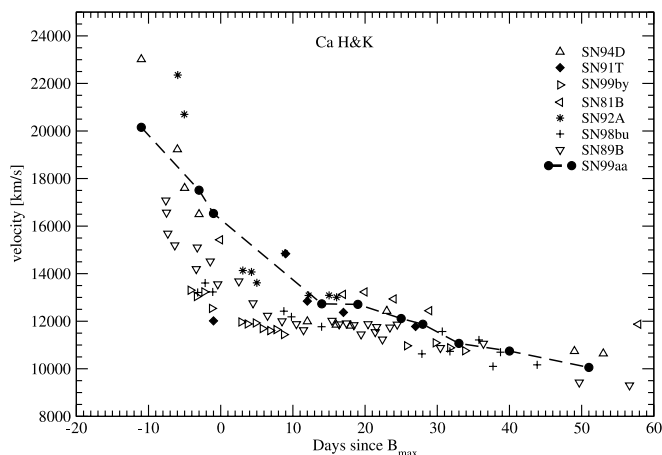
FIG. 17.—Doppler shift of the Ca H and K. The values for SN 1999aa are compared with those for other SNe Ia taken from Wang et al. (1996), Garnavich et al. (2001), Kirshner et al. (1993), Patat et al. (1996), and Jha et al. (1999) and references therein.
