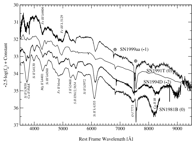
FIG. 7.—Day -1 spectrum of SN 1999aa together with those of SN 1991T, SN 1981B, and SN 1994D from Jeffery et al. (1992); Branch et al. (1983), and Patat et al. (1996). Each spectrum is labeled with the phase (days since B maximum). The circled plus sign marks atmospheric absorptions.
