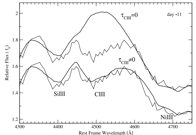
FIG. 6.—Synthetic spectra compared with SN 1999aa spectrum for day -11 around 4500 Å. Lines from top to bottom : \tau_{\text{C III}} = 0 and data, \tau_{\text{C III}} \neq 0 and data.
