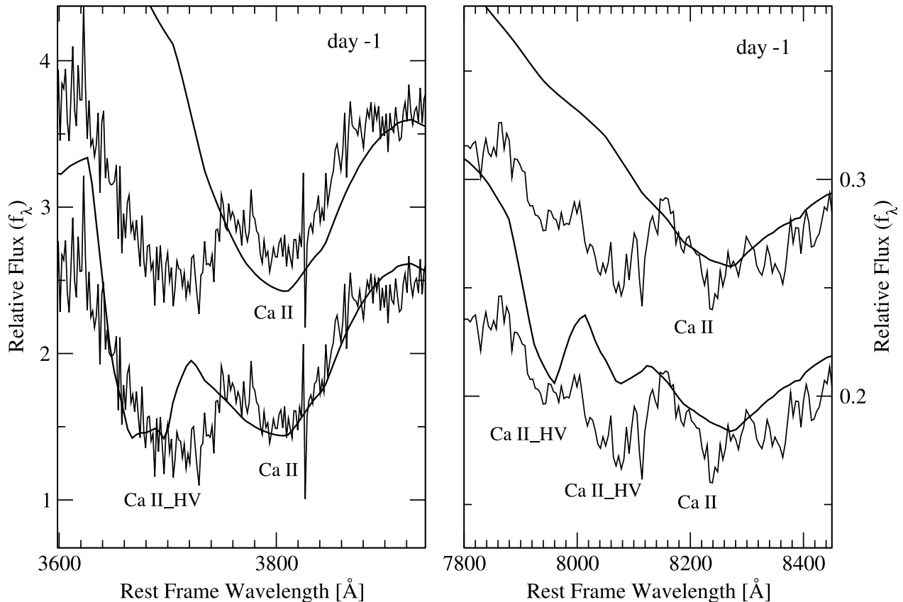
FIG. 9.—Synthetic spectrum compared with SN 1999aa spectrum for day -1 around 3800 (left) and 8000 Å (right). Top models: Solid lines, \tau_{\text{Ca II,HV}} = 0 and data; Bottom models: Solid lines, \tau_{\text{Ca II,HV}} \neq 0 and data; the continuum level in the right panel has been shifted to match the data. Ions responsible for features in the synthetic spectrum are labeled.
