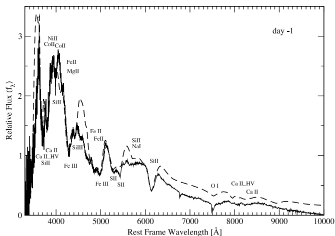
FIG. 8.—Synthetic spectrum compared with SN 1999aa spectrum for day -1 . SYNOW parameters used are presented in Table 3. The regions around 3800 and 8000 \text{ \AA} are enlarged in Fig. 9 to highlight the contribution of Ca II HV. Above 6200 \text{ \AA} the blackbody assumption fails in reproducing the correct flux values, but it does not affect the identification of the lines. Ions responsible for features in the synthetic spectrum are labeled.
