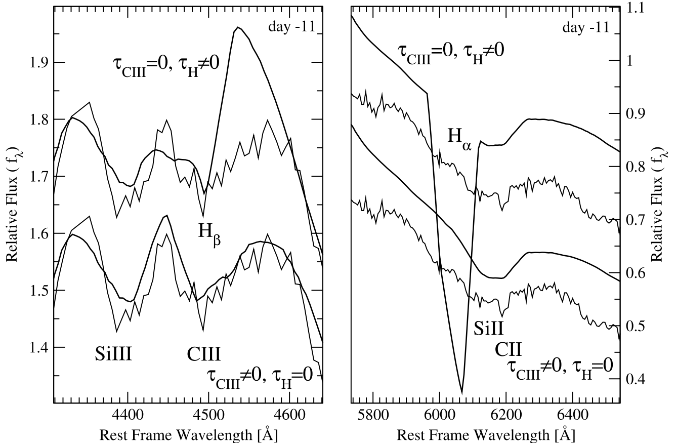
FIG. 22.—Synthetic spectra compared with SN 1999aa spectrum for day -11 around 4500 (left) and 6150 Å (right). Top model : Solid lines, \tau_{\text{H}} \neq 0 , \tau_{\text{C III}} = 0 and data. Bottom model : Solid lines, \tau_{\text{H}} = 0 , \tau_{\text{C III}} \neq 0 (as bottom model in Fig. 6) and data. In the resonance scattering approximation the optical depth necessary to reproduce the observed absorption at 4500 Å with \text{H}\beta produces a too strong \text{H}\alpha that could be weaker considering the net emission effect. SYNOW parameters for C III are presented in Table 2 and those for H are presented in the text. Ions responsible for features in the synthetic spectrum are labeled.
