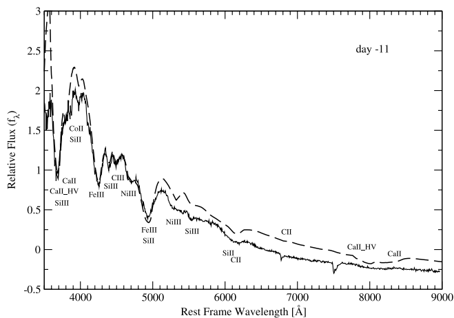
FIG. 4.—Synthetic spectrum compared with SN 1999aa spectrum for day -11 . SYNOW parameters are presented in Table 2. The regions around 6150 and 4500 \text{ \AA} are enlarged in Figs. 5 and 6 to highlight the possible contributions of C II and C III. The mismatch of the continuum level above 5000 \text{ \AA} has to be considered a limitation of the underlying blackbody assumption, but it does not affect the line identification. Ions responsible for features in the synthetic spectrum are labeled.
