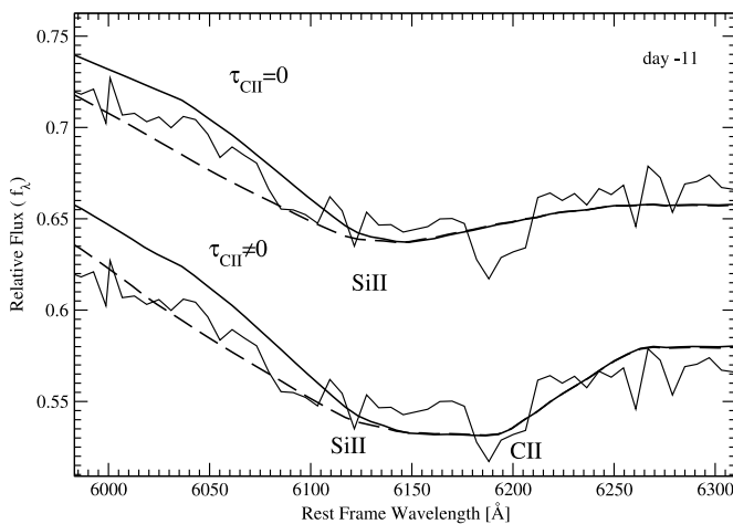
FIG. 5.—Synthetic spectra compared with SN 1999aa spectrum for day -11 around 6150 Å. Top model : Solid lines, \tau_{\text{C II}} = 0 and data; dashed lines, \tau_{\text{C II}} = 0 and Si II with v_{\max} = 30 \times 10^3 \text{ km s}^{-1} . Bottom model : Solid lines, \tau_{\text{C II}} \neq 0 and data; dashed lines, \tau_{\text{C II}} \neq 0 and Si II with v_{\max} = 30 \times 10^3 \text{ km s}^{-1} . The continuum level has been shifted to match the data. Ions responsible for features in the synthetic spectrum are labeled. The position of the minimum changes by about 50 Å when the C II component is included. The small notch around 6200 Å is an artifact of the spectrum extraction and does not have to be considered a supernova feature.
