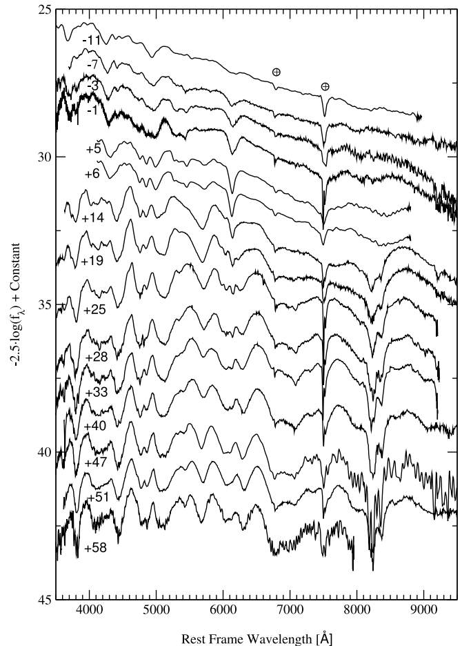
FIG. 2.—SN 1999aa spectral time sequence. The spectra are labeled in days relative to B -band maximum light. The circled plus sign marks telluric atmospheric absorptions.
