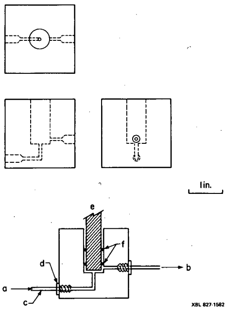
Fig. 4.11. "Electrode blocks" in continuous flow system; machined from Lucite and polished. a. mixed SCW and SAOB enter. b. solution exits block. c. 1mm I.D. thin-walled Teflon tube. d. drilled plastic screw. e. electrode. f. O-rings. Blocks for reference and silver sulfide electrodes are as shown. Cavity of pH electrode block has conical bottom to accommodate electrode bulb.
