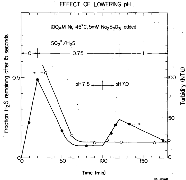
Fig. 3.3. Development of reactivity and turbidity; effect of lowering pH.
