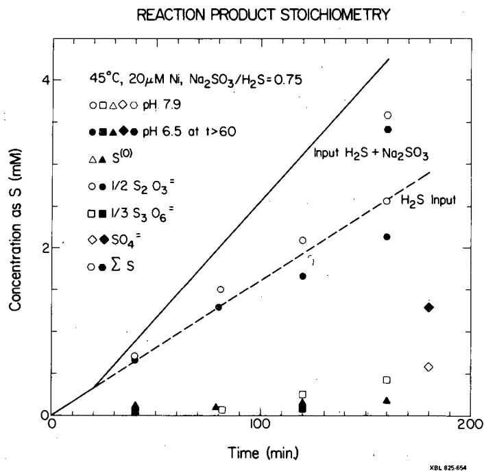
Fig. 3.11. Distribution of reaction products; 20 μM nickel, sulfite:sulfide = 0.75. Open symbols: pH = 7.9. Solid symbols: pH = 6.5.
