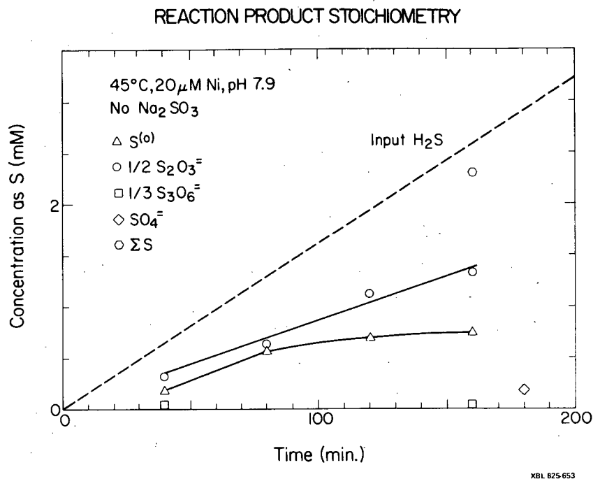
Fig. 3.10. Distribution of reaction products; 20 μM nickel, no sulfite, pH = 7.9.
