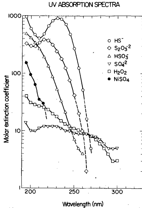
Fig. 3.17. UV absorption spectra of sulfur compounds.
