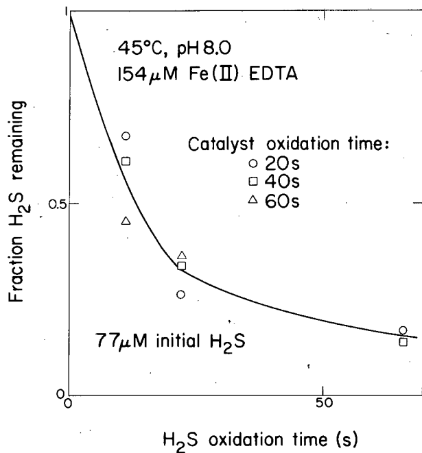
Fig. 4.4. Reaction catalyzed by iron complexes; effect of catalyst oxidation time.
