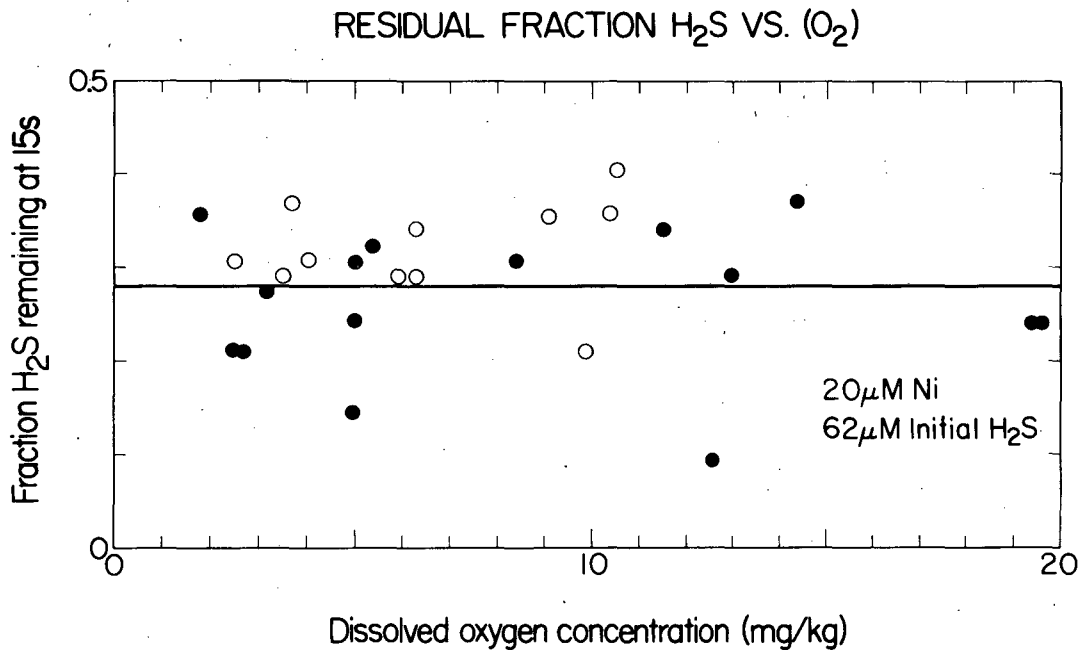
Fig. 3.9. Reactivity vs. oxygen concentration.
