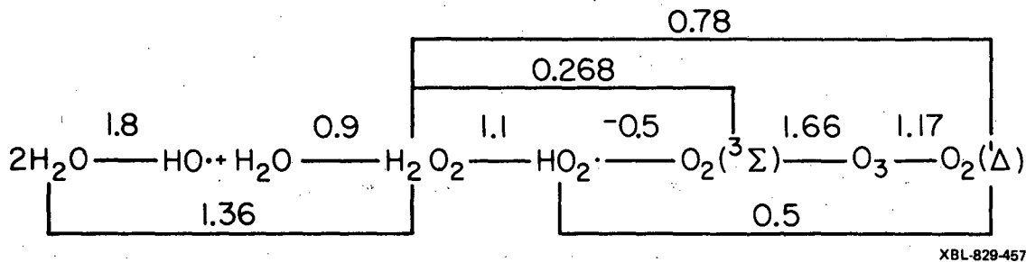
Fig. 2.3. Reduction potentials in the oxygen system at pH 7 and 25°C. Calculated from values tabulated by Latimer (1952).
