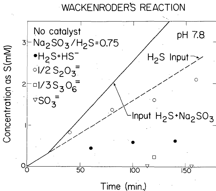
Fig. 4.2. Wackenroder's reaction; no catalyst added.
