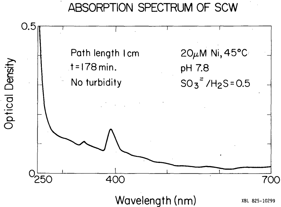
Fig. 3.18. Absorption spectrum of SCW.
