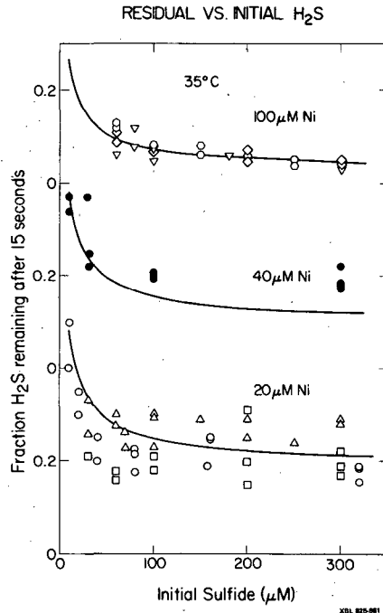
Fig. 3.4. Fraction sulfide remaining after 15 seconds; 35°C and various concentrations of nickel. Vertical scale displaced between curves. In Figures 3.4 to 3.9 different symbols represent data from different experiments. "Initial sulfide" is the amount added in reactivity determinations.
