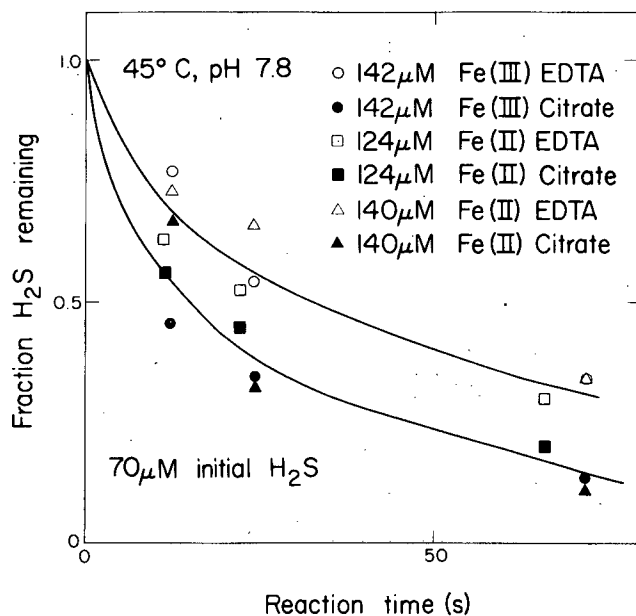
Fig. 4.3. Reaction catalyzed by iron complexes; comparison of catalysts, effect of catalyst's oxidation state. Data generated with continuous flow system.
