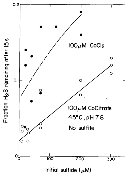
Fig. 4.7. Reaction catalyzed by cobalt. Solid symbols: 100 \mu\text{M} cobalt chloride. Open symbols: 100 \mu\text{M} cobalt citrate. 70 \mu\text{M} sulfide added in reactivity determinations.
