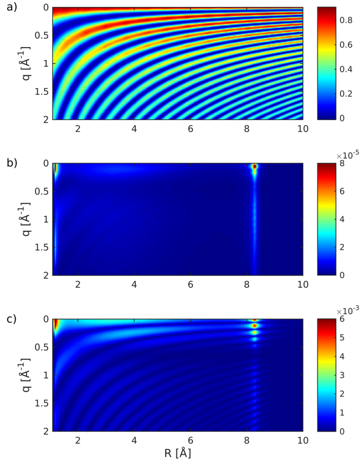
FIG. 5. Relevant density operator matrix elements in the nuclear subspace of NaF [obtained using Eq. (8)]: (a) \hat{\sigma}_{ee}^2(\mathbf{q}, R) , (b) \hat{\sigma}_{ge}^2(\mathbf{q}, R) , and (c) |\hat{\sigma}_{ee}^\dagger(\mathbf{q}, R)\hat{\sigma}_{ge}(\mathbf{q}, R)| . \hat{\sigma}_{gg}^2 is not shown due to its visual similarity to \hat{\sigma}_{ee}^2 .
