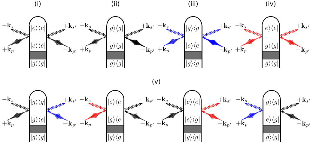
FIG. 2. Loop diagrams for single-molecule X-ray scattering processes as given by Eq. (5) and Fig. 4. The shaded area represents an arbitrary excitation that prepares the system in a superposition state of |g\rangle and |e\rangle . Diagrams for elastic scattering from e and g are shown in (i) and (ii) respectively, while the diagrams for inelastic scattering from e and g are displayed in (iii) and (iv). The bottom row (v) represents all diagrams involving electronic coherences. We denote modes of the X-ray probe pulse with p and p' , whereas s, s' represent relevant scattering modes ( \mathbf{k}_{p(i)} has frequency \omega_{p(i)} and \mathbf{k}_{s(i)} has frequency \omega_{s(i)} ). Elastic scattering processes come with \hat{\sigma}_{gg} or \hat{\sigma}_{ee} and are denoted by black field arrows. Inelastic processes in which the molecule gains (Stokes) or loses (anti-Stokes) energy to the field come with \hat{\sigma}_{ge} or \hat{\sigma}_{eg} depending whether the action is on the ket or bra and are denoted with red and blue field arrows to indicate the field's spectral shift due to the particular diagram. Note that we use |i\rangle instead of |\phi_i\rangle for the electronic states in this figure to aid readability.
