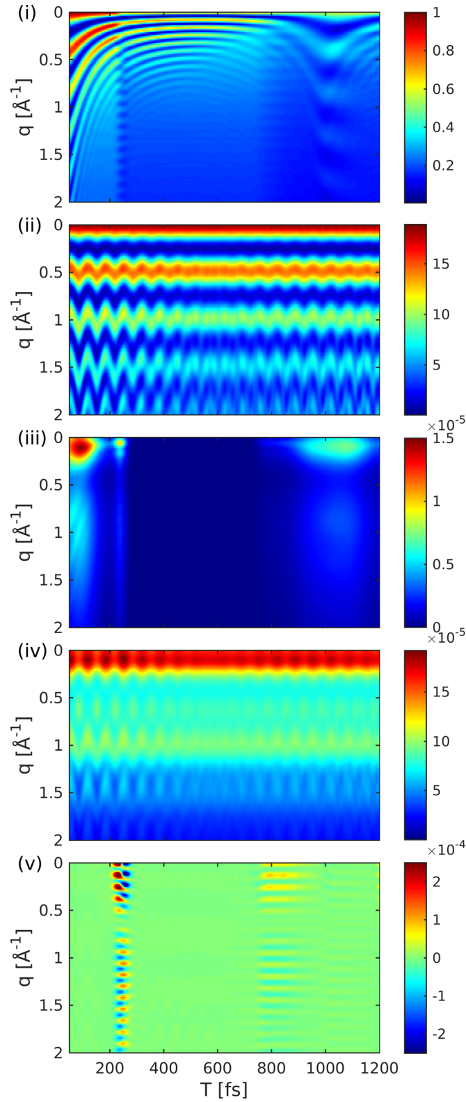
FIG. 8. Variation with a probe delay T of the five basic contributions to the gas-phase diffraction signal of NaF vs. the momentum transfer q . Panel labeling corresponds to Eq. (6). Signal intensities are normalized relative to (i). (i) and (ii) Elastic contributions from e and g , respectively. (iii) and (iv) Weaker inelastic contributions from e and g , respectively. (v) Combined contribution of inelastic scattering and electronic coherences whose intensity lies between the elastic and inelastic terms.
