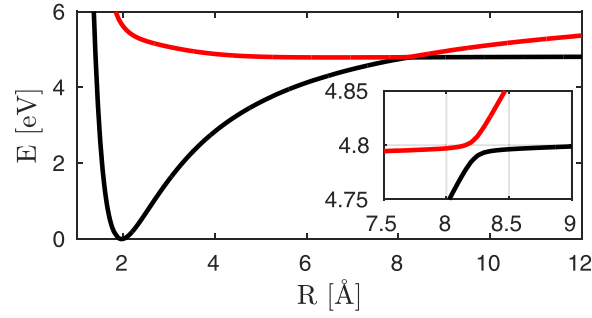
FIG. 3. Adiabatic potential energy surfaces for the electron harpooning in NaF (ionic state X^1\Sigma |g\rangle black, covalent state A^1\Sigma, |e\rangle red). The inset displays a close up of the avoided crossing region.
