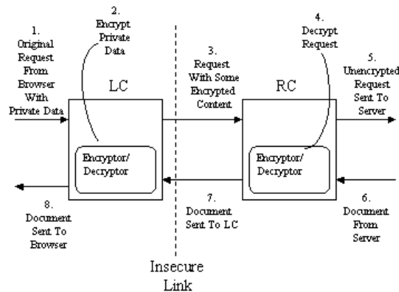
Fig. 10. The Selective Encryptor
