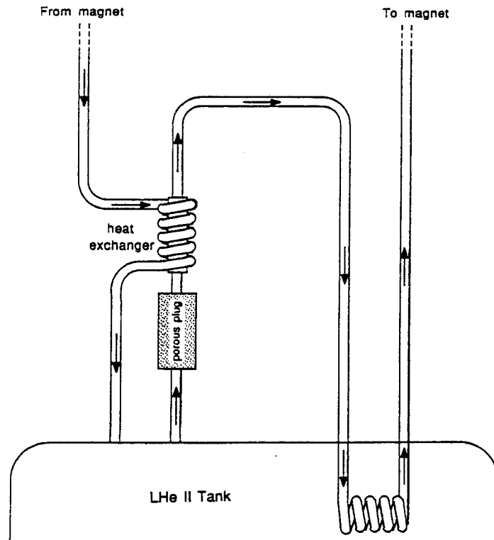
Figure 3 Thermomechanical Pump for Astromag
