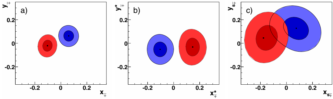
FIG. 1 (color online). Contours at 39.3% (dark) and 86.5% (light) two-dimensional C.L. in the (a) Z_{\mp} , (b) Z_{\mp}^* , and (c) Z_{s\mp} planes, corresponding to one- and two-standard deviation regions (statistical only), for B^- (solid lines) and B^+ (dotted lines) decays.
