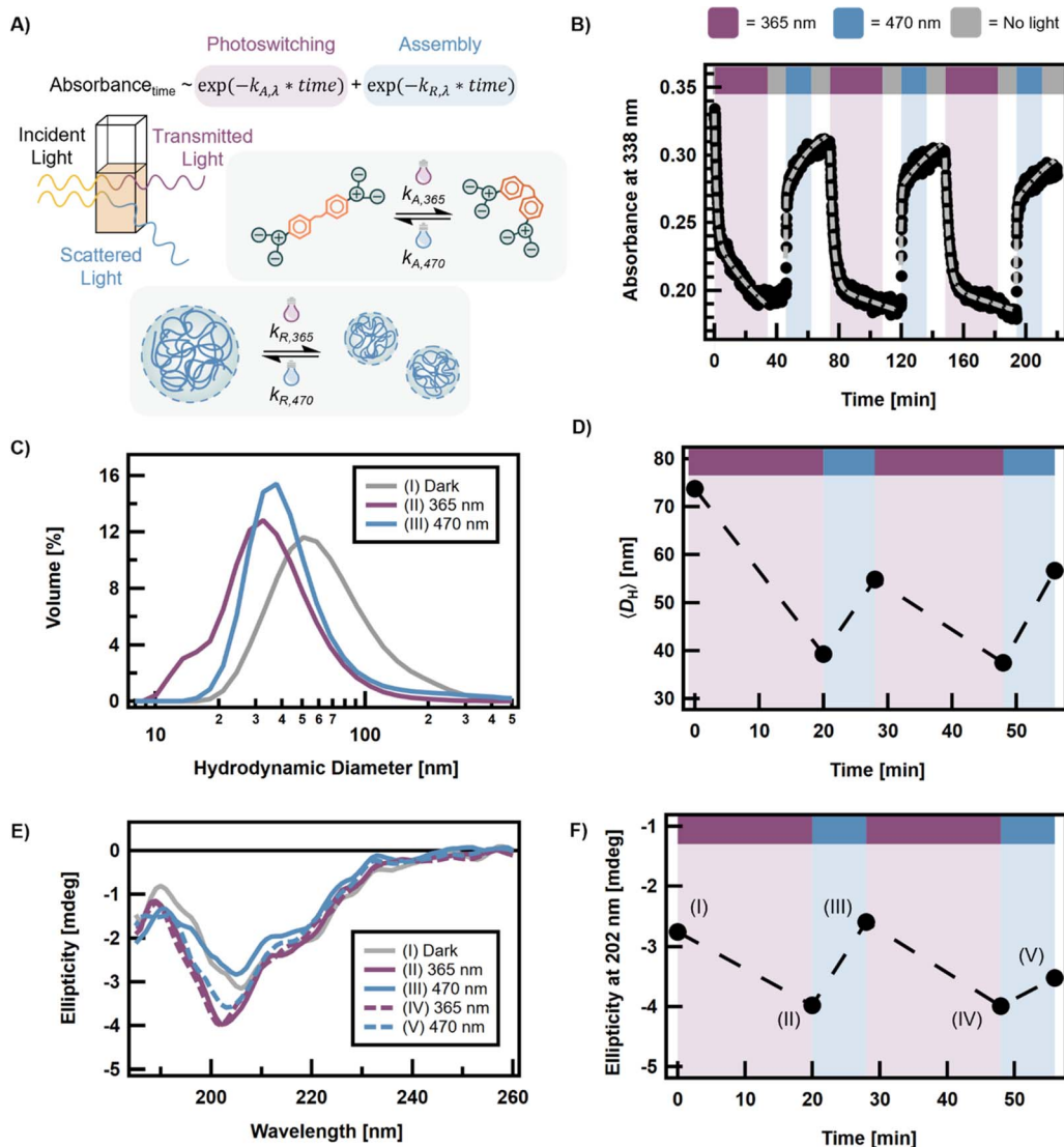
Fig. 5 Photoresponse of the azoEDTA–reflectin system for 8 \mu M reflectin and 240 \mu M azoEDTA. (A) Schematic illustrating how photoisomerization and turbidity contribute to changes in the measured absorbance of the system upon irradiation. (B) Time-dependent absorbance was collected for 3 cycles with UV light irradiation for 34 min, blue light for 17 min, and no light for 12 min following each irradiation (black dots). The behavior can be fit to a biexponential model (gray lines) that accounts for the photoisomerization and assembly processes. Rate coefficients are given in Table S2.† (C) DLS shows a change in assembly size distribution after irradiation with UV and blue light. (D) The change in \langle D_H \rangle , as measured by DLS, can be cycled twice. (E) Evolution of ellipticity of dark-equilibrated azoEDTA–reflectin complexes (I) when exposed to 365 nm (II, IV) and 470 nm (III, V) irradiation. (F) Ellipticity at 202 nm can be cycled as a function of light irradiation.
